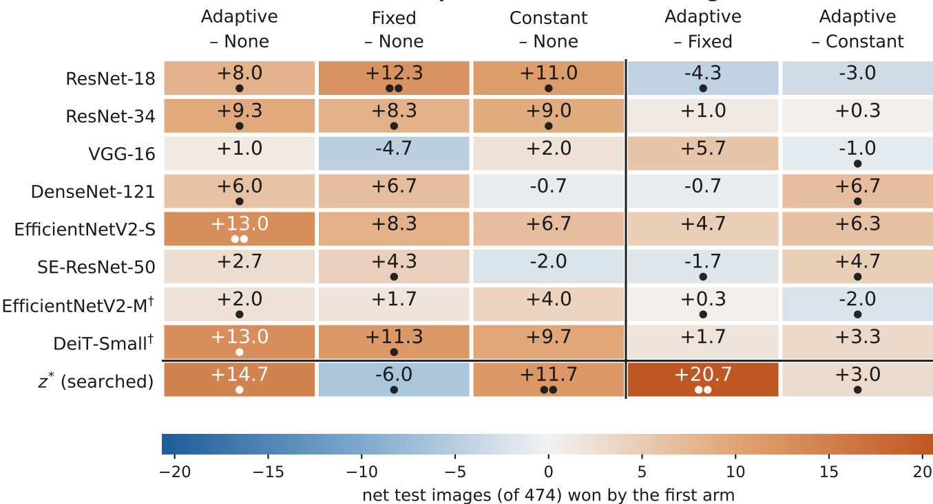
a Paired McNemar comparisons, mean net images over 3 seeds
