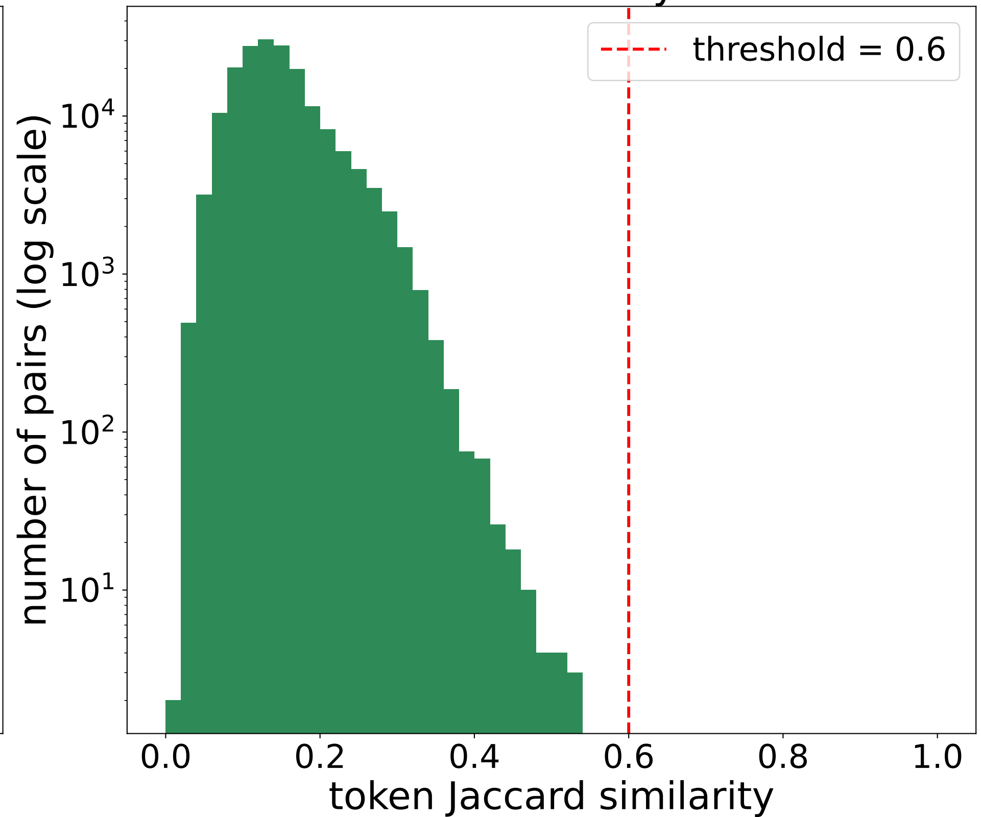
Pairwise token similarity distribution
