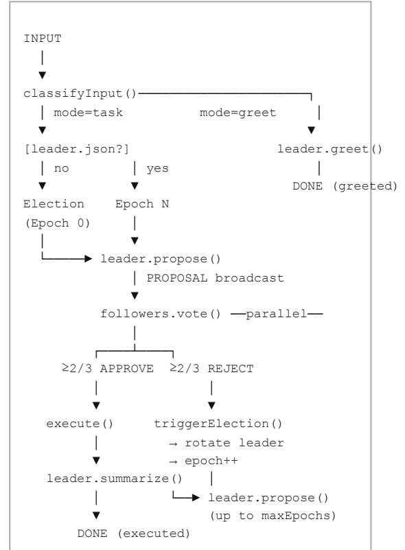
Figure 1. AgentRaft protocol state machine. Deposition loops back to the proposal phase with a new leader.
