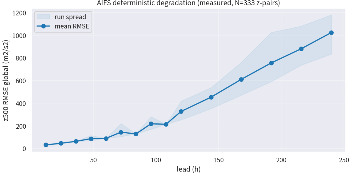
Figure 1: AIFS deterministic z_{500} global RMSE by lead (measured, N=333 pairs as of 2026-10-07, leads to 240 h; mean line, min–max spread band). Degradation is monotone at well-sampled leads; the long-lead spread is regime-structured (120 h bimodal by regime week, see Table 2 caption) and is itself first-class data.
