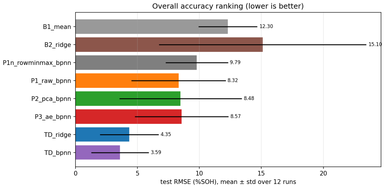
Figure R2. Overall test RMSE (%SOH, mean ± std over 12 runs). Time-domain features halve the best EIS error.
