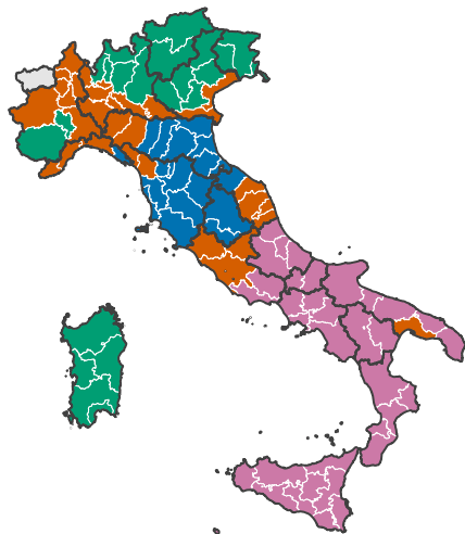
Preferred GW power
