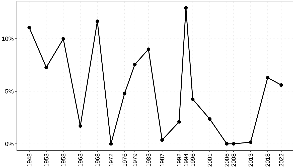
Zero-cell share
