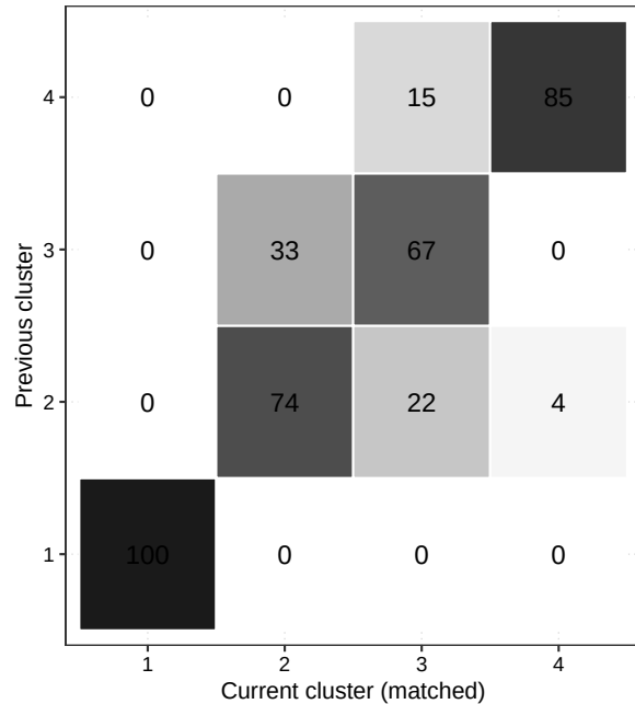
2008 -&gt; 2013 (ARI = 0.679)
