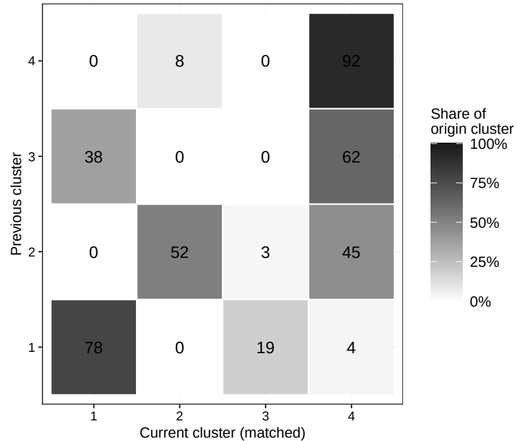
2013 -&gt; 2018 (ARI = 0.281)
