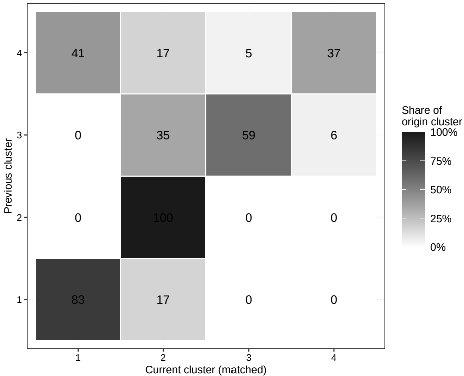
1994 -> 1996 (ARI = 0.299)
