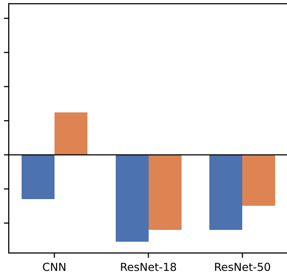
QAT
