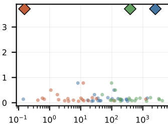
ResNet-18
