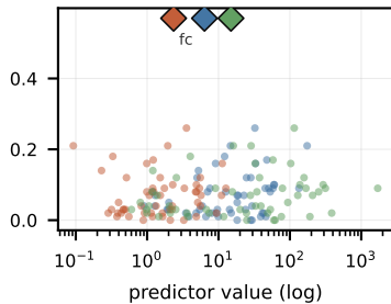
ResNet-50
