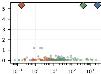
ResNet-50
