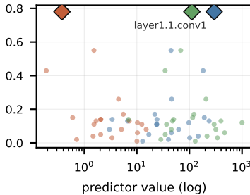
ResNet-18
