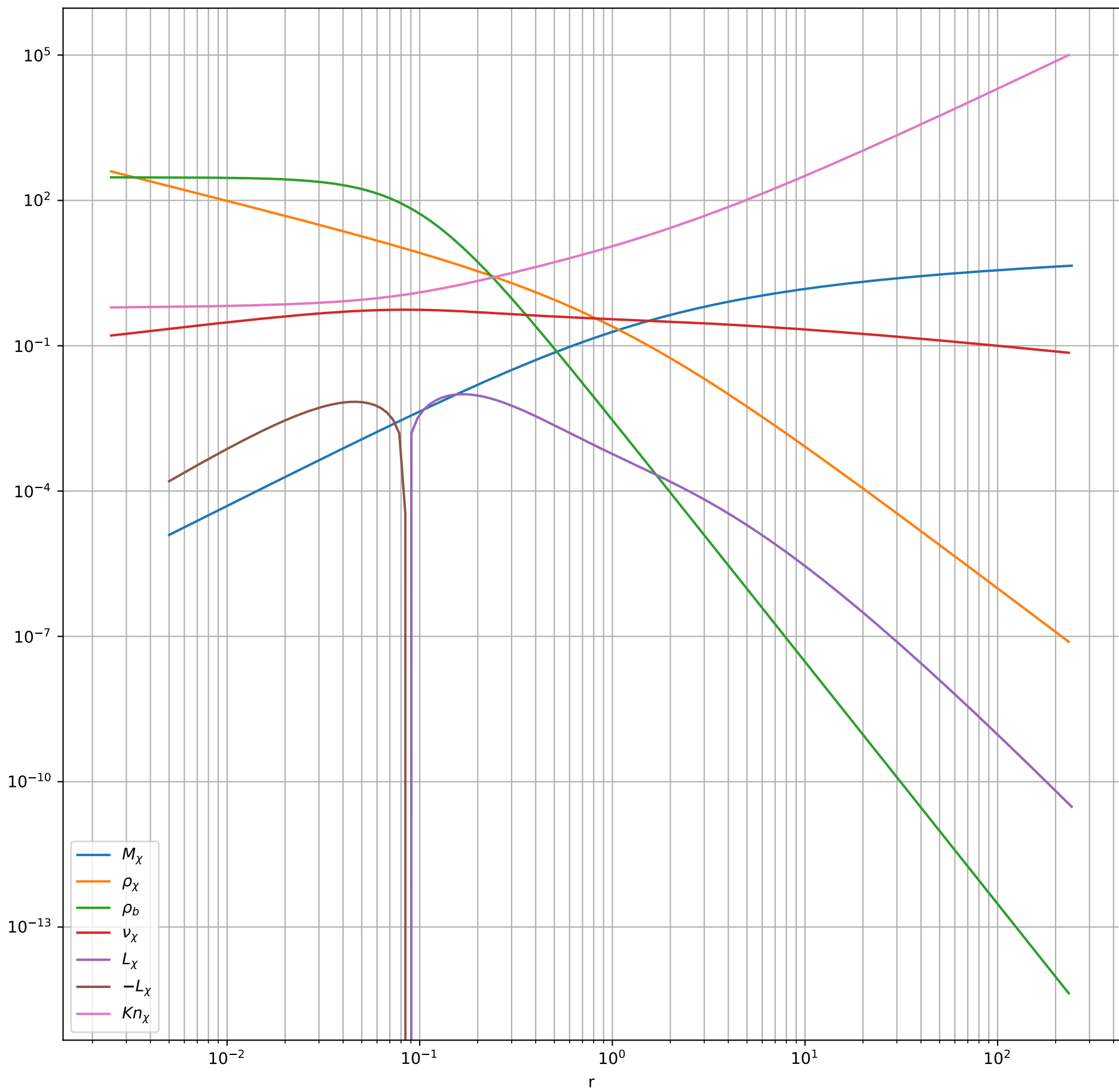
Red Dot Halo Initial Condition
