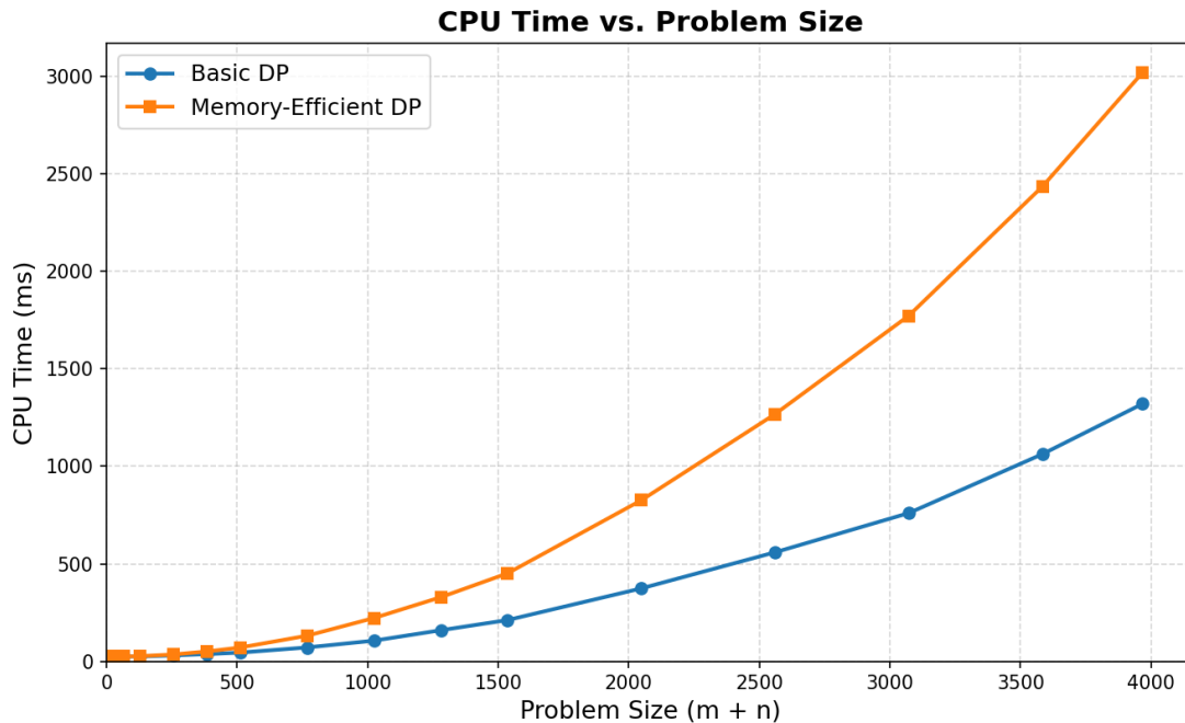
Graph 2 — CPU Time vs. Problem Size (M+N)
