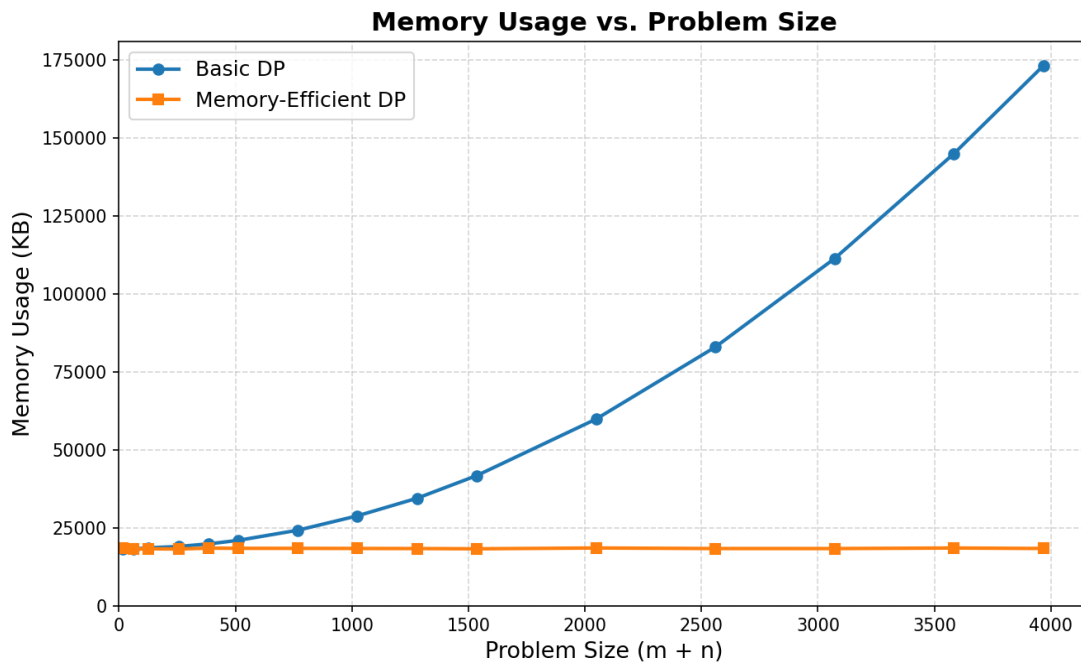
Graph 1 — Memory Usage vs. Problem Size (M+N)
