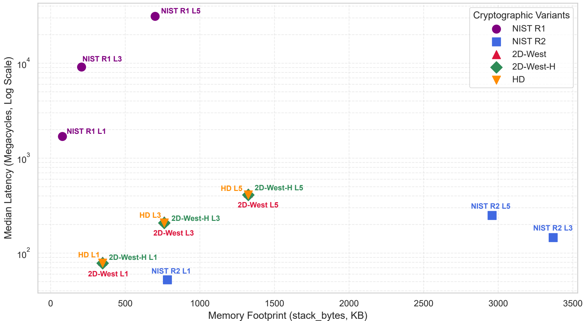
Keygen Latency vs. Memory Footprint (stack_bytes)
