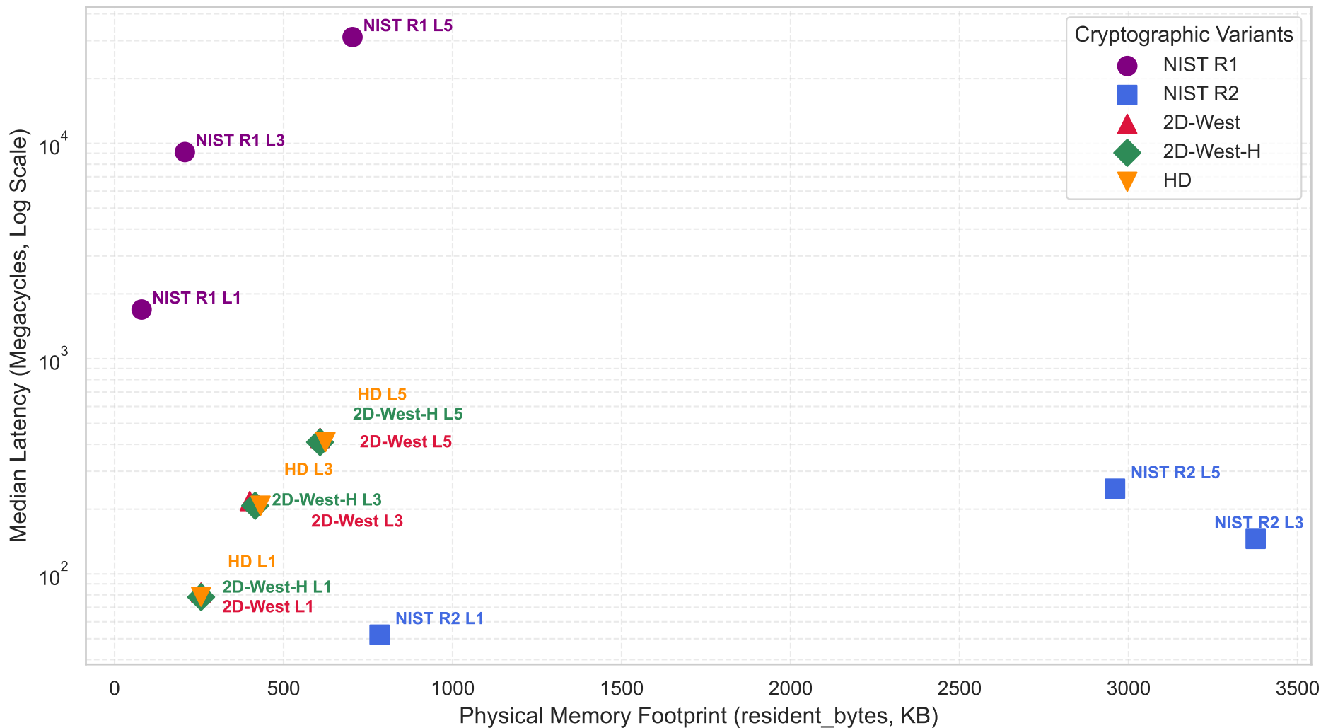
Keygen Latency vs. Physical Memory Footprint (resident_bytes)
