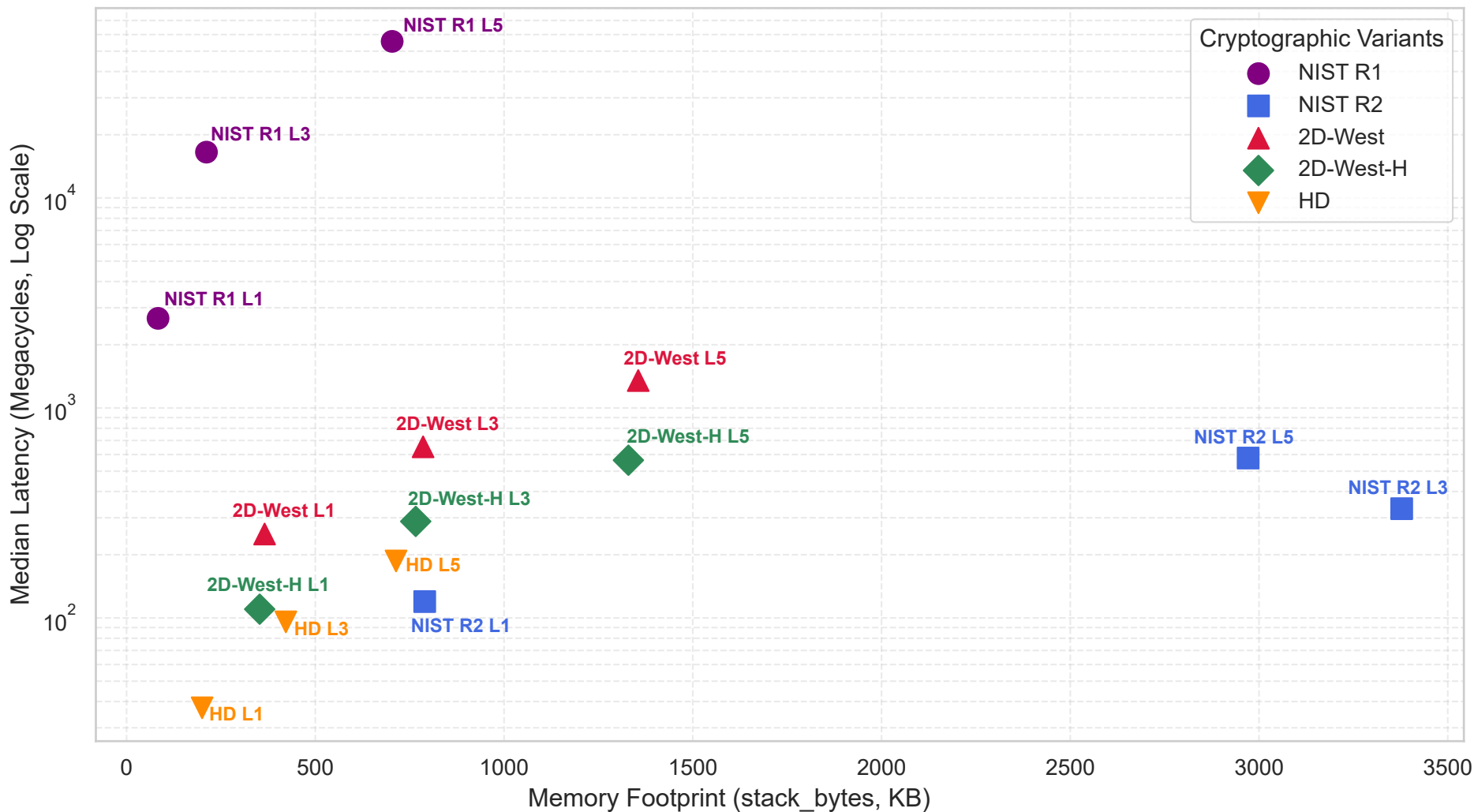
Signature Generation Latency vs. Memory Footprint (stack_bytes)
