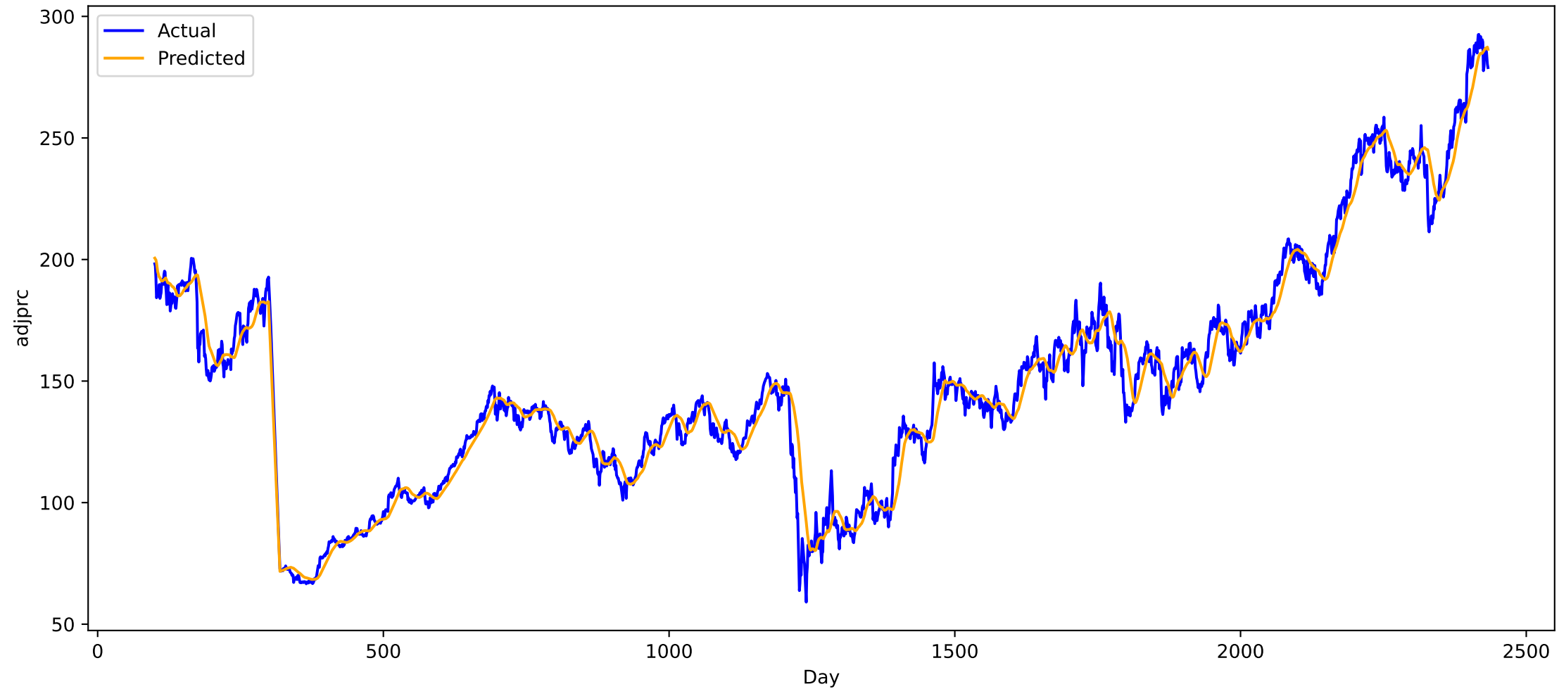
Predicted vs Actual for stock MAR (all), MAE: 5.648866176605225
