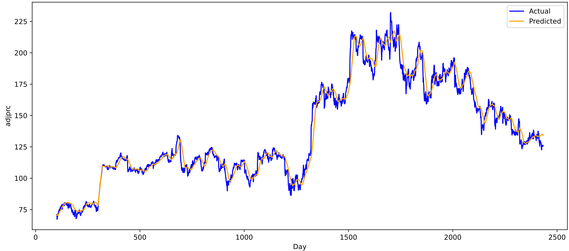
Predicted vs Actual for stock UPS (all), MAE: 4.600536823272705
