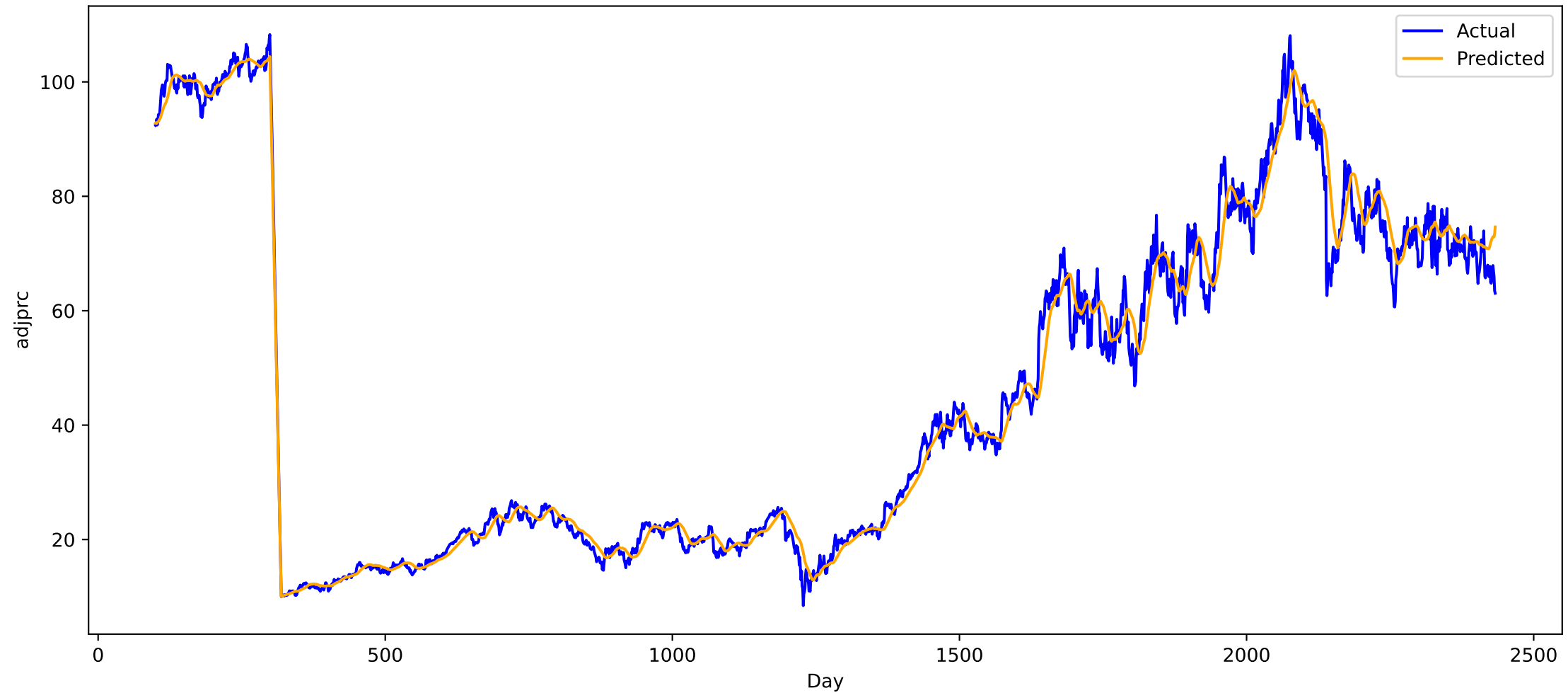
Predicted vs Actual for stock ON (all), MAE: 2.289071798324585
