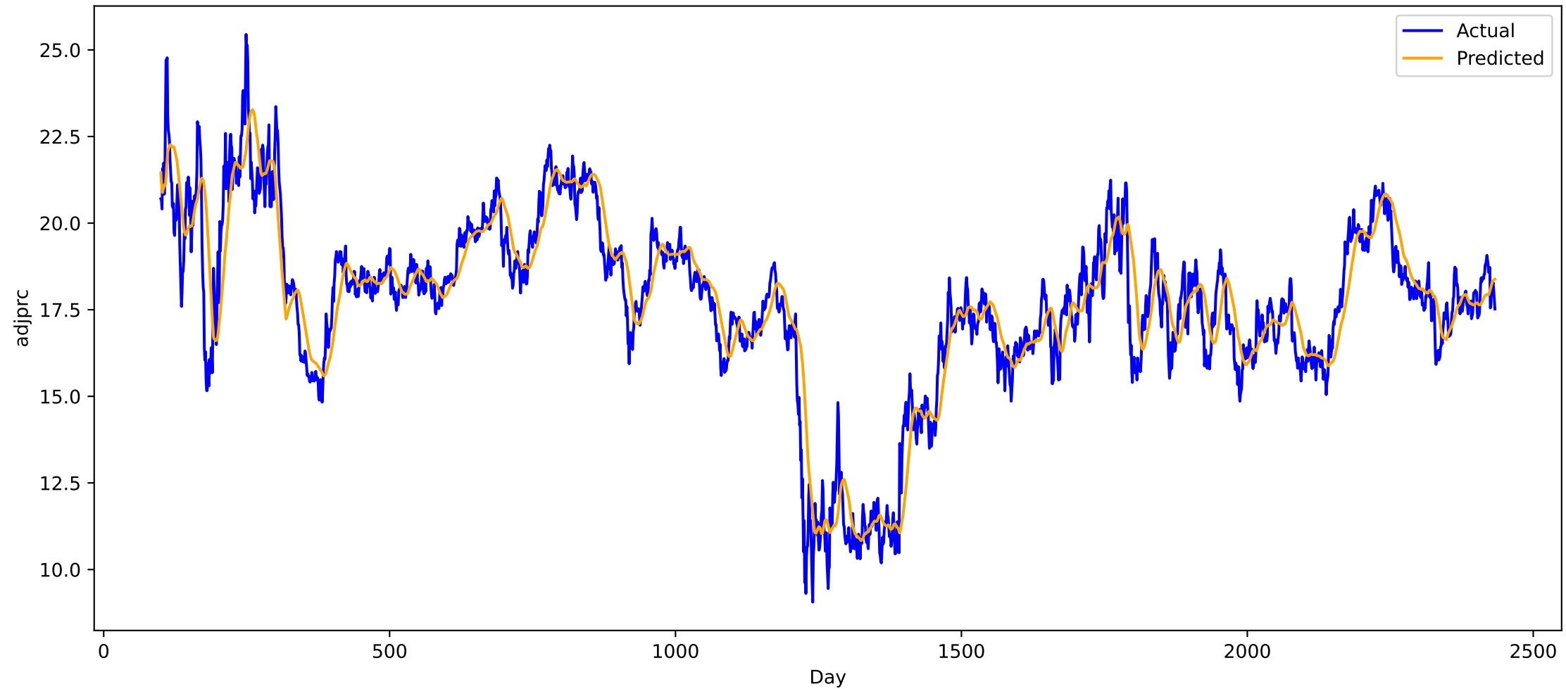
Predicted vs Actual for stock HST (all), MAE: 0.7033441662788391
