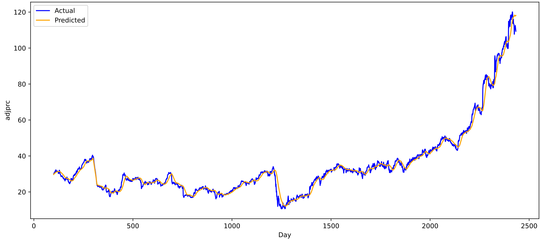
Predicted vs Actual for stock HWM (all), MAE: 1.5679173469543457
