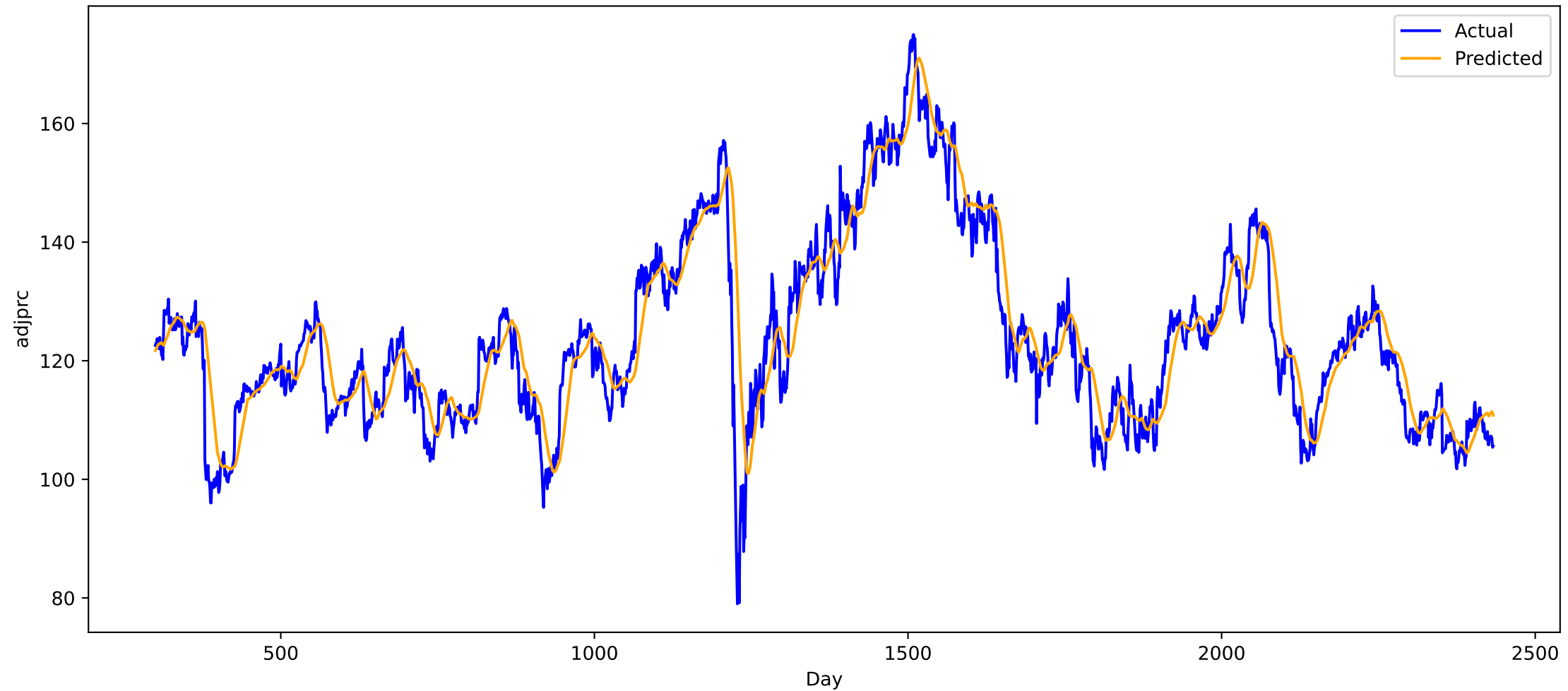
Predicted vs Actual for stock ZBH (all), MAE: 4.2281365394592285
