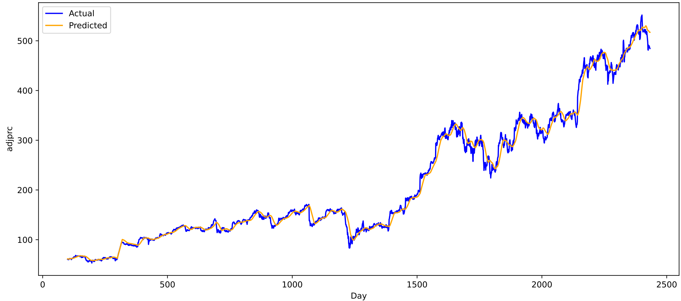
Predicted vs Actual for stock IT (all), MAE: 7.6262102127075195
