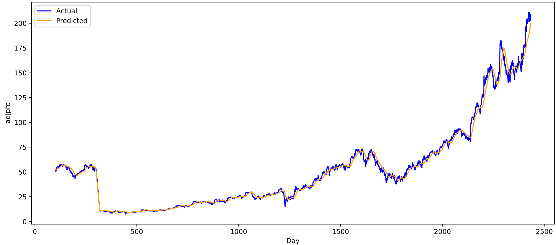
Predicted vs Actual for stock DECK (all), MAE: 2.5886971950531006
