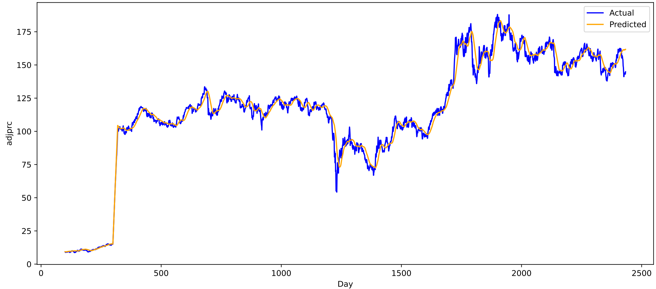
Predicted vs Actual for stock CVX (all), MAE: 3.8197360038757324
