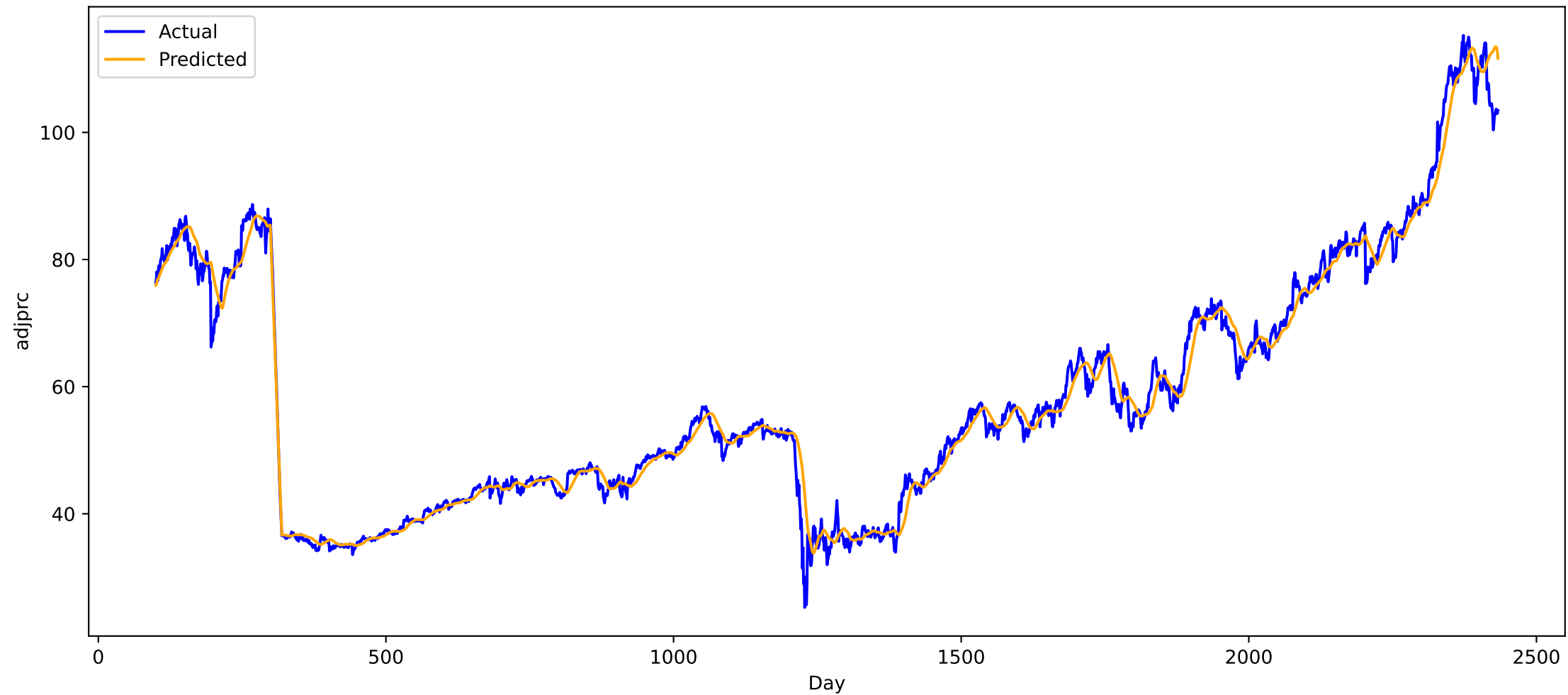
Predicted vs Actual for stock AFL (all), MAE: 1.612550139427185
