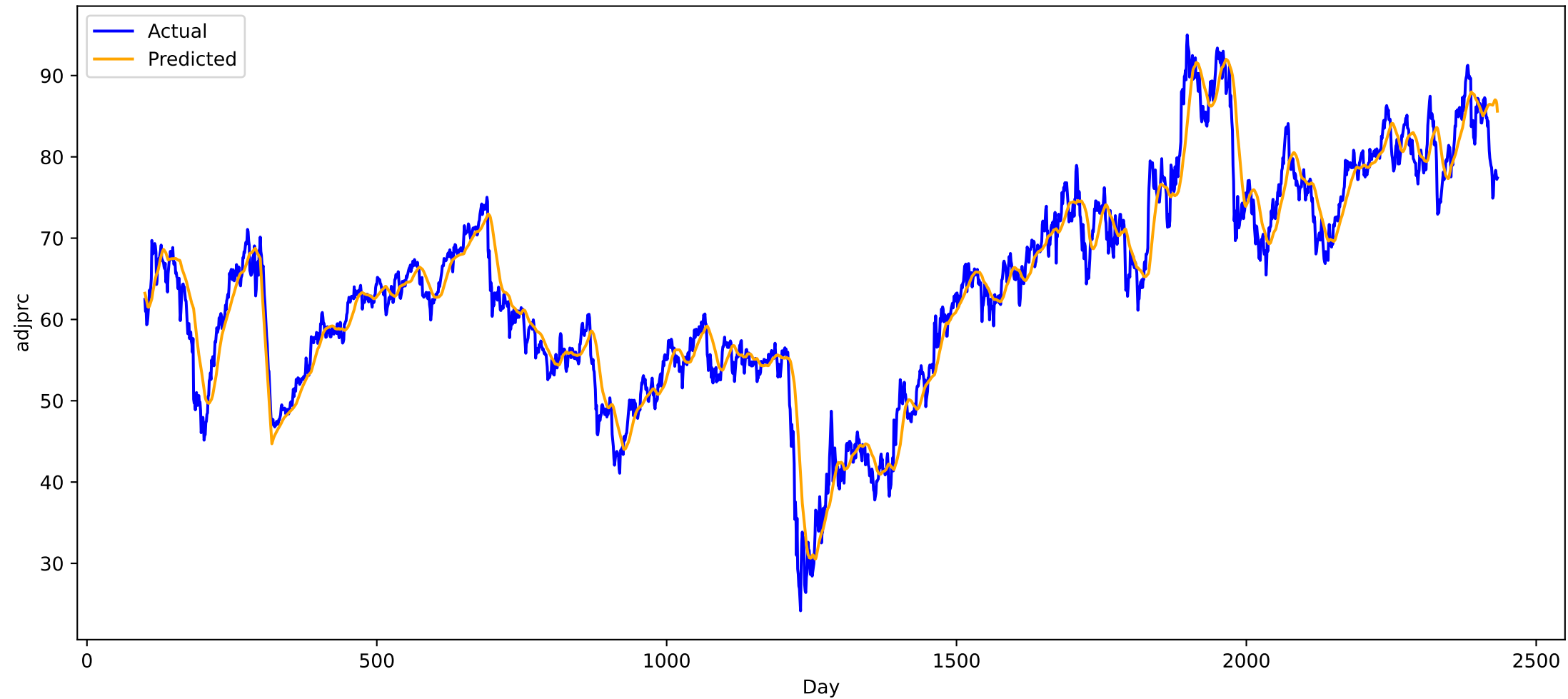
Predicted vs Actual for stock PFG (all), MAE: 2.351050853729248
