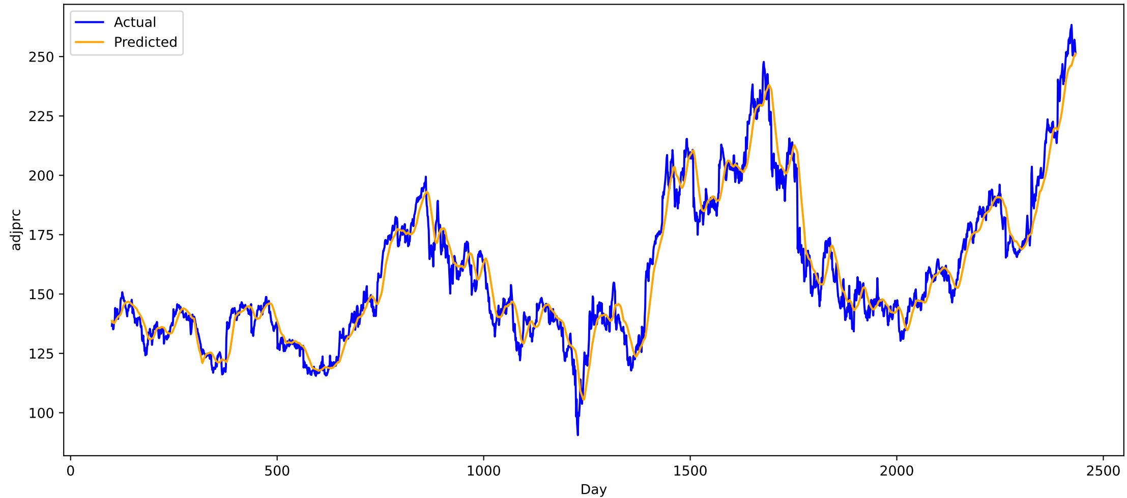
Predicted vs Actual for stock FFIV (all), MAE: 5.701138496398926
