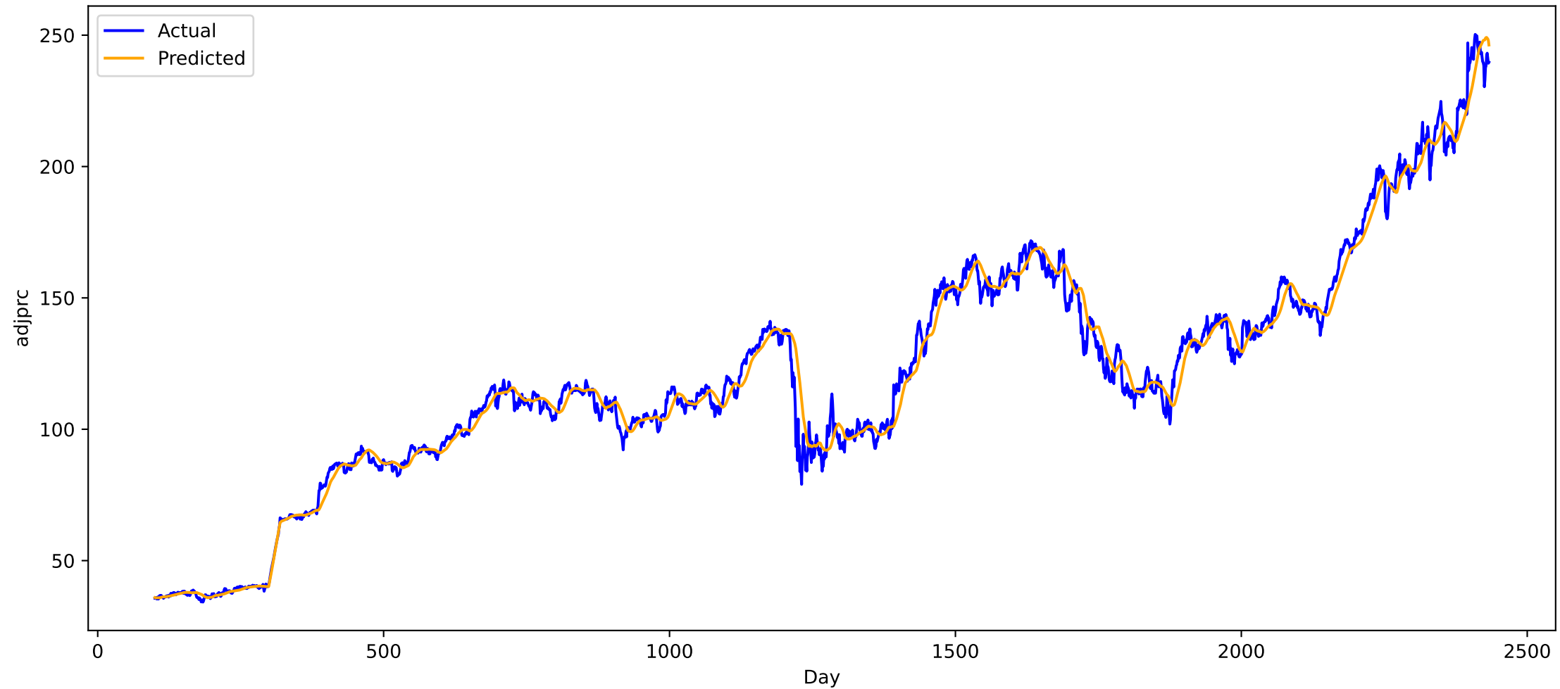
Predicted vs Actual for stock JPM (all), MAE: 3.824572801589966
