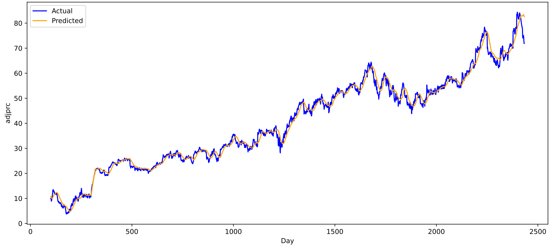
Predicted vs Actual for stock FAST (all), MAE: 1.4500446319580078
