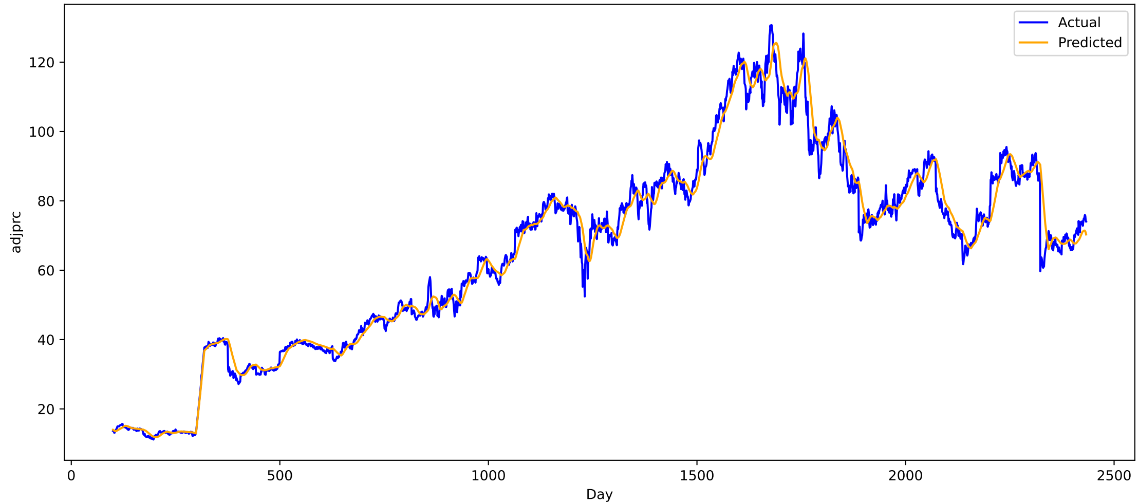
Predicted vs Actual for stock EW (all), MAE: 2.675748586654663
