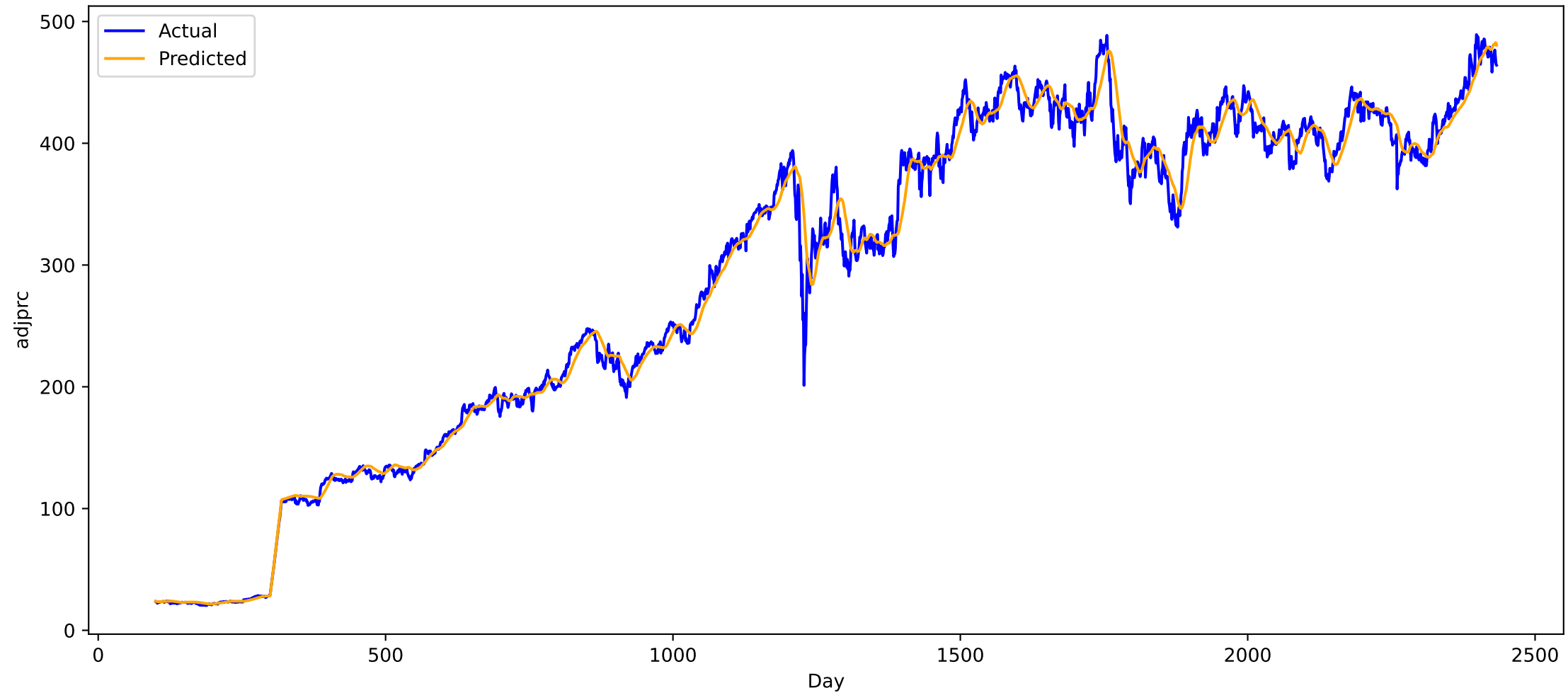
Predicted vs Actual for stock TDY (all), MAE: 9.188980102539062
