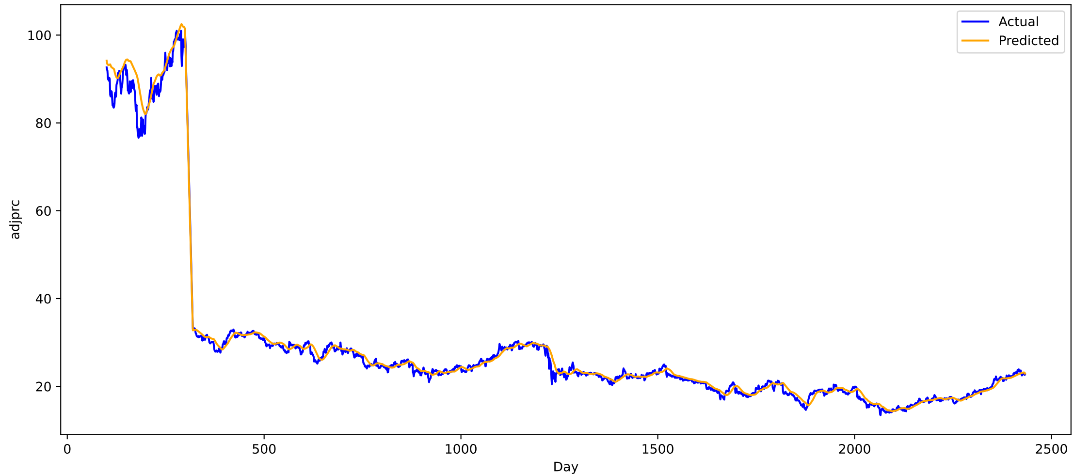
Predicted vs Actual for stock T (all), MAE: 0.901858389377594
