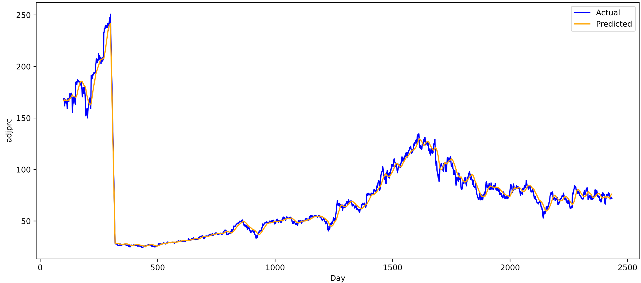
Predicted vs Actual for stock TECH (all), MAE: 3.237626552581787
