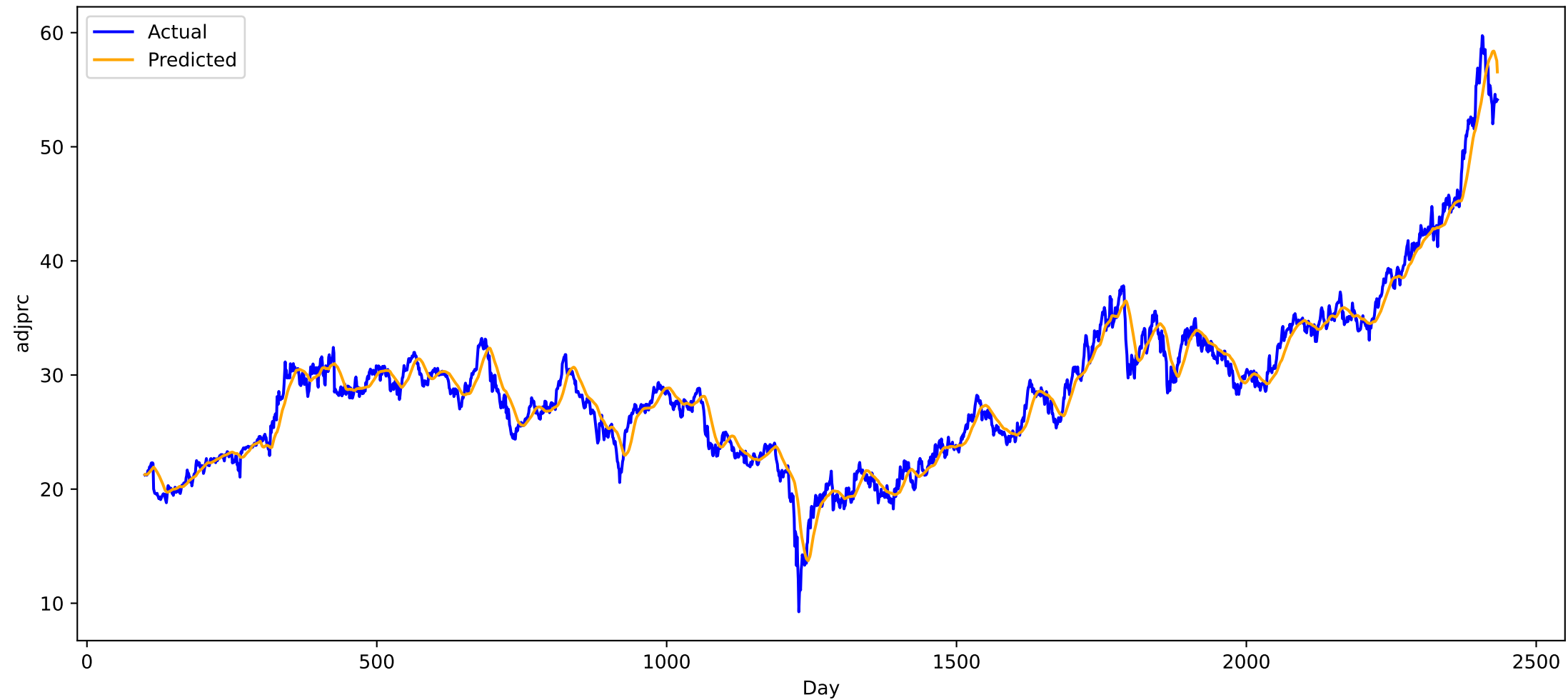
Predicted vs Actual for stock WMB (all), MAE: 0.9806333184242249
