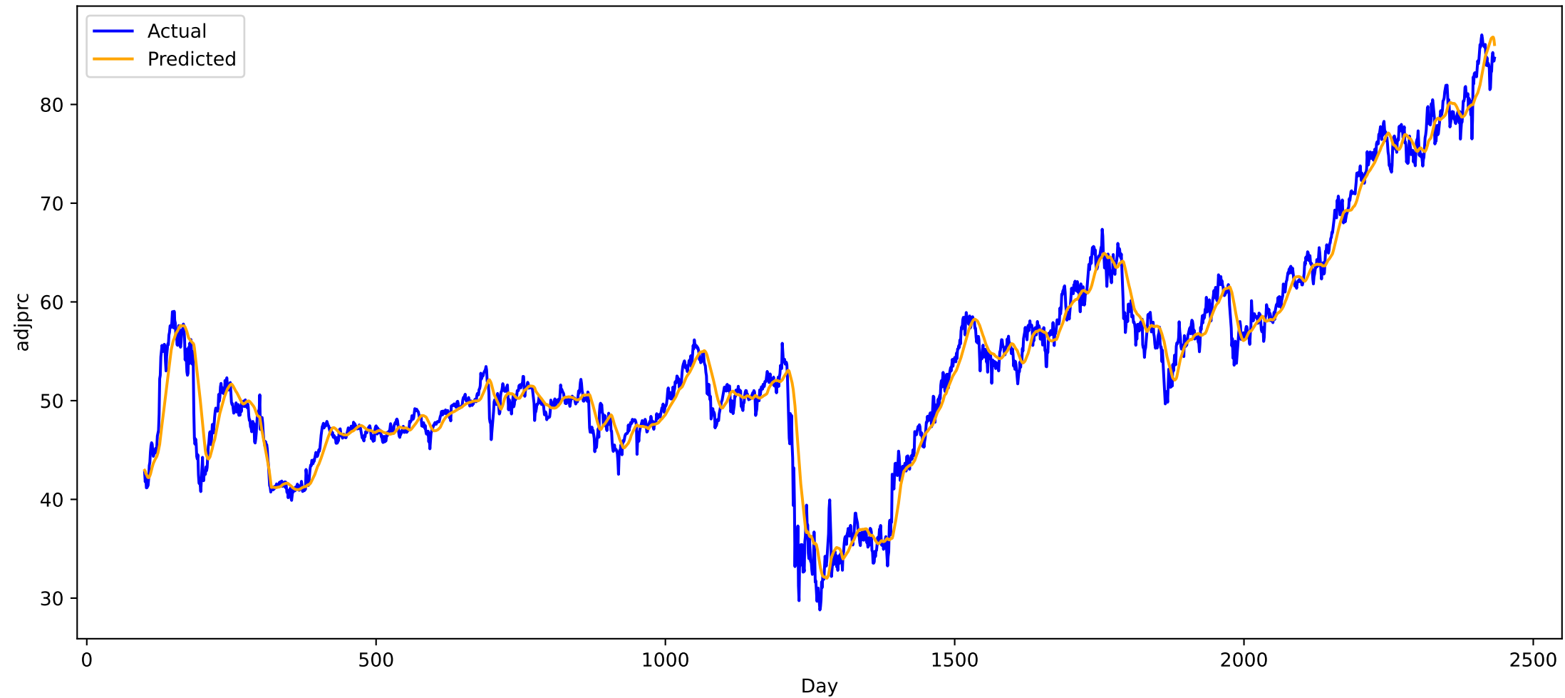
Predicted vs Actual for stock L (all), MAE: 1.4092875719070435
