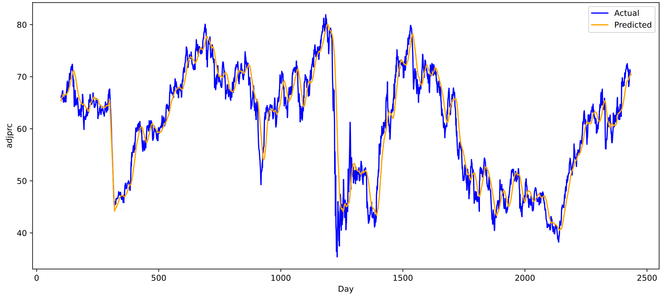
Predicted vs Actual for stock C (all), MAE: 2.269148826599121
