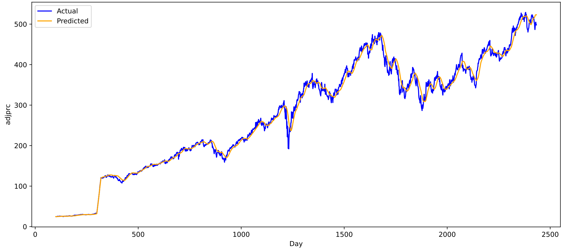
Predicted vs Actual for stock SPGI (all), MAE: 8.678832054138184
