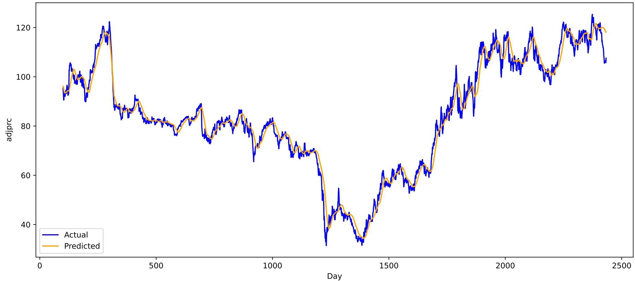
Predicted vs Actual for stock XOM (all), MAE: 2.704681396484375
