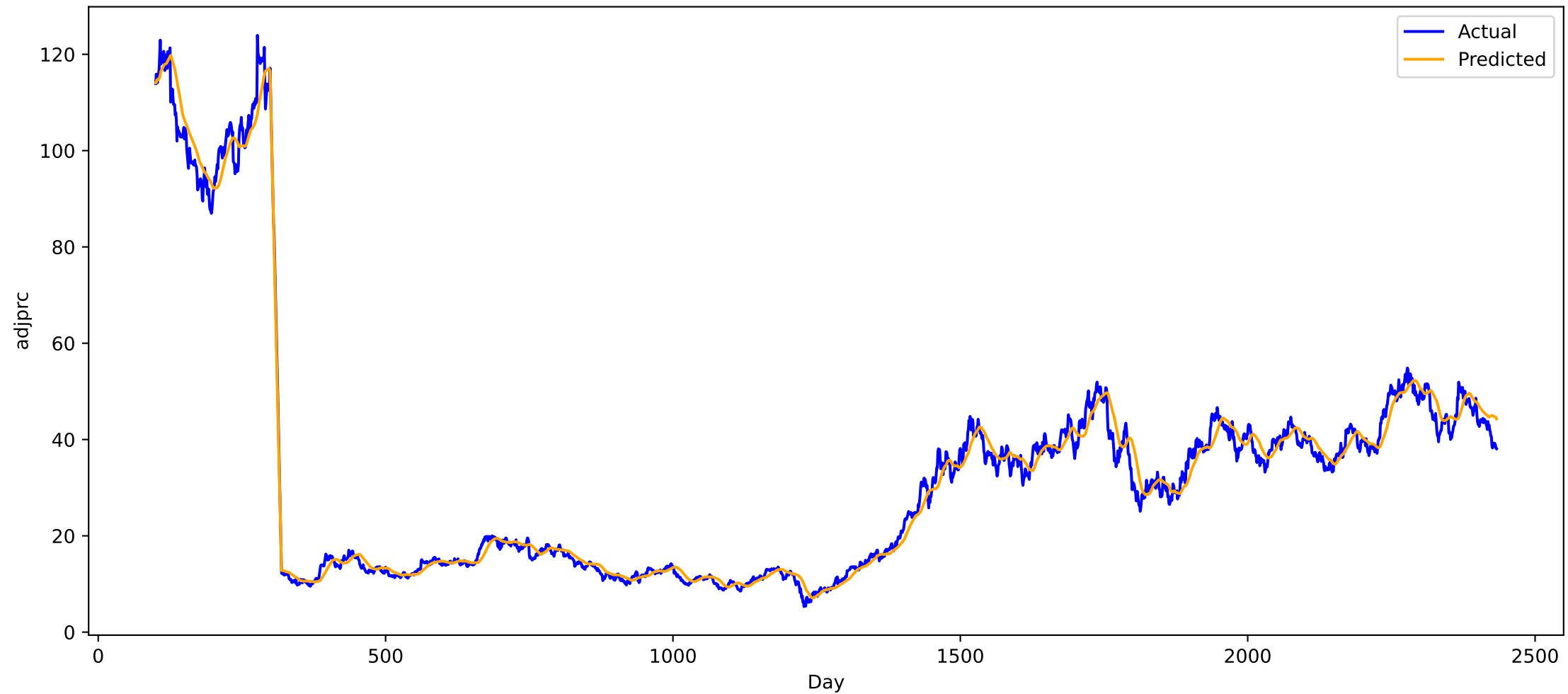
Predicted vs Actual for stock FCX (all), MAE: 1.8001666069030762
