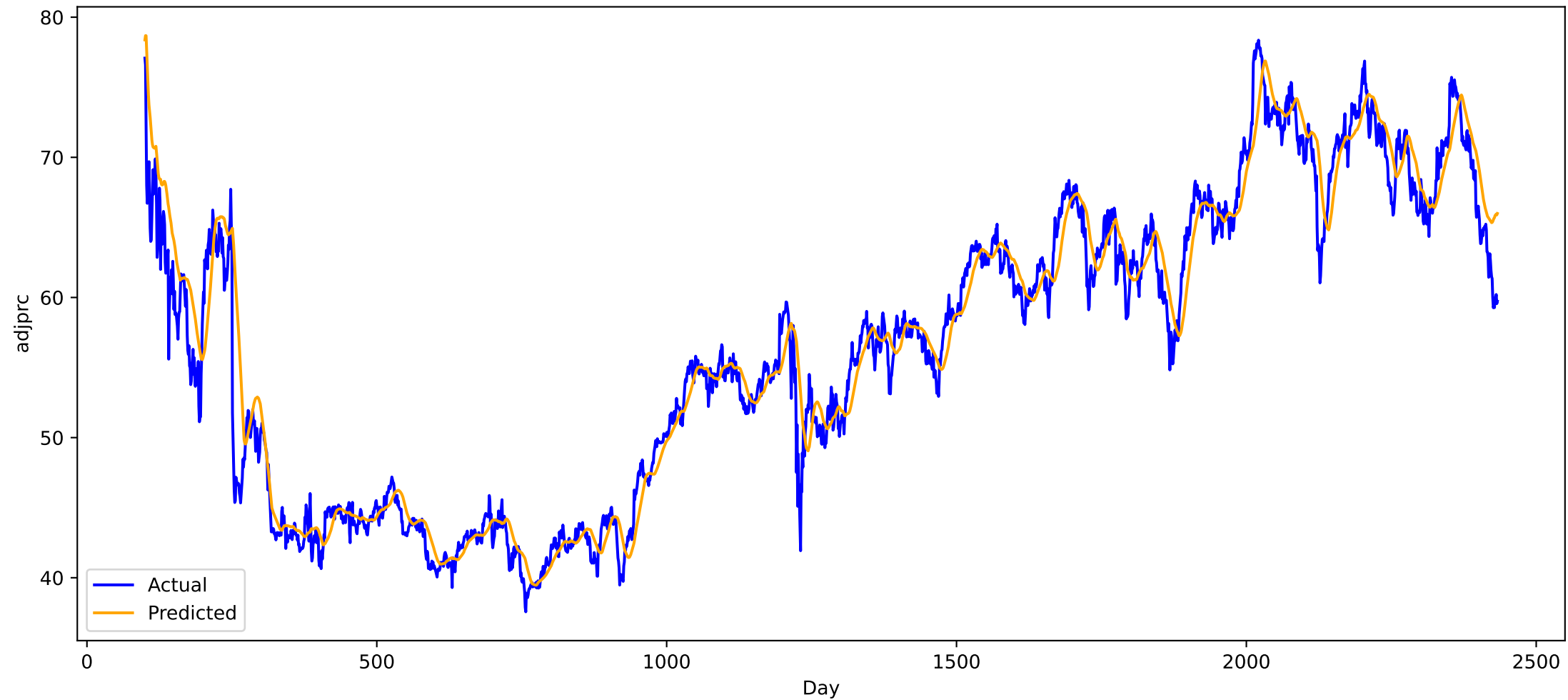
Predicted vs Actual for stock MDLZ (all), MAE: 1.5968542098999023
