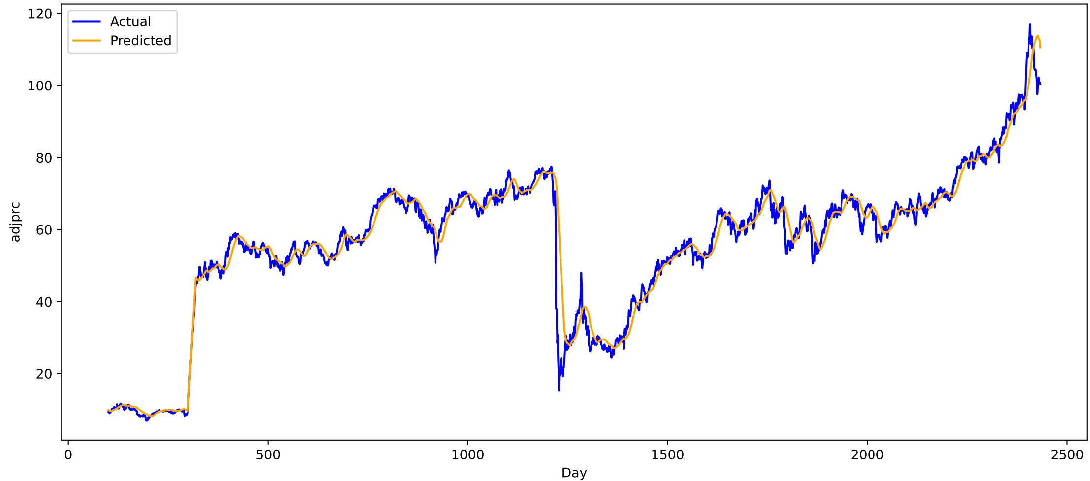
Predicted vs Actual for stock OKE (all), MAE: 2.2645654678344727
