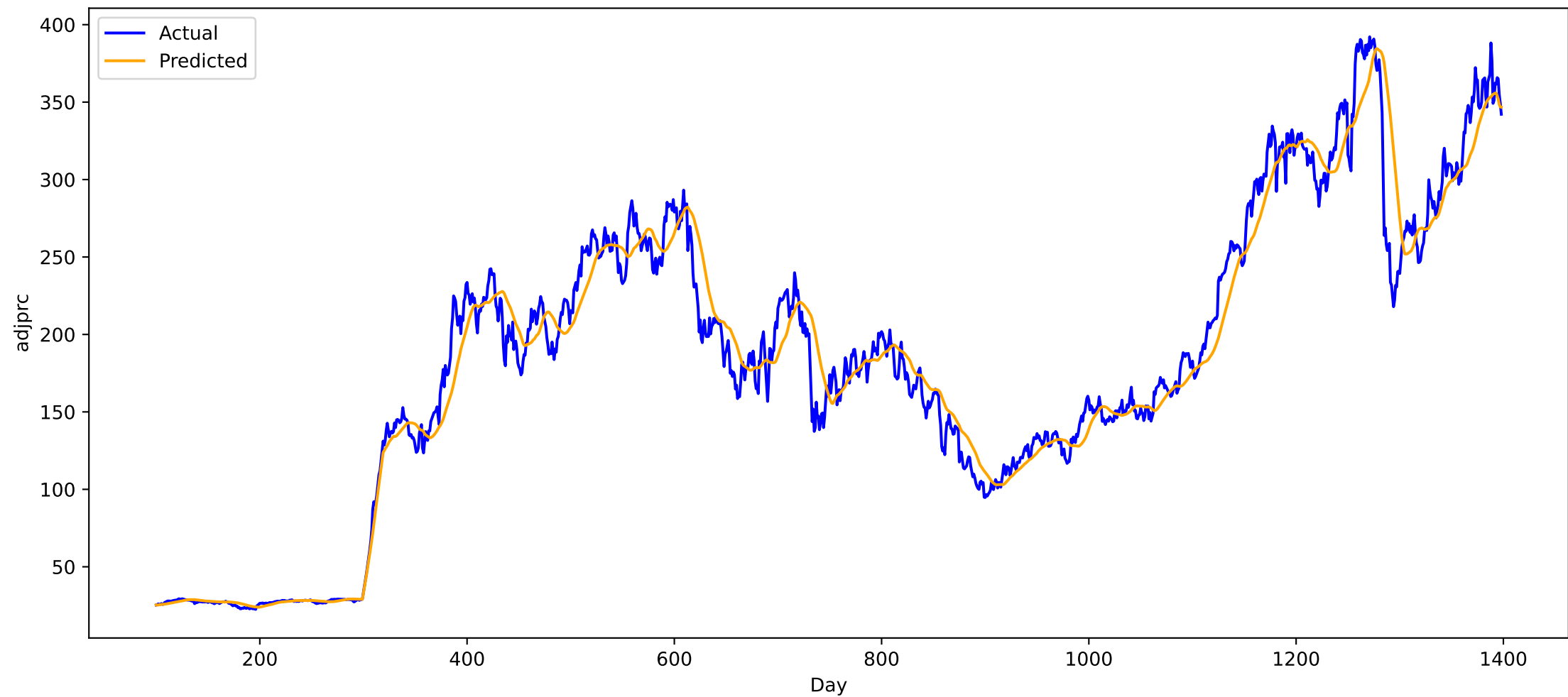
Predicted vs Actual for stock CRWD (all), MAE: 12.460086822509766
