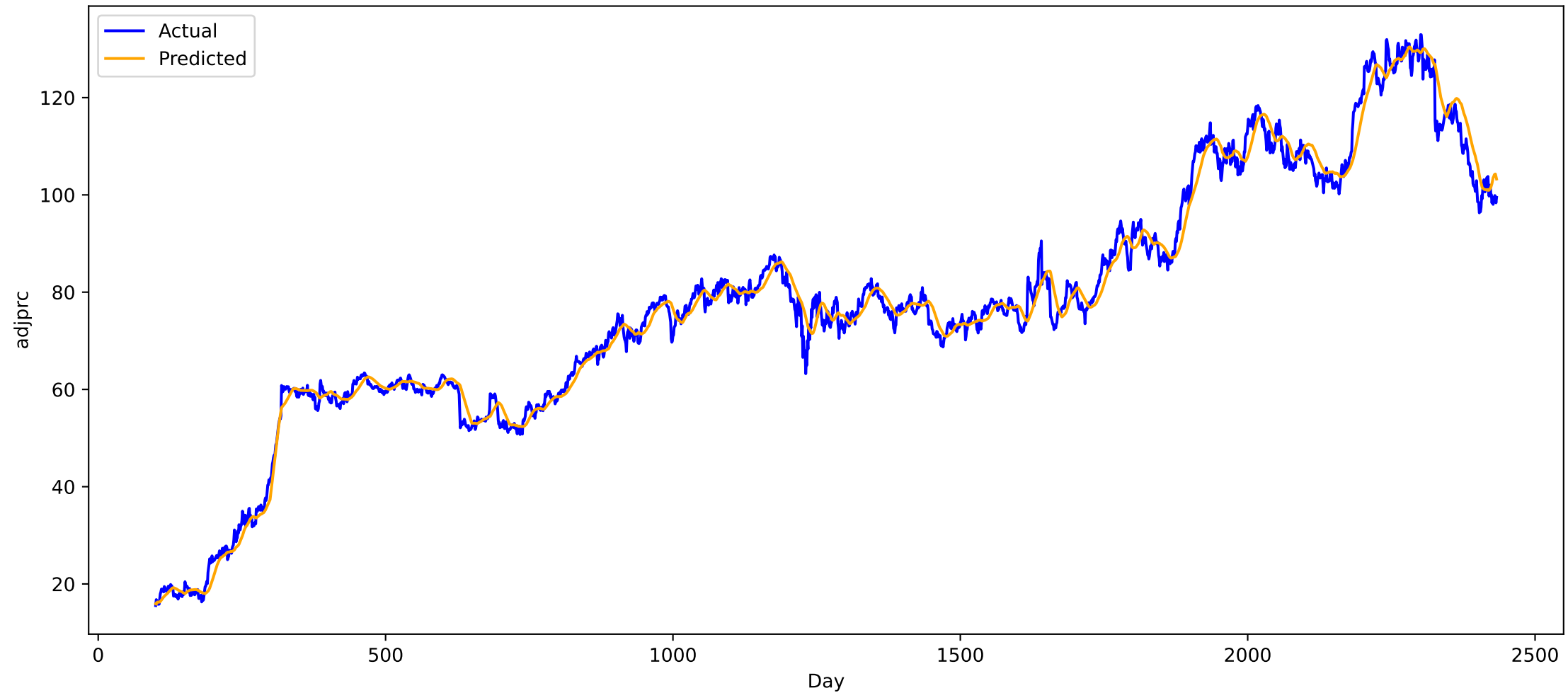
Predicted vs Actual for stock MRK (all), MAE: 2.180987596511841
