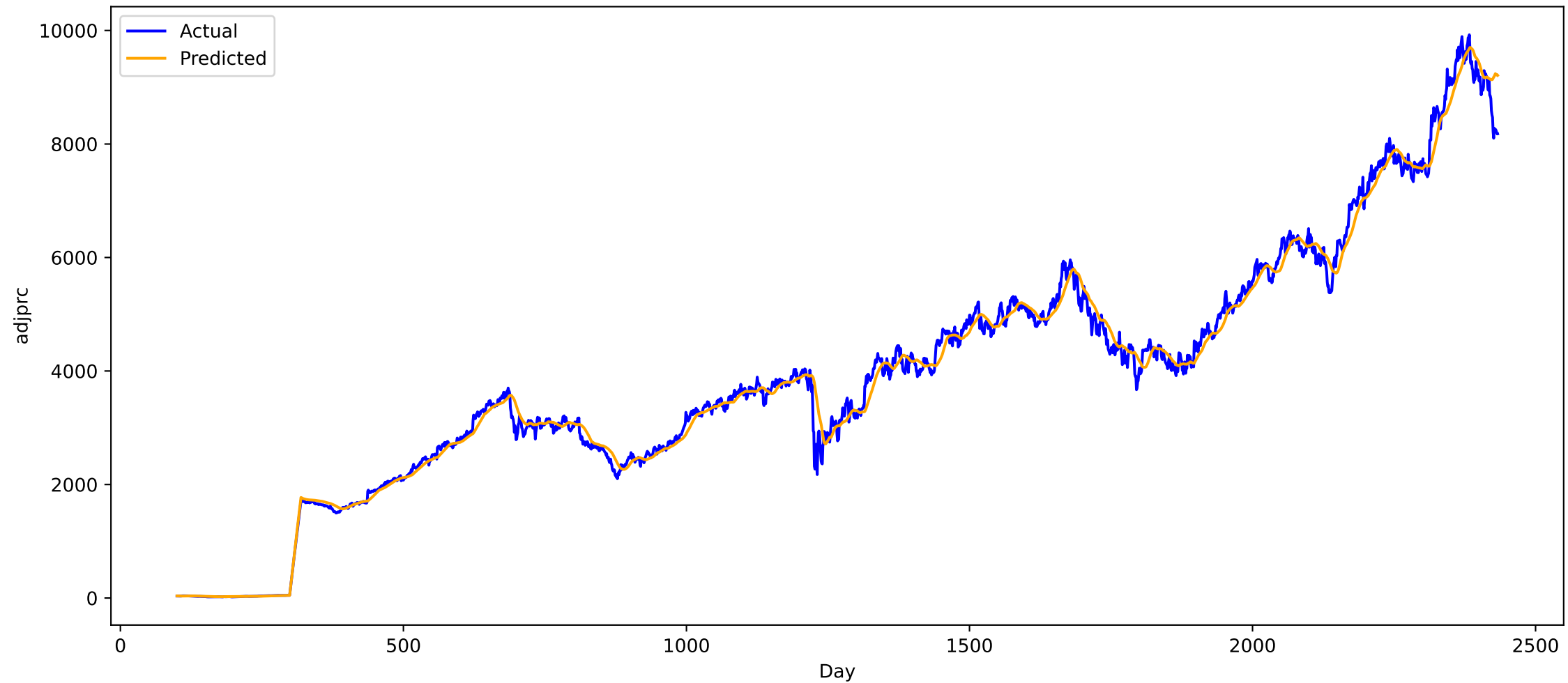
Predicted vs Actual for stock NVR (all), MAE: 134.5380401611328
