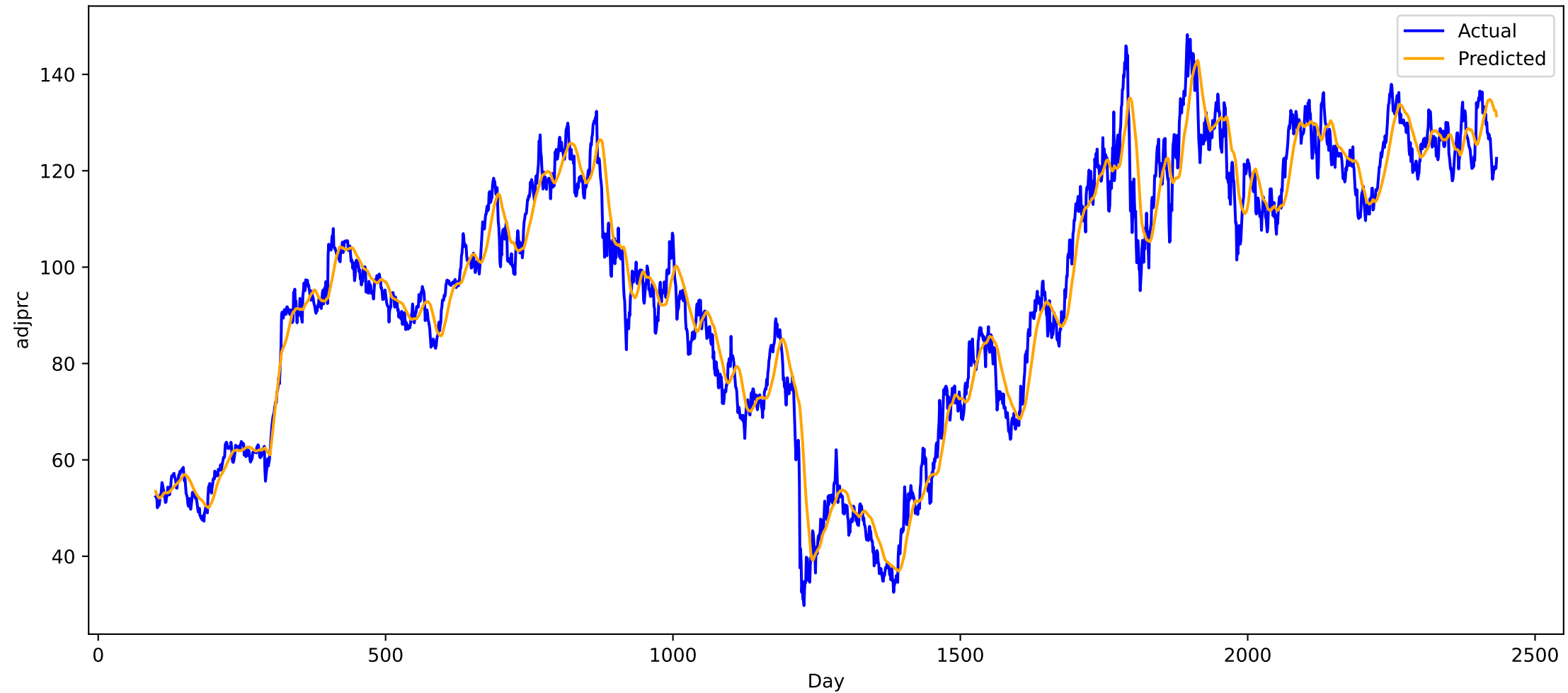
Predicted vs Actual for stock EOG (all), MAE: 4.336812496185303
