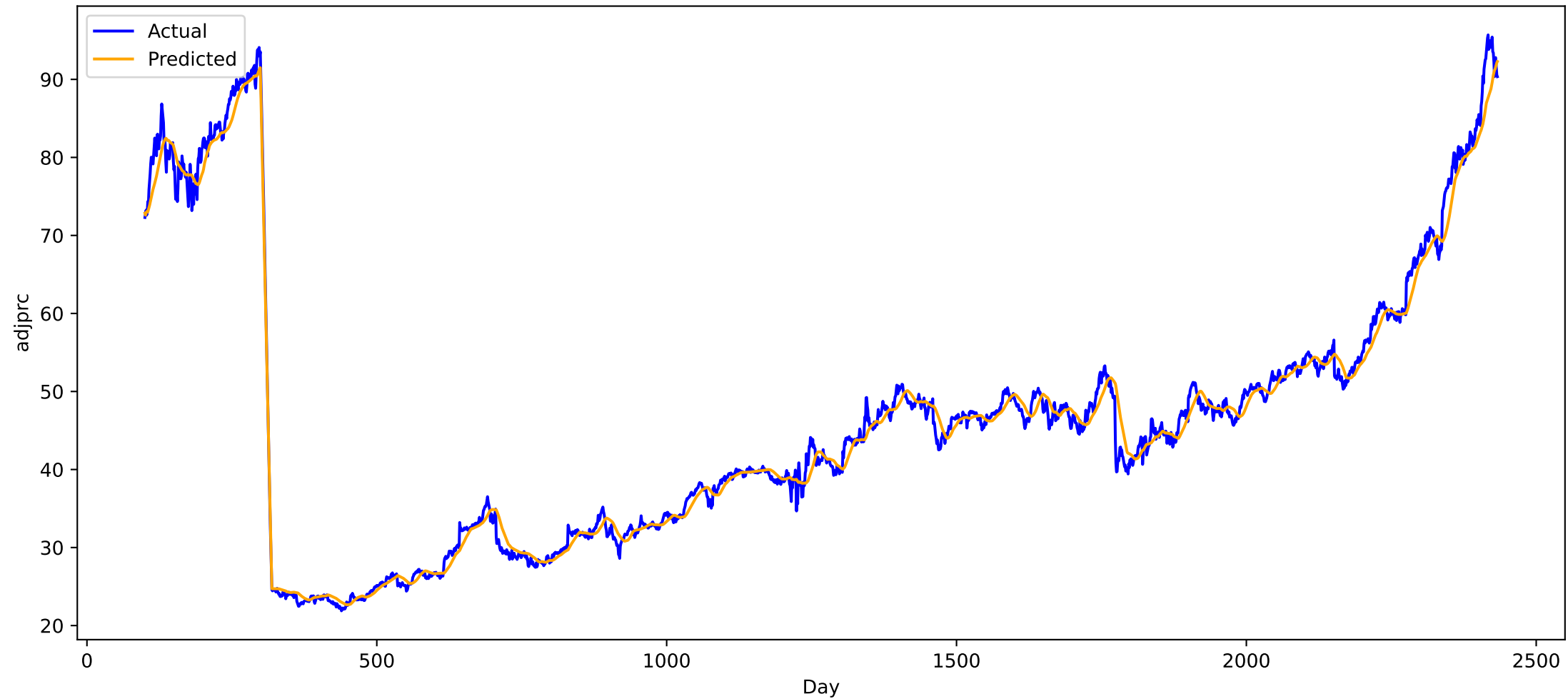
Predicted vs Actual for stock WMT (all), MAE: 1.1713670492172241
