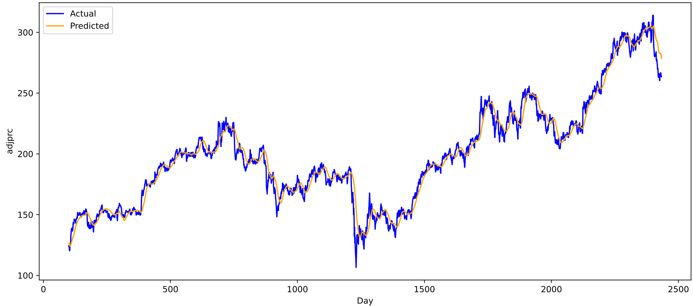
Predicted vs Actual for stock GD (all), MAE: 5.078924179077148
