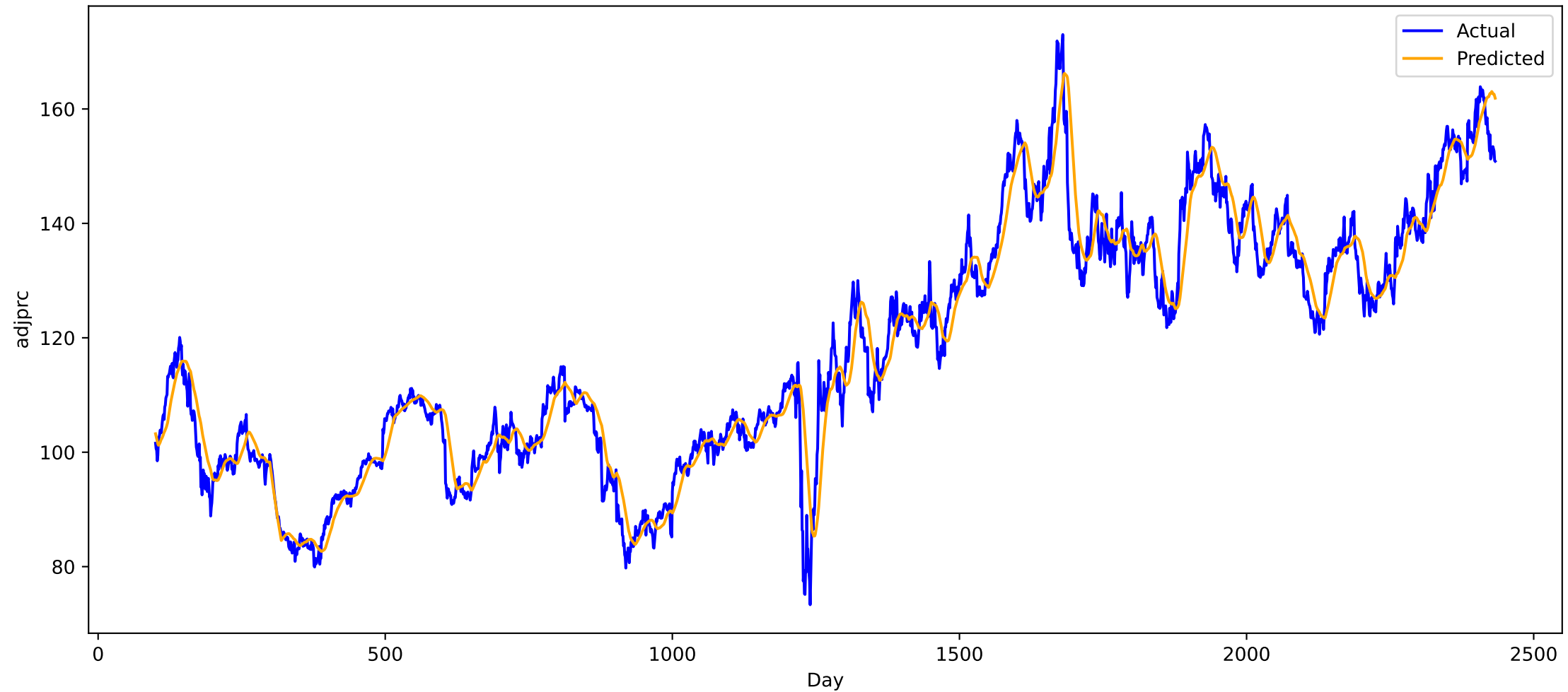
Predicted vs Actual for stock DGX (all), MAE: 3.5172665119171143
