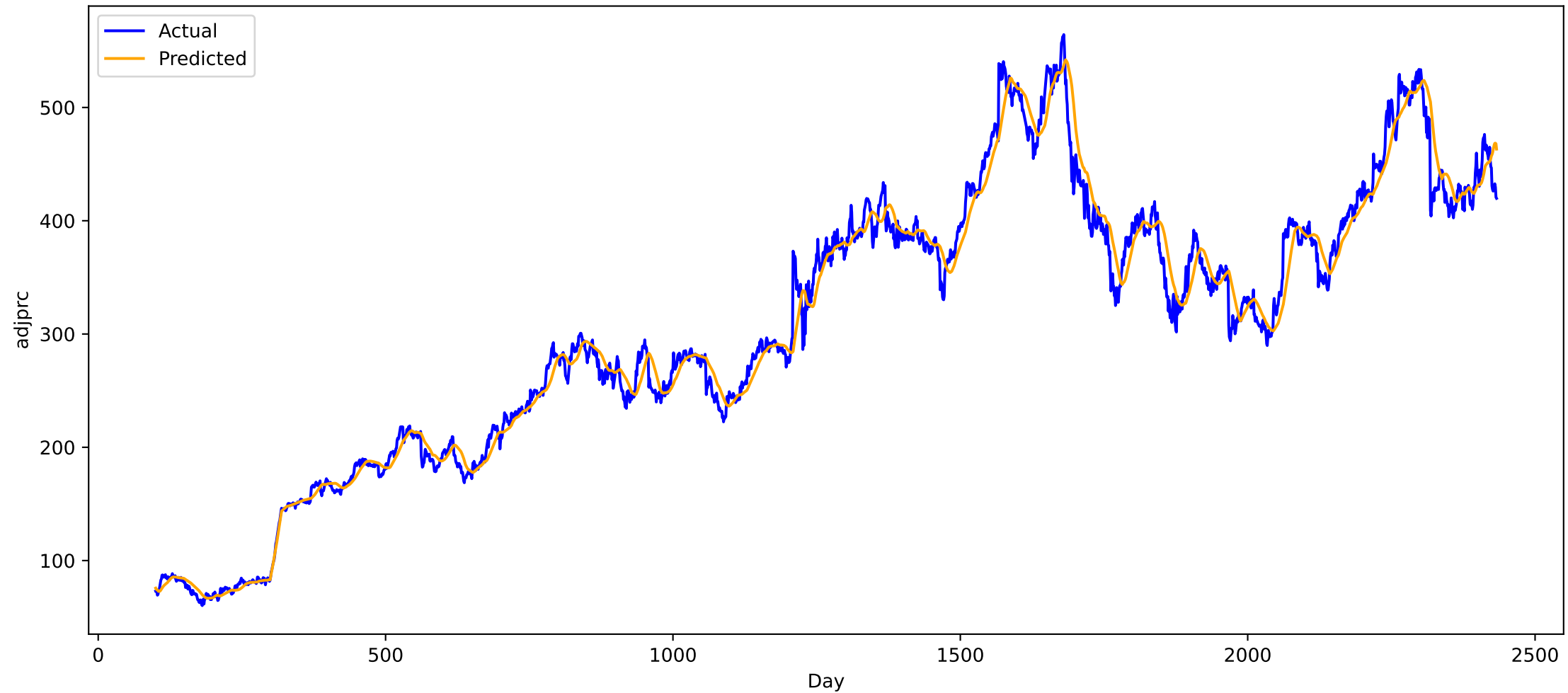
Predicted vs Actual for stock DPZ (all), MAE: 11.882258415222168
