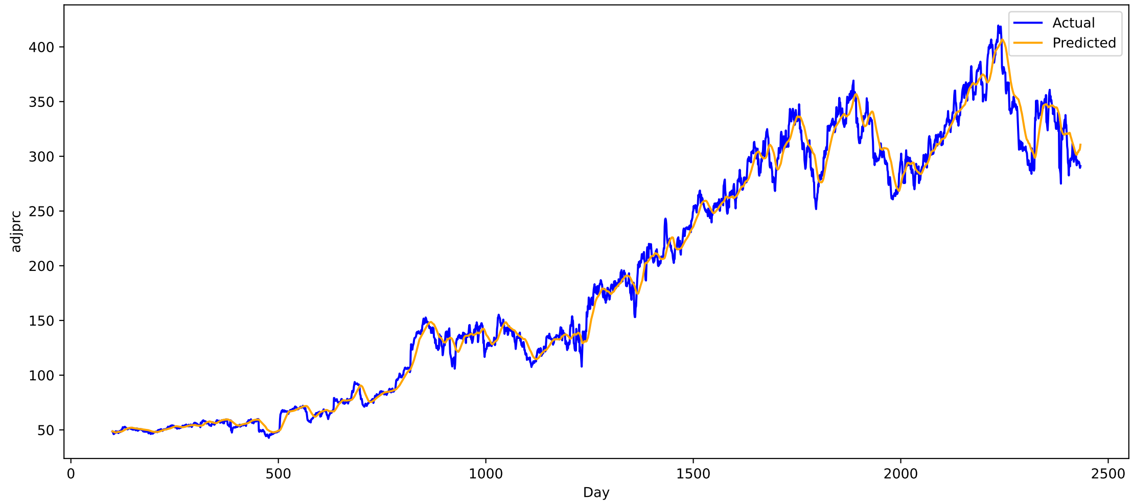
Predicted vs Actual for stock MOH (all), MAE: 8.112724304199219
