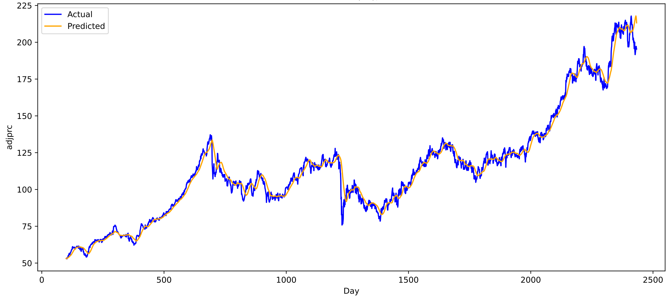
Predicted vs Actual for stock CBOE (all), MAE: 3.2723562717437744
