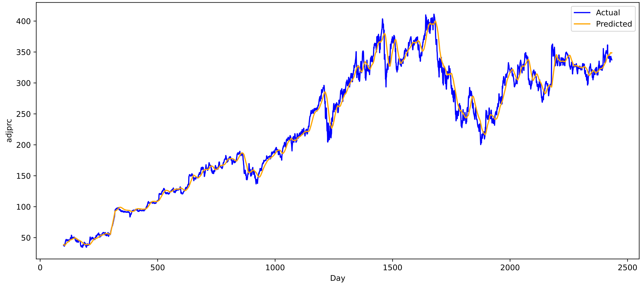
Predicted vs Actual for stock ANSS (all), MAE: 8.72858715057373
