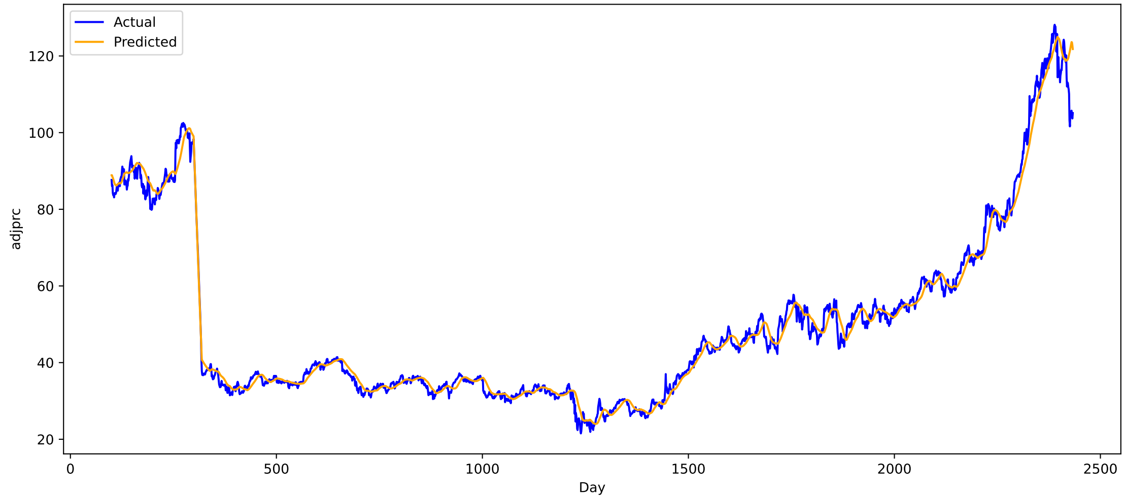
Predicted vs Actual for stock IRM (all), MAE: 1.8031067848205566
