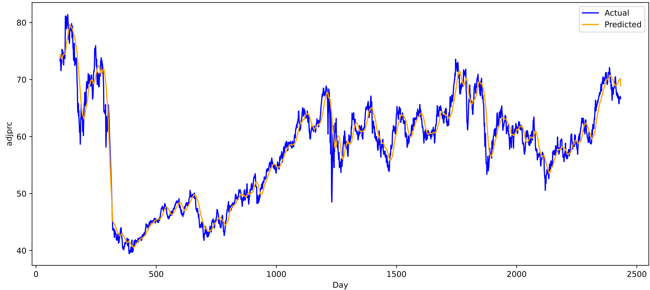
Predicted vs Actual for stock CMS (all), MAE: 1.4894657135009766
