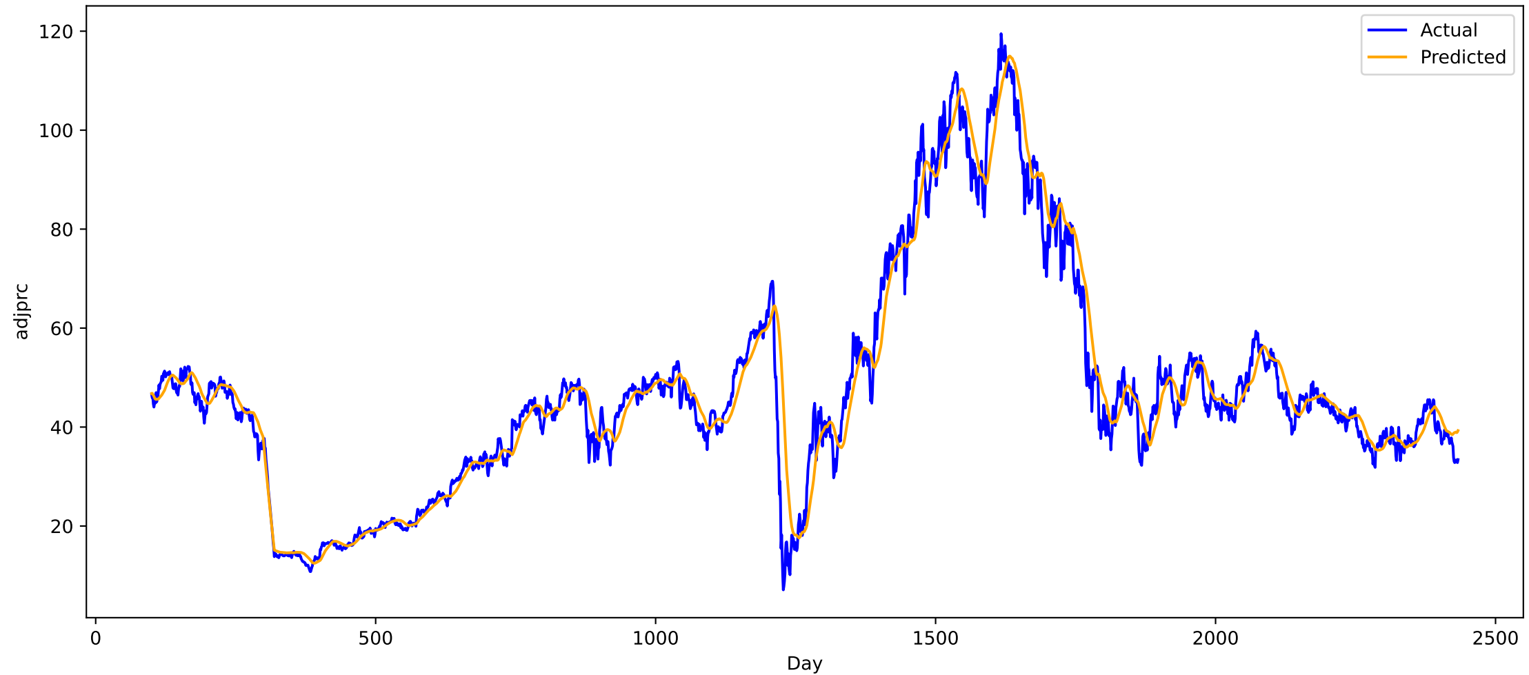
Predicted vs Actual for stock CZR (all), MAE: 3.2017648220062256
