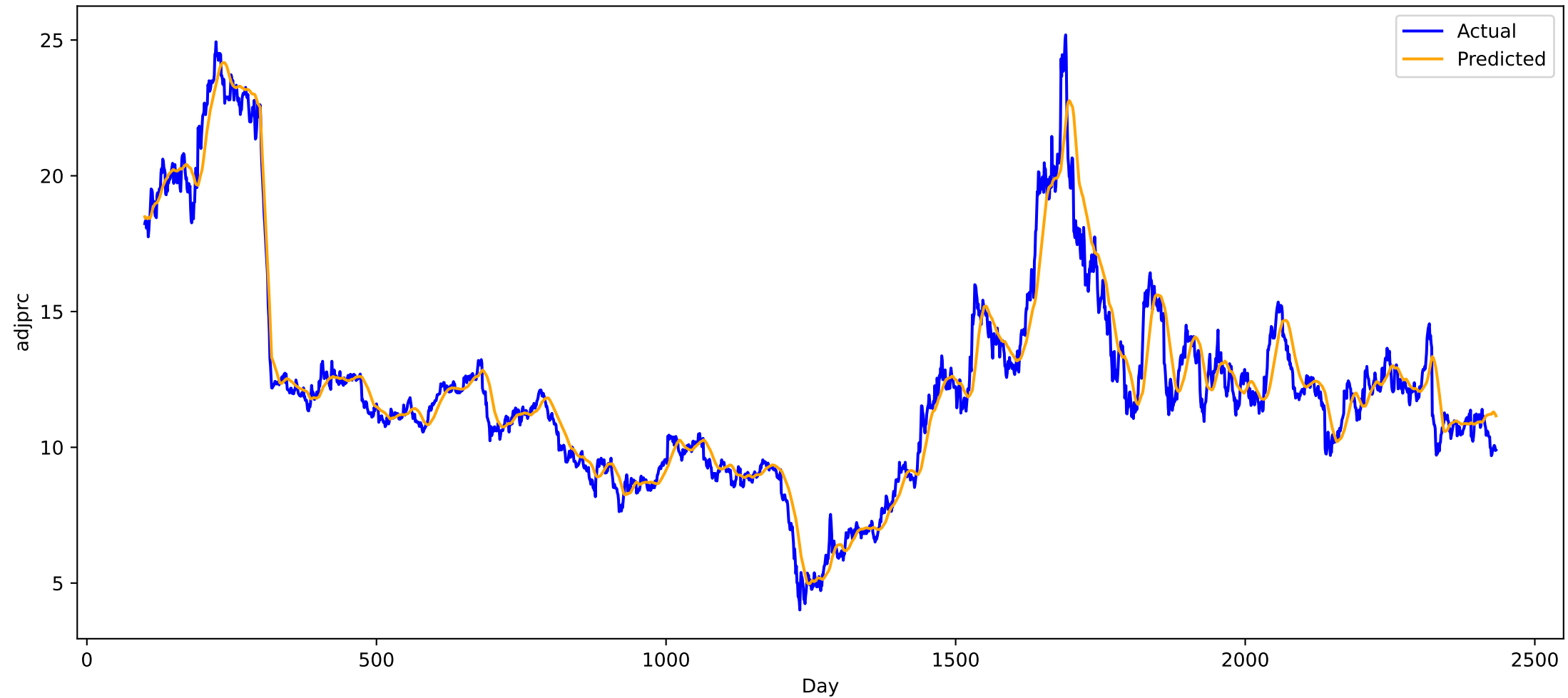
Predicted vs Actual for stock F (all), MAE: 0.5950244665145874
