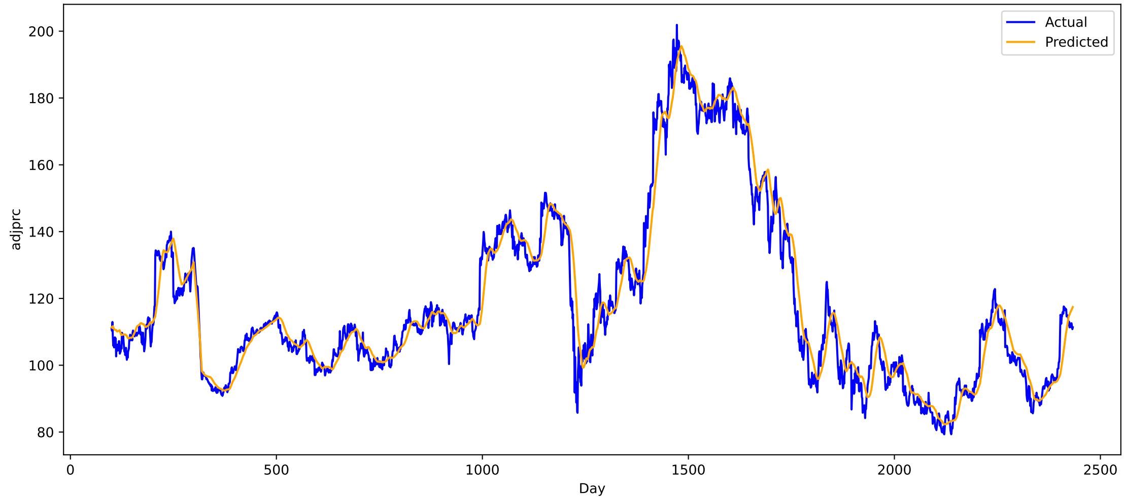
Predicted vs Actual for stock DIS (all), MAE: 4.153318881988525
