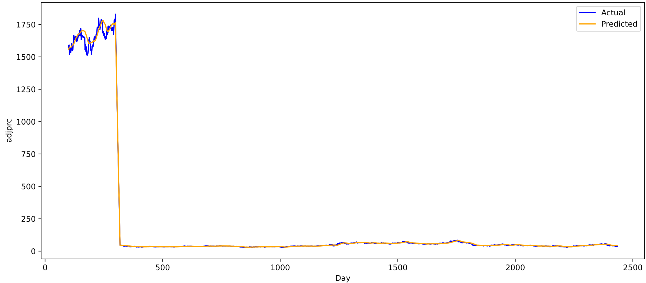
Predicted vs Actual for stock NEM (all), MAE: 5.50050687789917
