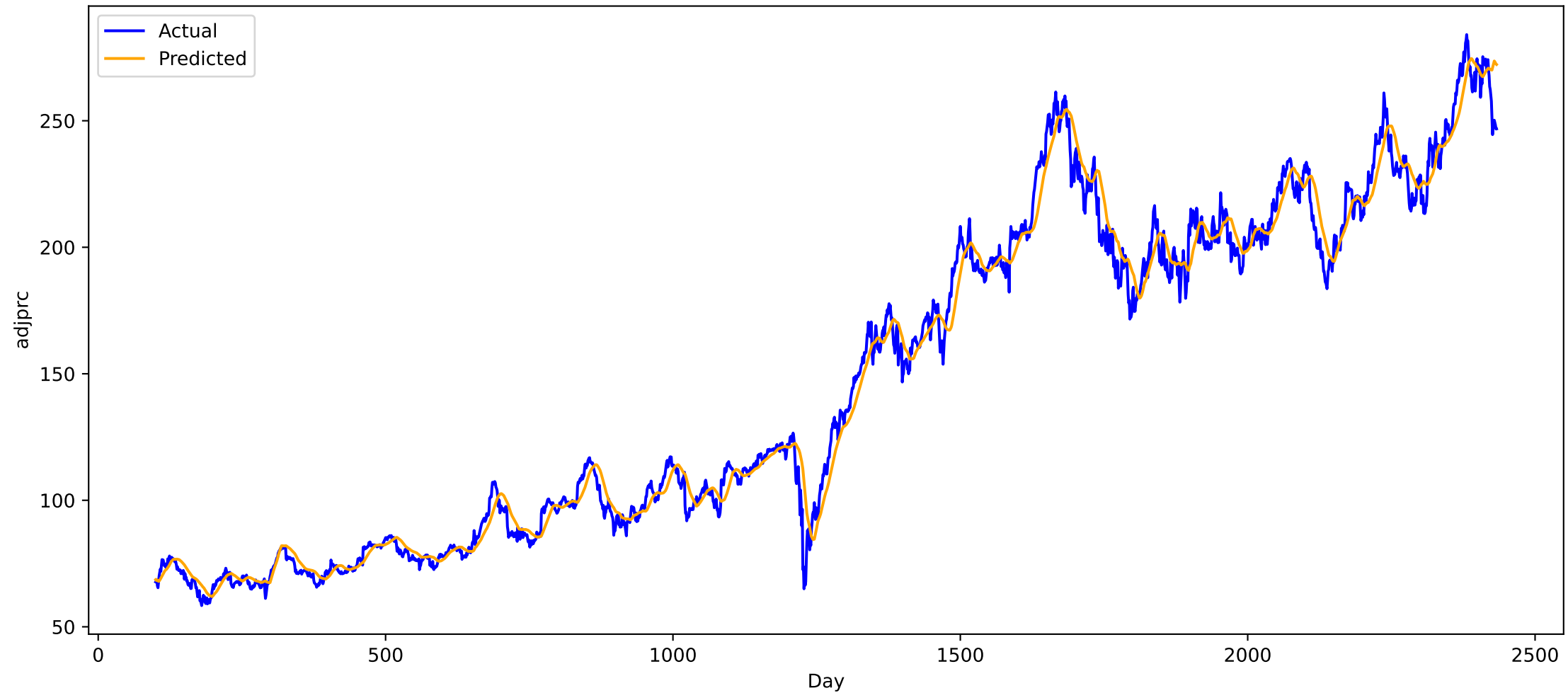
Predicted vs Actual for stock LOW (all), MAE: 5.426214218139648
