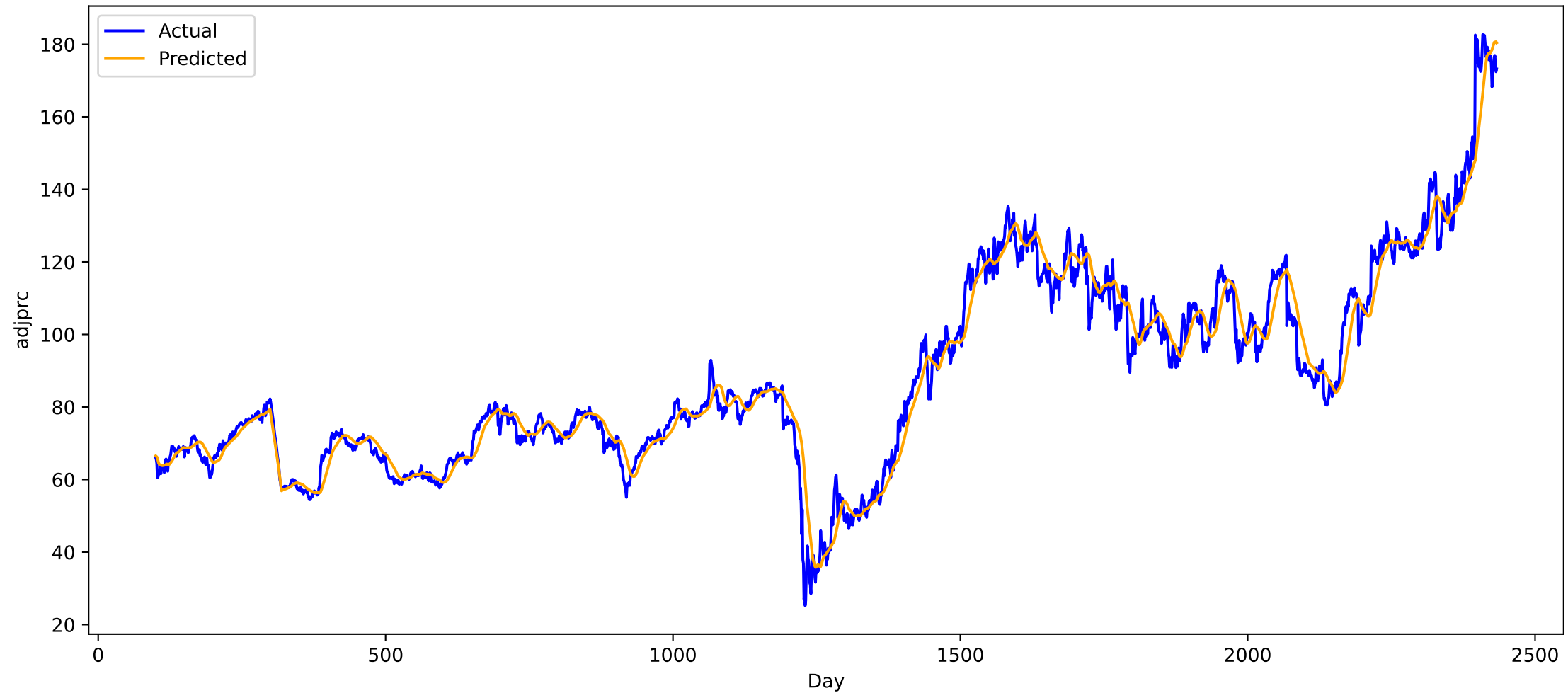
Predicted vs Actual for stock DFS (all), MAE: 3.6929702758789062
