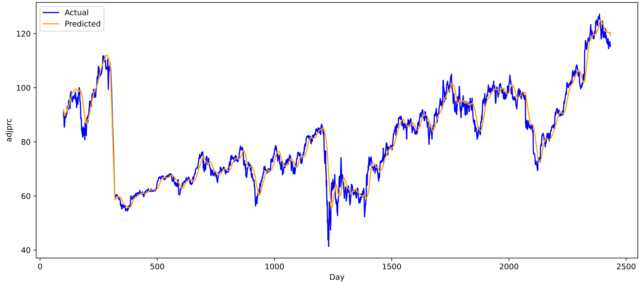
Predicted vs Actual for stock RTX (all), MAE: 2.532026767730713
