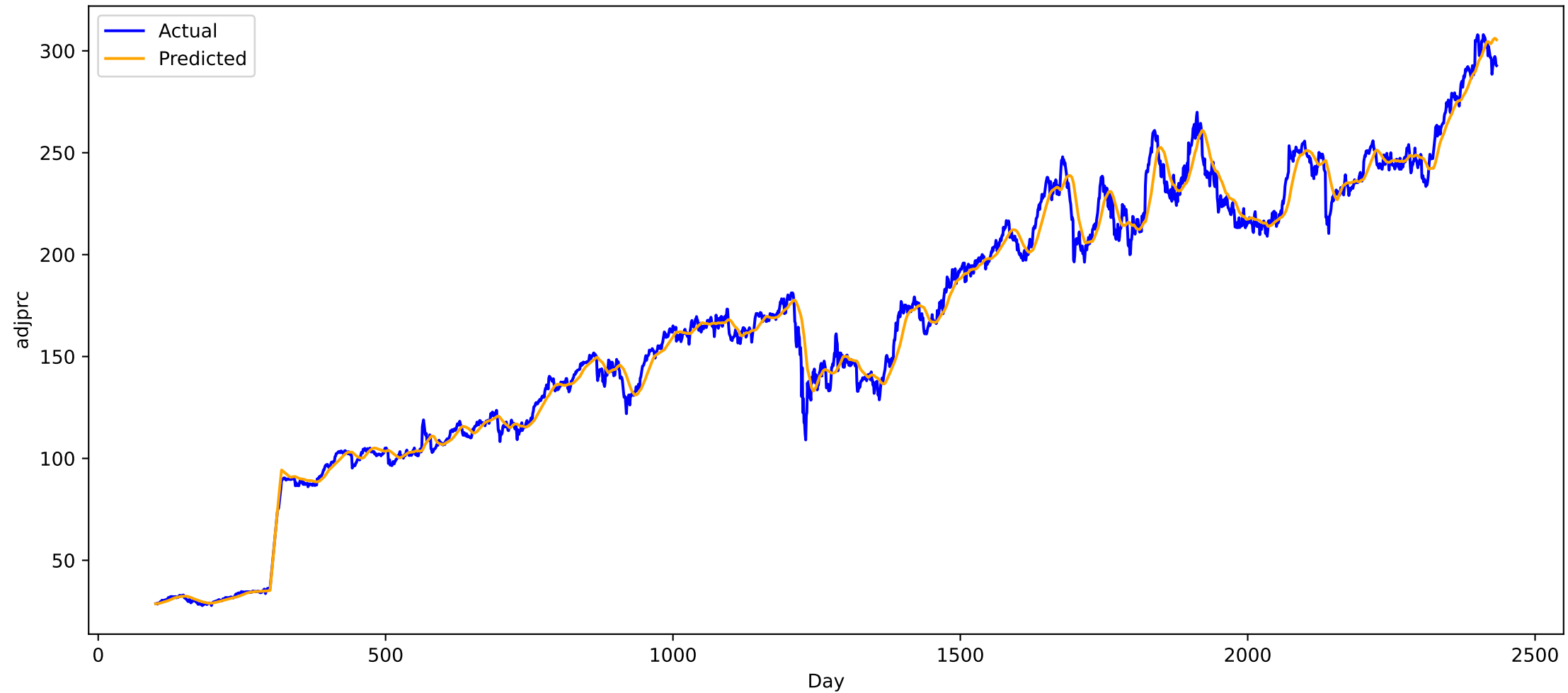
Predicted vs Actual for stock ADP (all), MAE: 4.652768135070801
