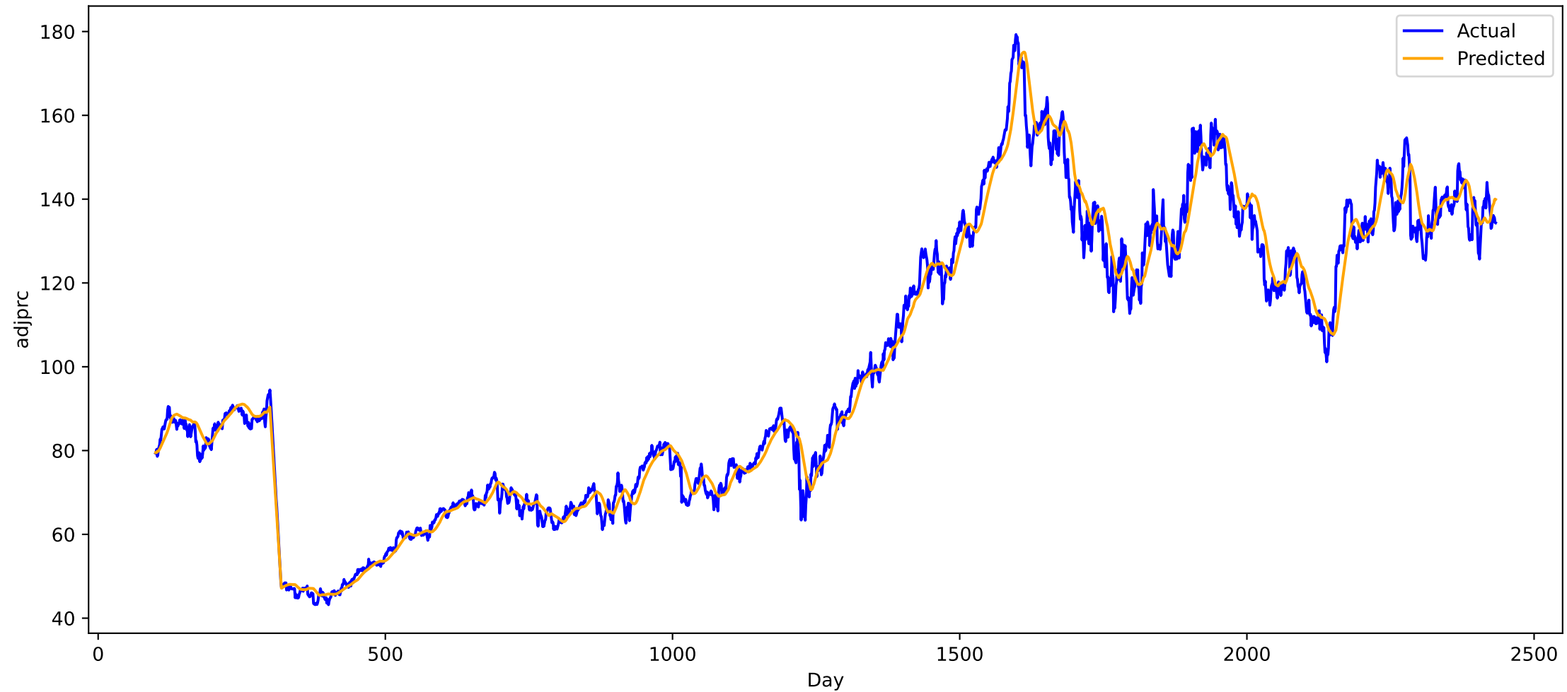
Predicted vs Actual for stock A (all), MAE: 3.3963639736175537
