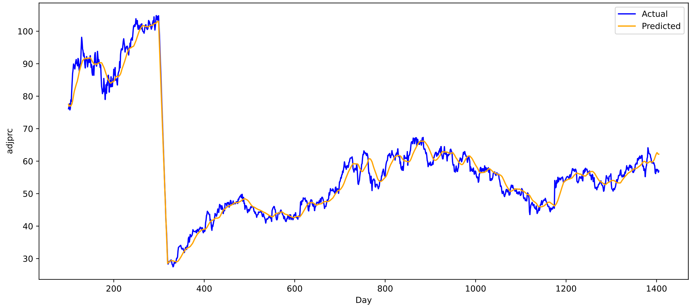
Predicted vs Actual for stock CTVA (all), MAE: 1.9424552917480469
