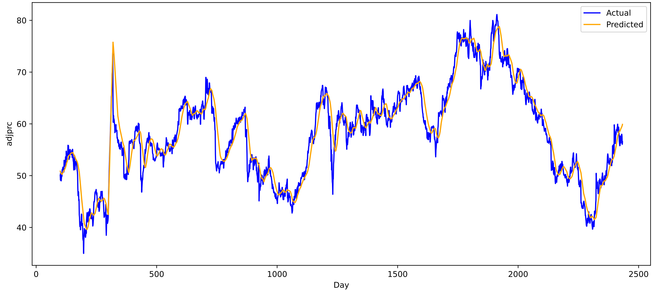
Predicted vs Actual for stock BMY (all), MAE: 1.9077949523925781
