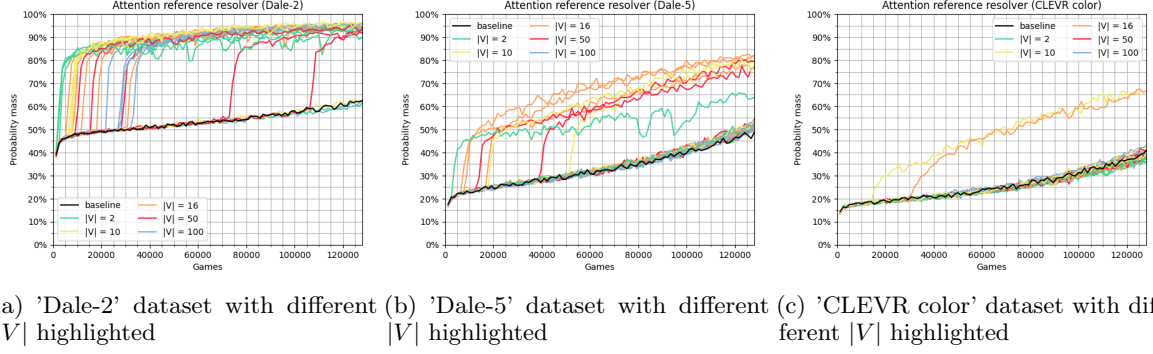
Figure 3: Learning curves of all language games on each dataset. The colors correspond to different vocabulary sizes |V| . The baseline is marked in black.
