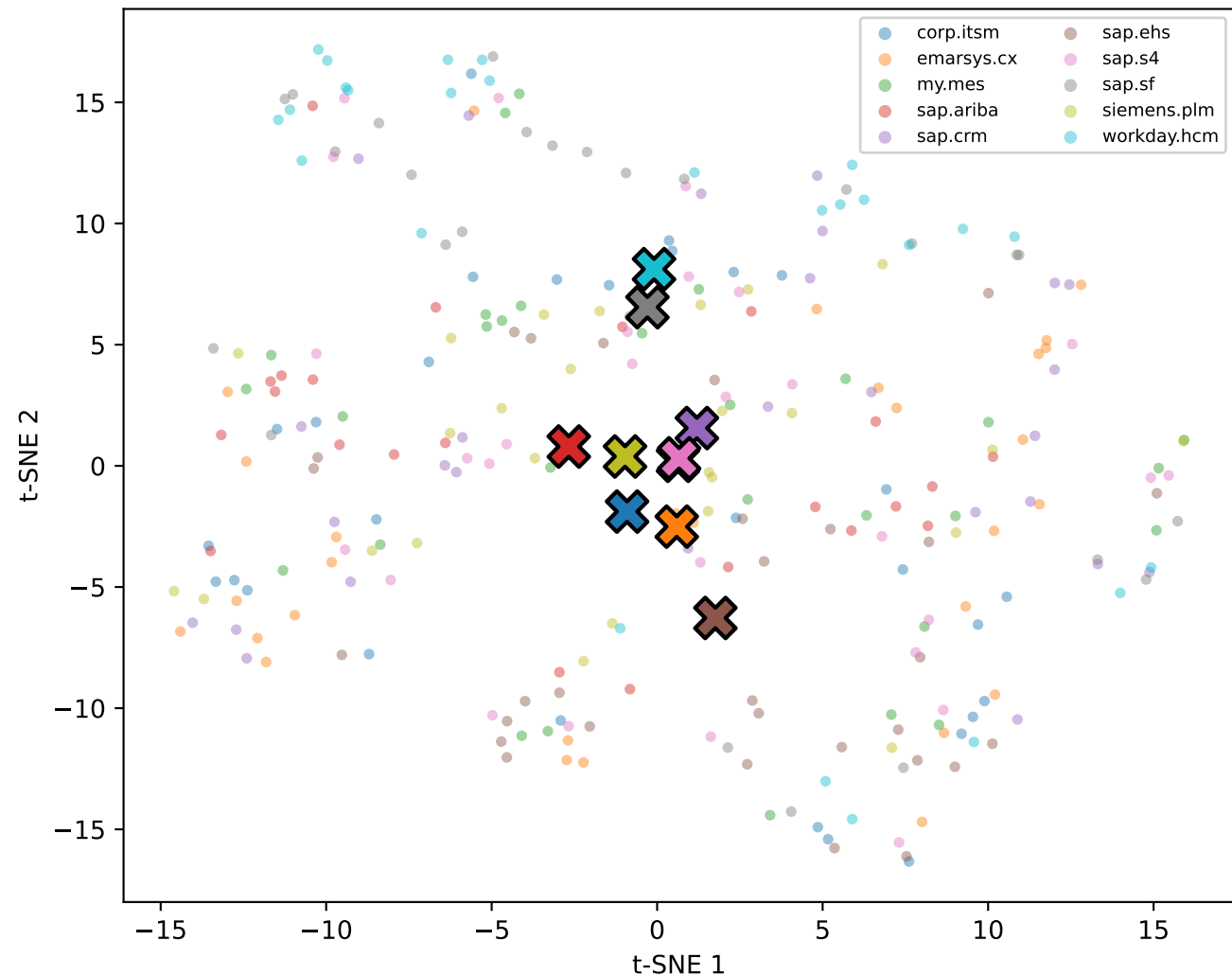
Resources coloured by system (namespace) [enriched] X = system centroid | namespace silhouette = -0.041
