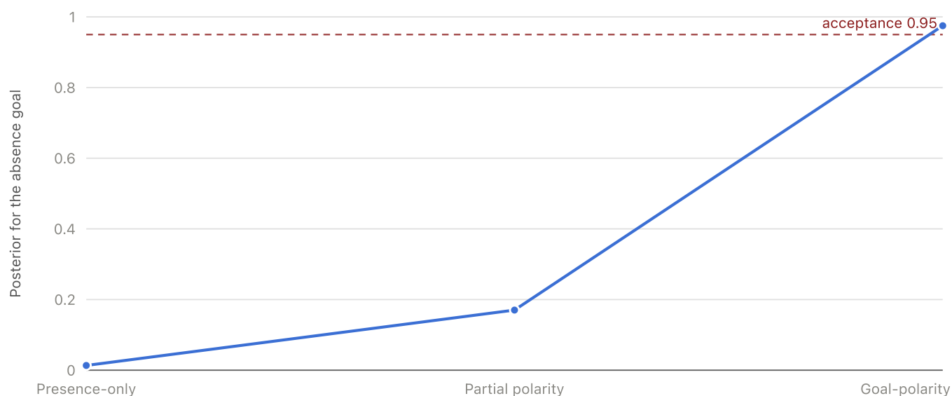
Figure 3. Posterior for the “delete a file that is already absent” goal under three observation-channel conditions. Run-level accuracy on the suite rose from 87.5% (7/8, one false incomplection) to 100% (9/9); false incomplections fell from 1 to 0.
