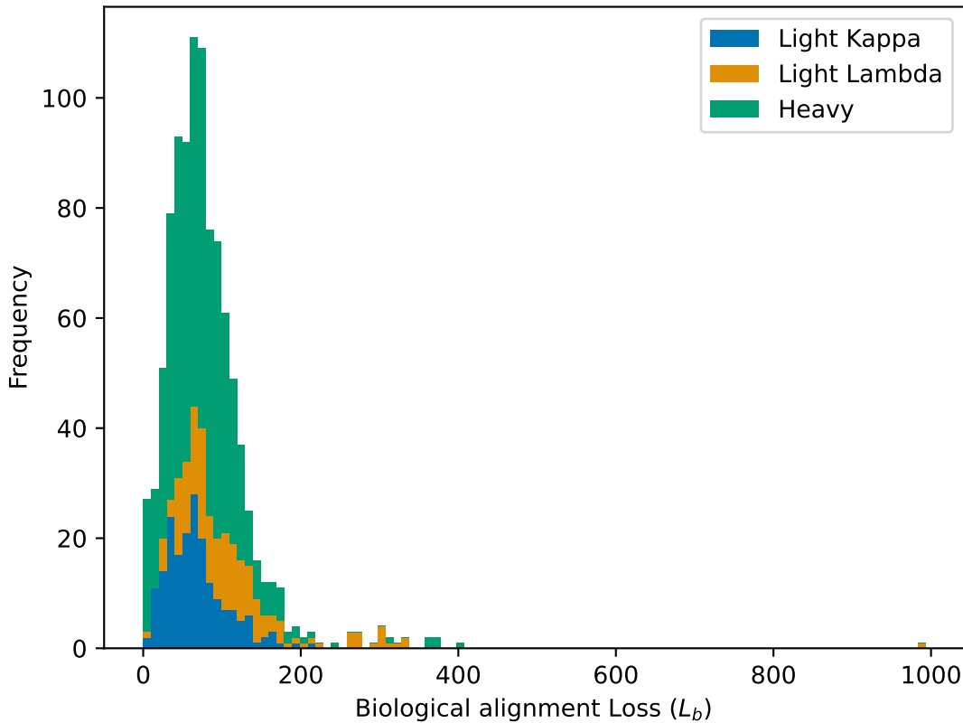
Alignment Score Histogram for Large OAS greedy model
