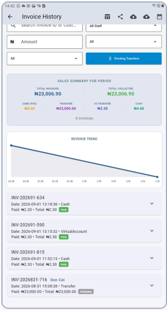
Figure 2: Invoice History & Sales Summary — Multi-criteria search, cashier filters, payment breakdown cards, and expandable invoice audit records.
