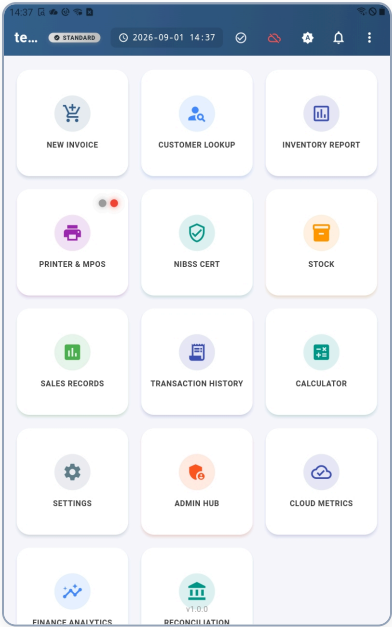
Figure 1: Invify Retail Main Dashboard — 14 operational tiles providing direct access to billing, inventory, hardware, reconciliation, and analytics.
