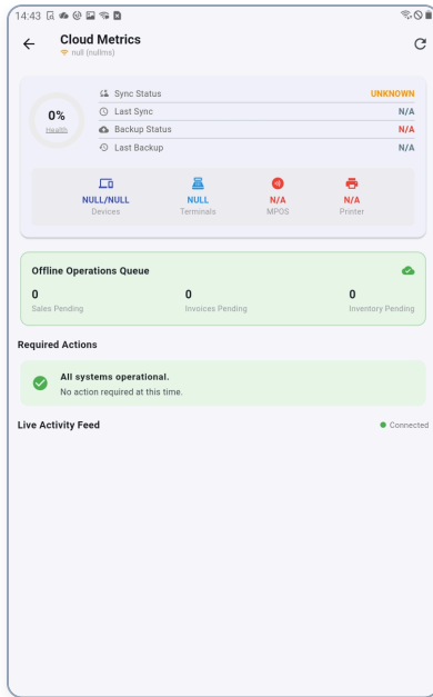
Figure 4: Cloud Metrics Dashboard — Health percentage score, peripheral connections, and offline transaction queue counts.
