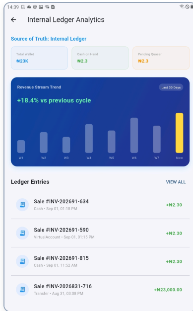
Figure 3: Internal Ledger Analytics — Wallet balances, Cash on Hand, Pending Quasar clearances, and weekly revenue trends.
