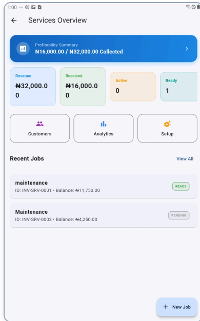
Figure 2: Services Overview — Profitability summary banner, revenue collected vs invoiced, active/ready counts, and recent jobs list with + New Job action.
