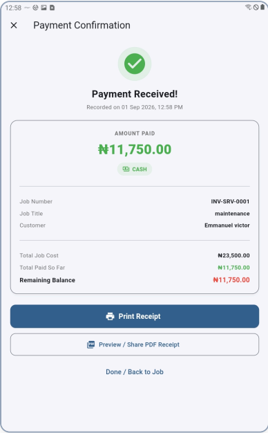
Figure 5: Payment Confirmation Screen — Instant confirmation of partial deposit (₦11,750.00 Cash), remaining balance calculation, and print/share options.
