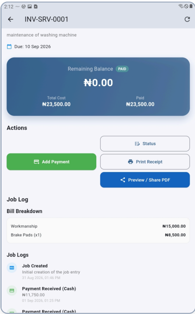
Figure 4: Bill Breakdown & Job Logs — Settled job with Remaining Balance ₦0.00 (PAID), itemized workmanship & parts, and timestamped audit logs.
