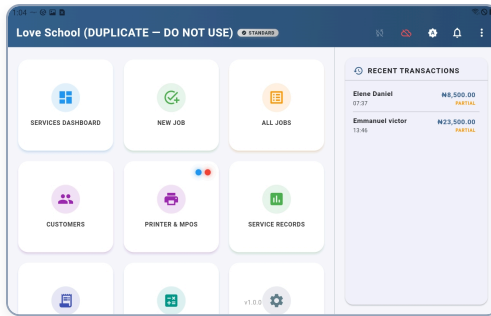
Figure 1: Service Mode Home Dashboard — Core service navigation tiles and sliding Recent Transactions drawer showing active jobs, client names, and partial/paid tags.
