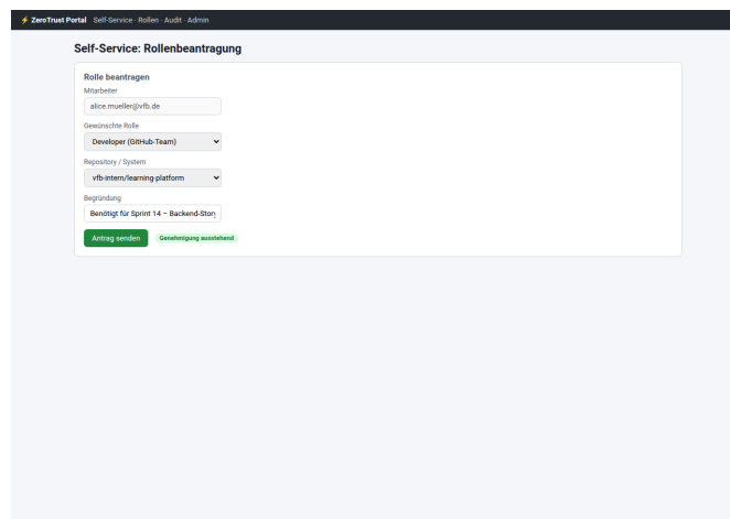
Abbildung 19: Self-Service: Rollenbeantragung
