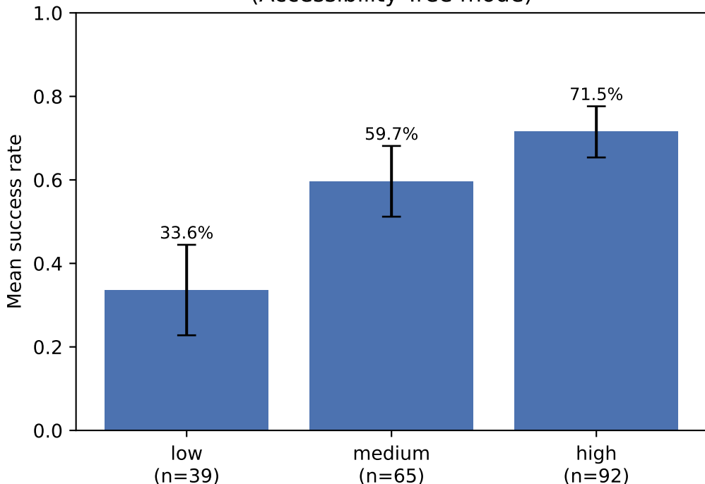
Agent success by WCAG compliance band (Accessibility Tree mode)
