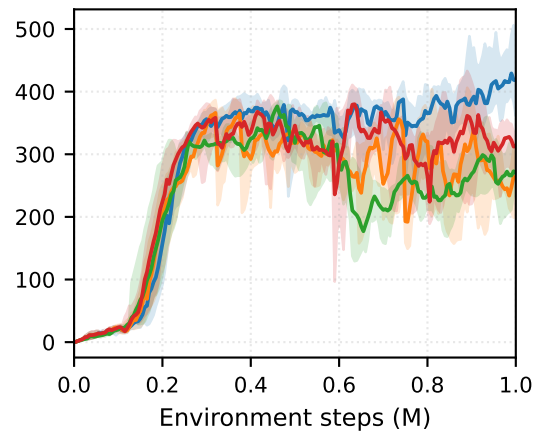
SAC: Walker2d
