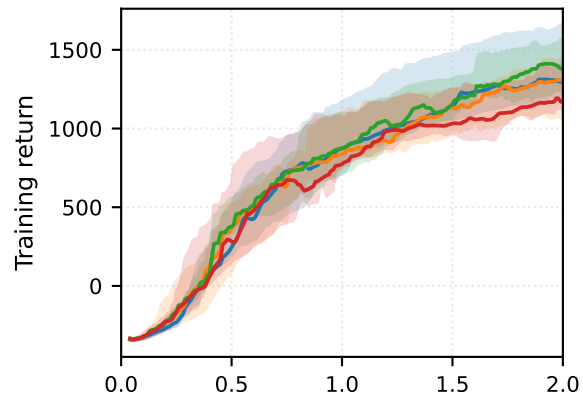
SAC: HalfCheetah
