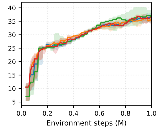
SAC: Swimmer
