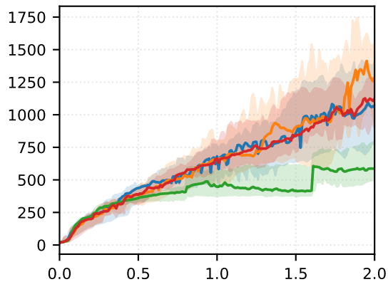
SAC: Hopper
