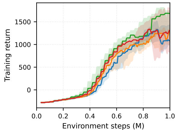
SAC: HalfCheetah
