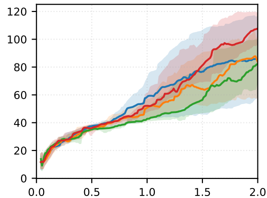
SAC: Swimmer
