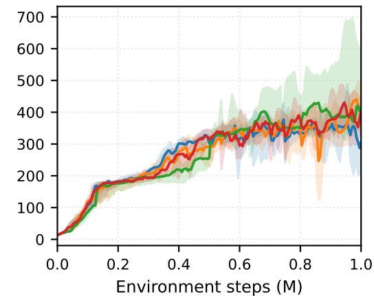
SAC: Hopper
