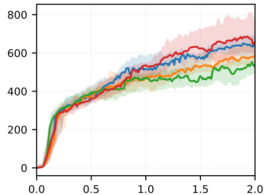
SAC: Walker2d
