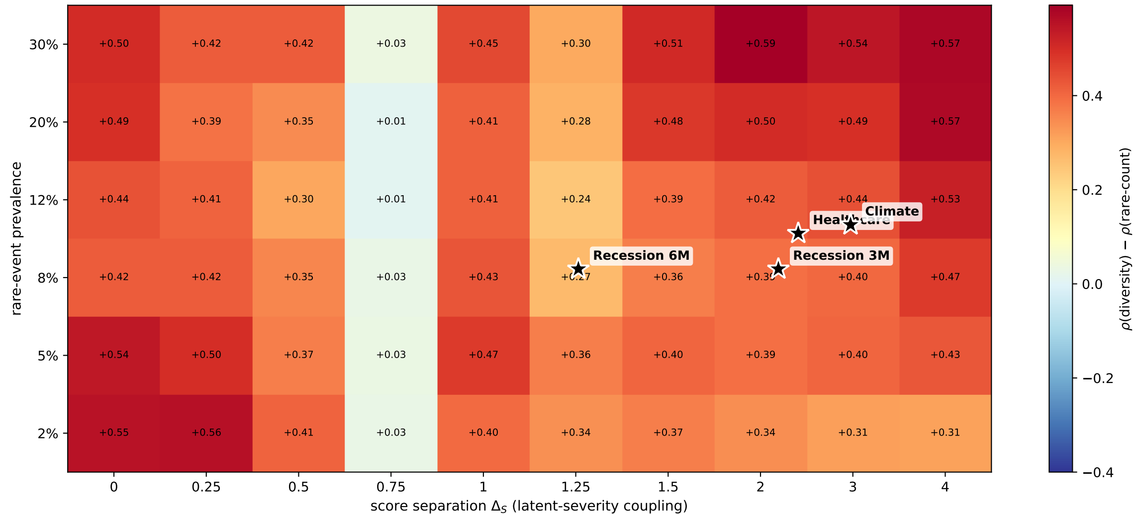
Correlated latent-severity generator (both event probability and score magnitude driven by the same Z_t ; stars = real domains)
