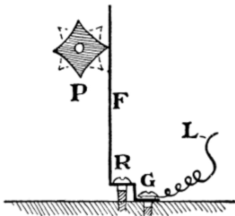
FIG. 19.—The contact-breaker.
