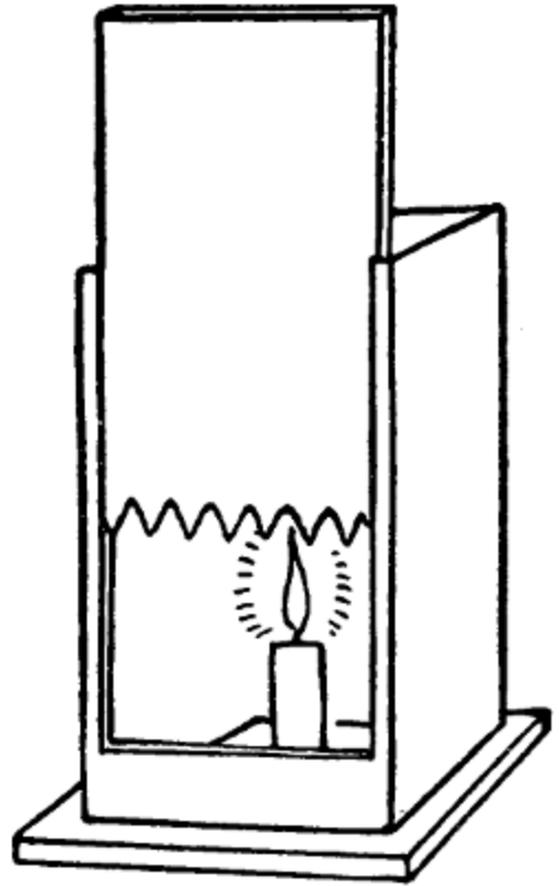
FIG. 5.—Lighting apparatus with serrated shutter.
