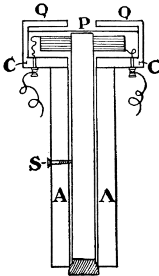
FIG. 3.—Section of completed instrument.
