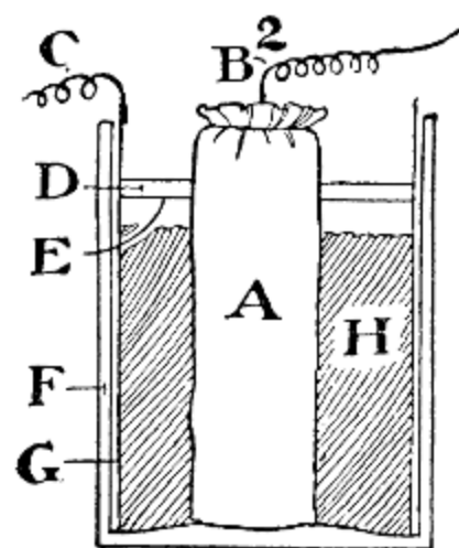
FIG. 4.—Section of the complete cell.
