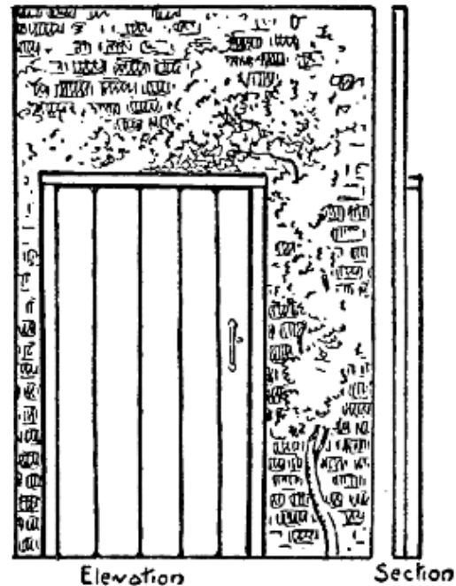
FIG. 8.—Flat 1 or 5 converted into exterior cottage door.
