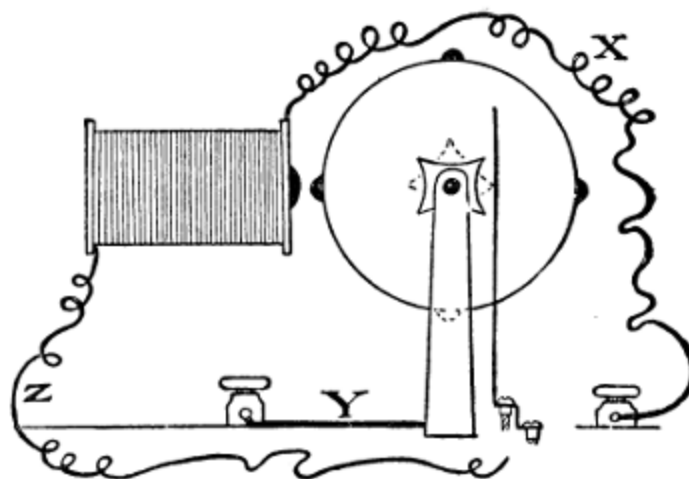
FIG. 20.—Showing wire connections (X, Y, Z) and motor.
