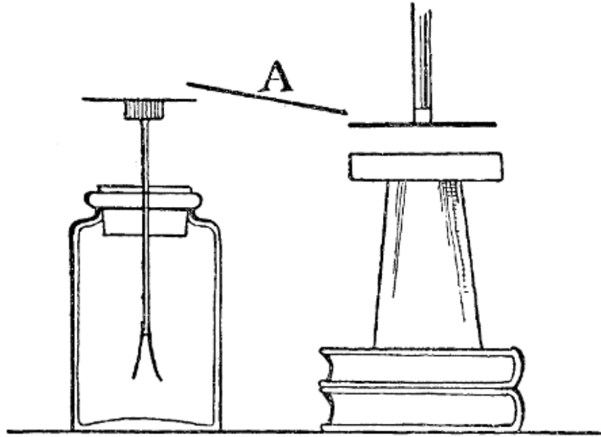
FIG. 10.—An experiment with the electrophorus and electroscope.
