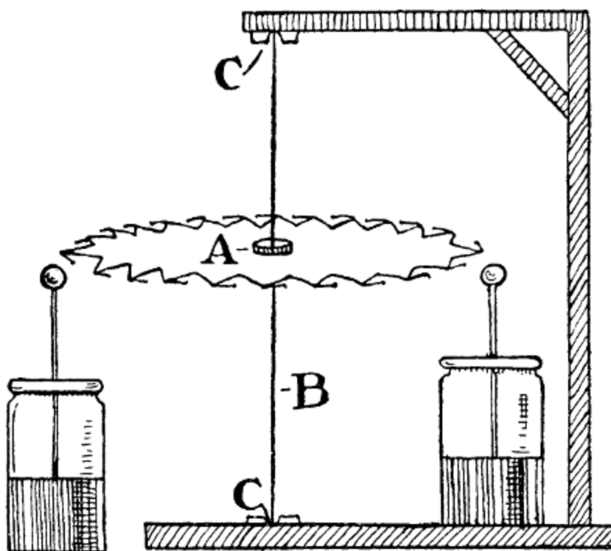
FIG. 12.—Electrostatic motor.
