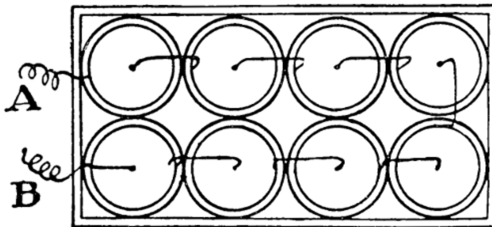
FIG. 6.—The complete battery.
