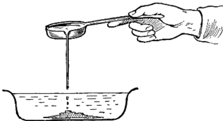
FIG. 3.—Granulating zinc.
