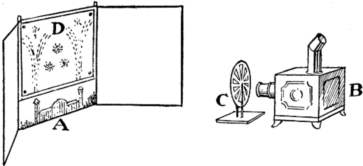
FIG. 4.—Firework apparatus complete.
