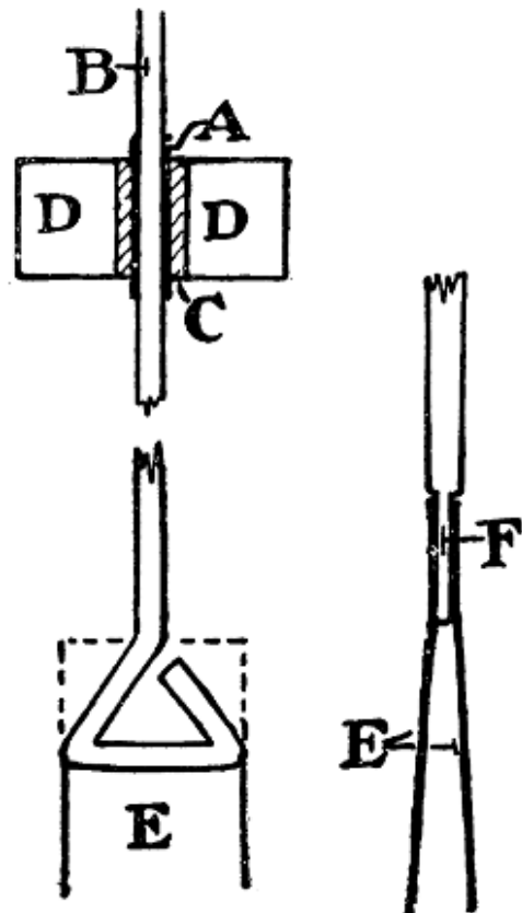
FIG. 5.—Electroscope parts.
