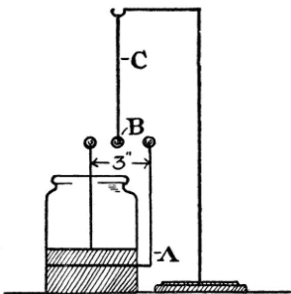
FIG. 8.—Oscillating pith ball.
