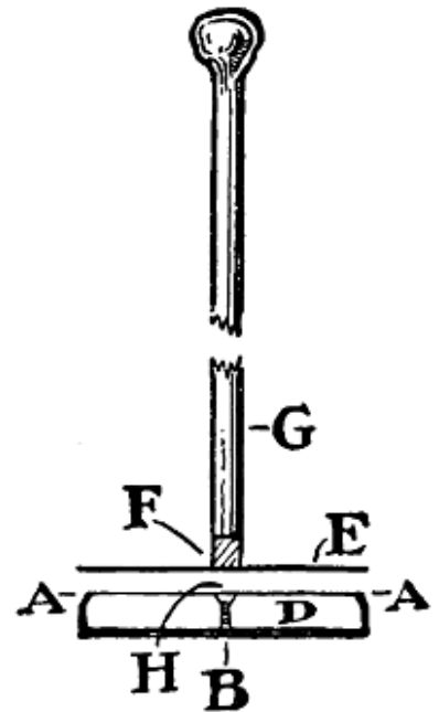
FIG. 6.—The electrophorus.
