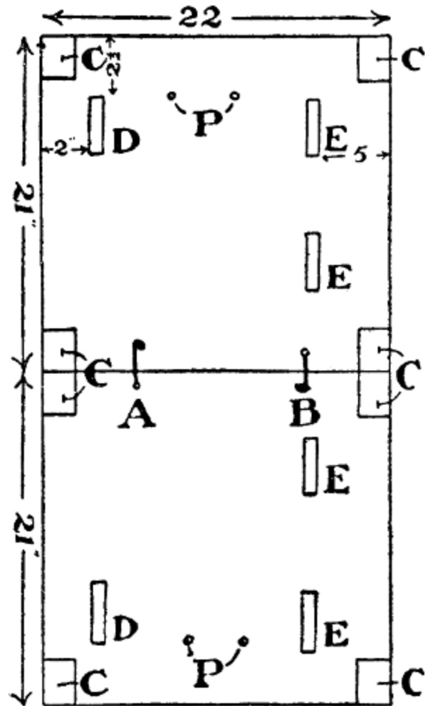
FIG. 1.—Plan of Marionette stage.
