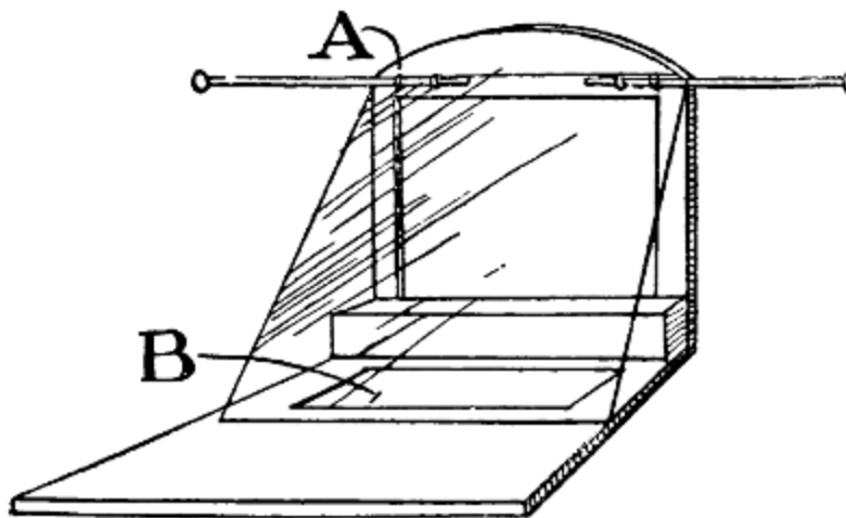
FIG. 3.—Back view of partially constructed apparatus.
