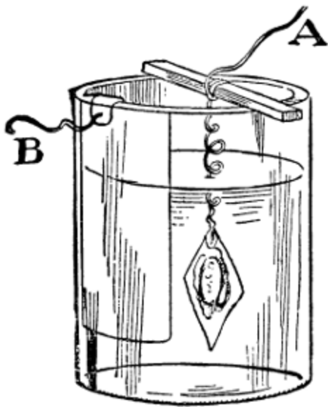
FIG. 25.—Preparation for experiment in electrotyping.
