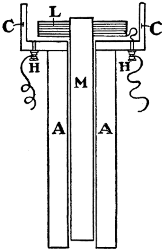
FIG. 2.—Arrangement of magnet.
