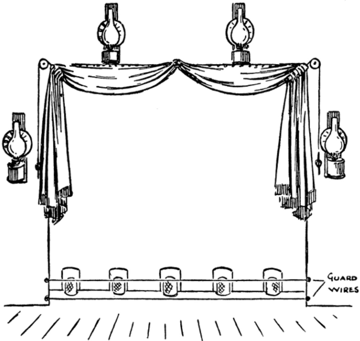
FIG. 1.—Lighting arrangement for back of frame.
