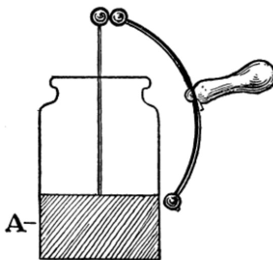
FIG. 9.—Sparks from discharger and Leyden jar.
