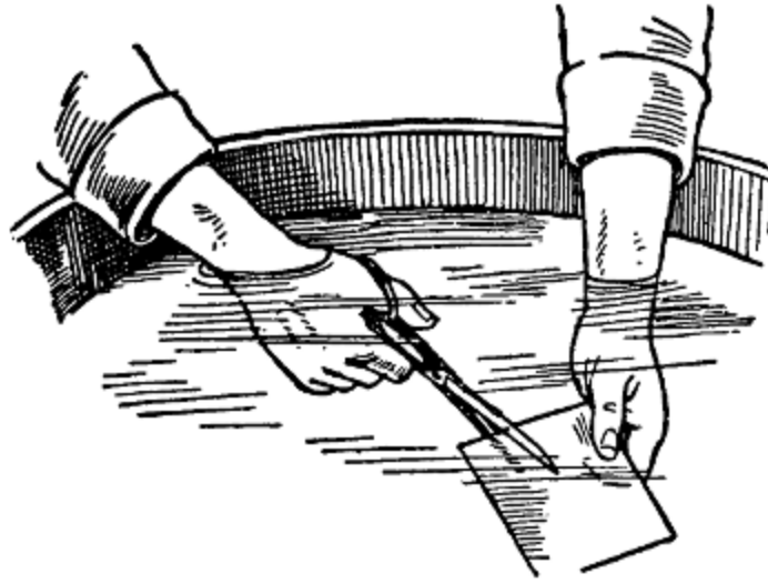
FIG. 17.—A glass-cutting experiment.
