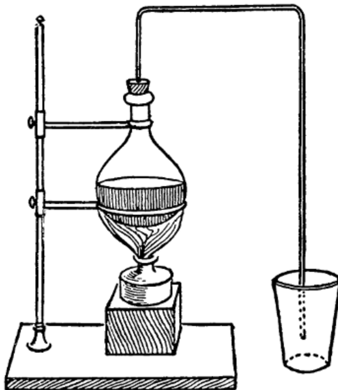
FIG. 15.—A carbonic acid gas experiment.
