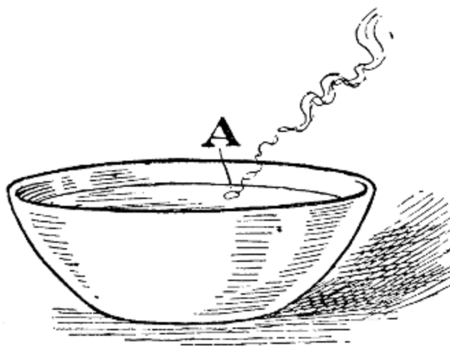
FIG. 7.—A sodium or potassium experiment.
