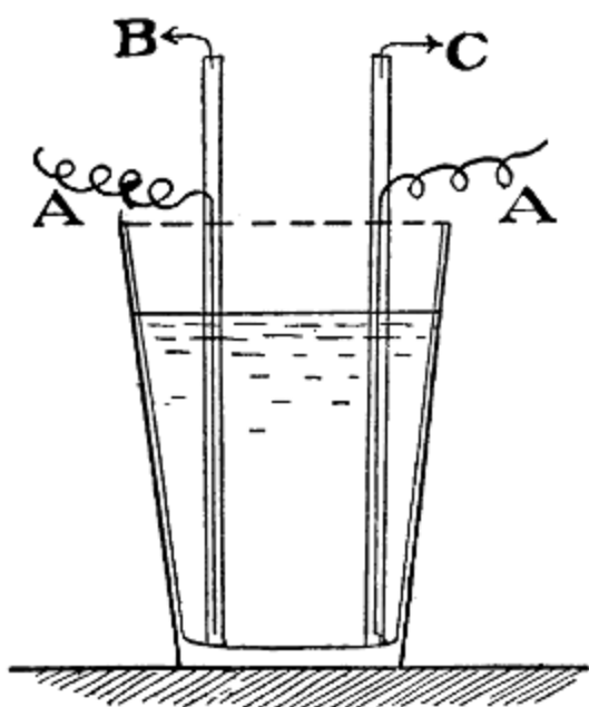
FIG. 23.—The hydrogen bubbles may be ignited by holding a match near the free end of the hydrogen tube.
