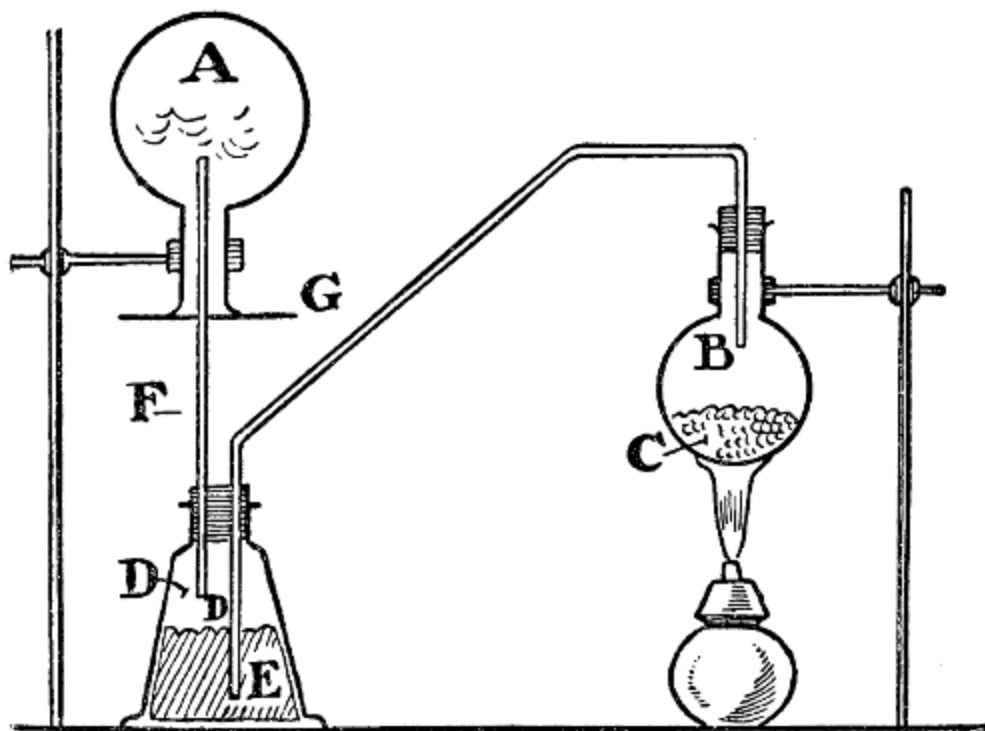
FIG. 12.—To prove water's affection for ammonia.
