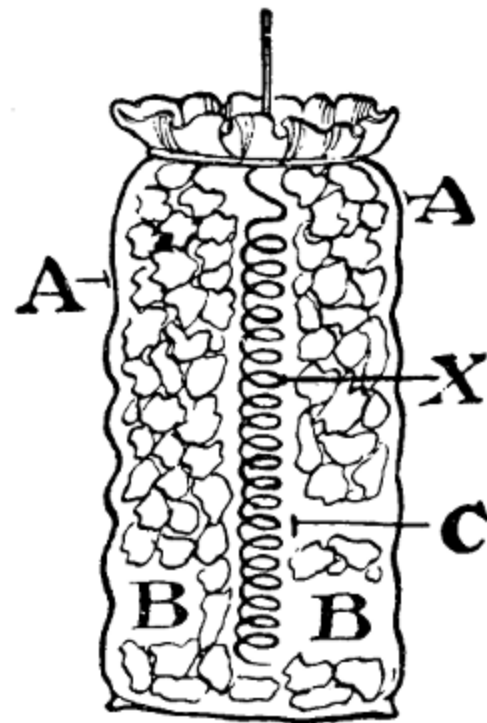
FIG. 2.—Copper spiral surrounded by broken coke in rag or flannel bag.
