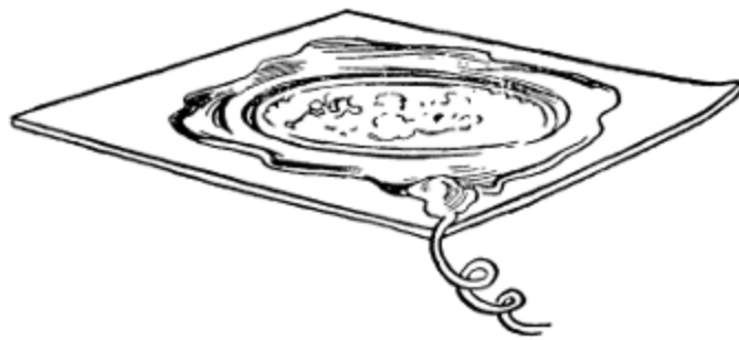
FIG. 26.—Sealing-wax mold suspended in solution of saturated copper sulphate, near to sheet of copper or coil of wire.
