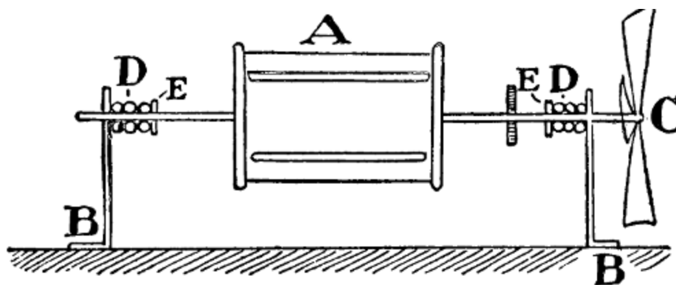
FIG. 17.—An electro-motor.
