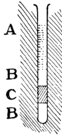
FIG. 4.—Silver solution and precipitate.
