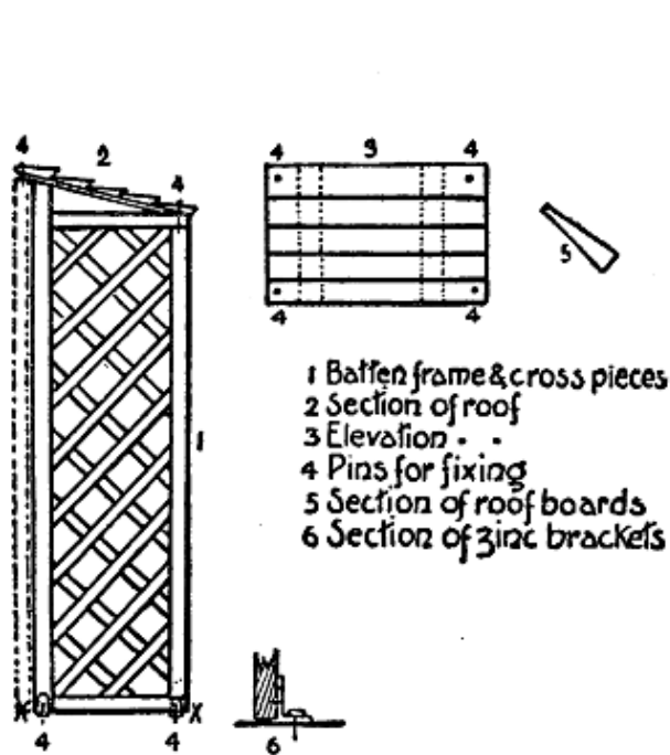
FIG. 9.—Construction of portable porch.
