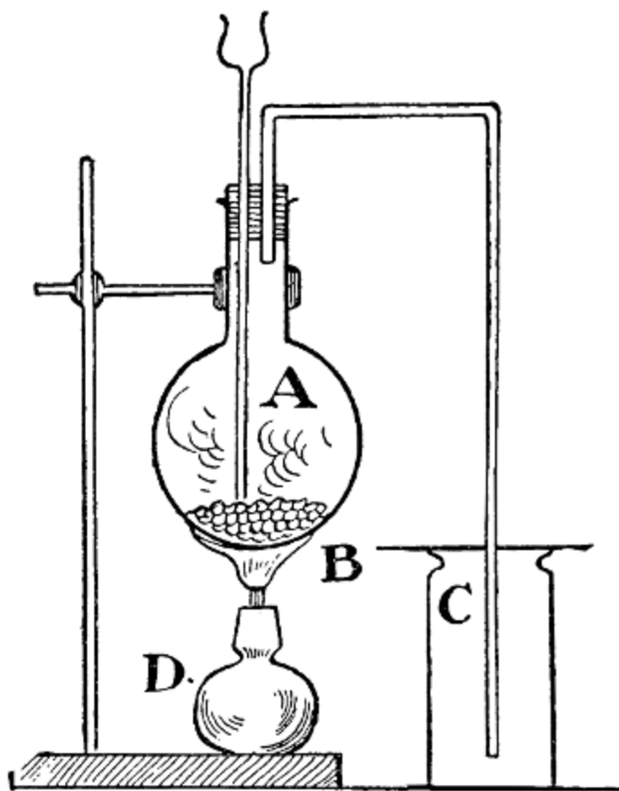
FIG. 1.—Apparatus for chlorine experiments.
