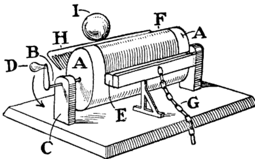
FIG. 13.—Frictional machine (more useful than the electrophorus for producing electric charges).
