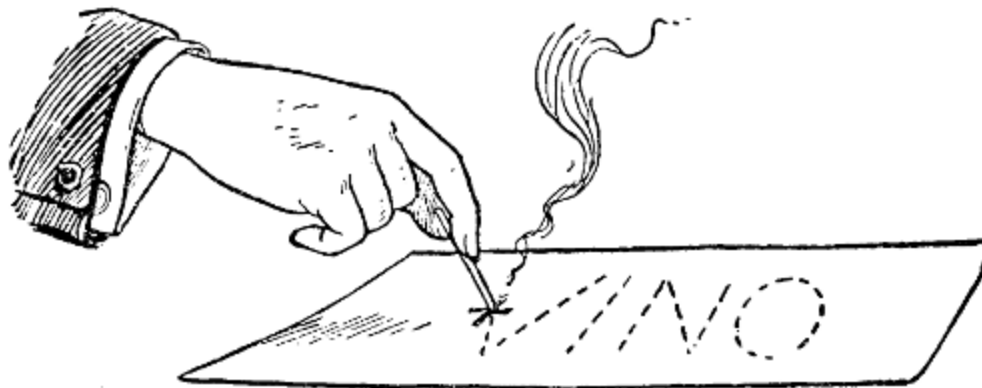
FIG. 5.—A niter paper experiment.
