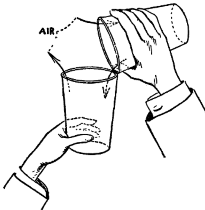
FIG. 16.—Pouring carbon dioxide from one glass to another.
