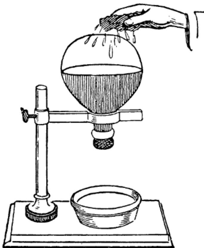
FIG. 13.—A curious boiling experiment.
