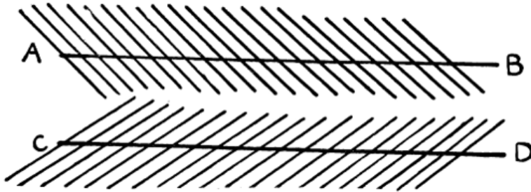
FIG. 6.—Zollner's lines.
