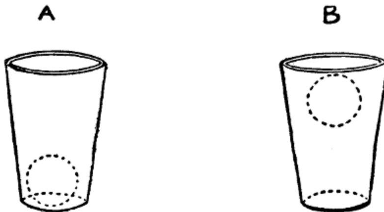
FIG. 17.—Soap bubbles in A (air), and B, carbon dioxide.
