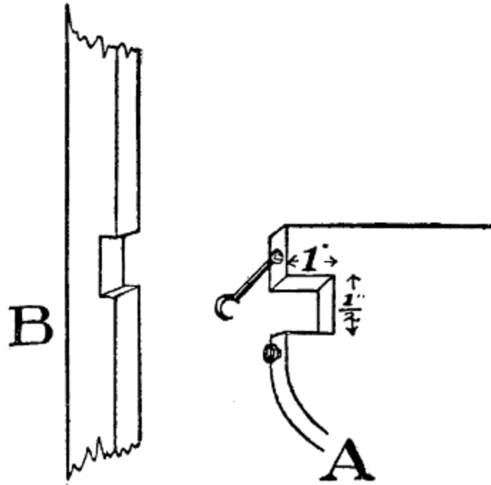
FIG. 4.—Arrangement for supporting platform on frame.
