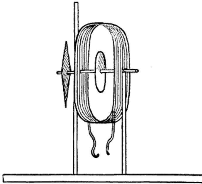
FIG. 3.—Revolving needle in coil.
