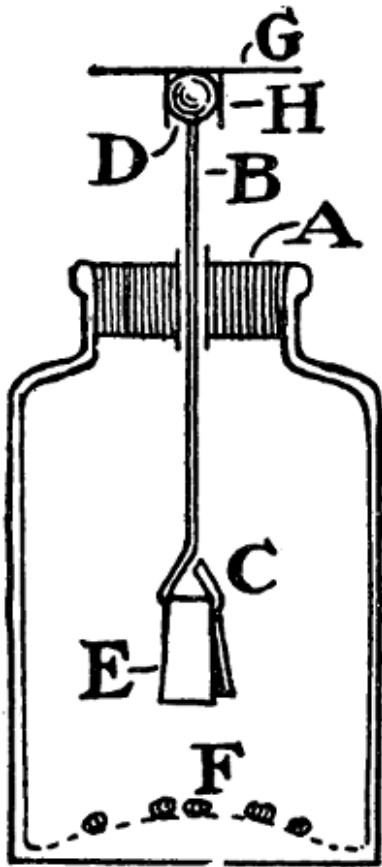
FIG. 4.—The electroscope.
