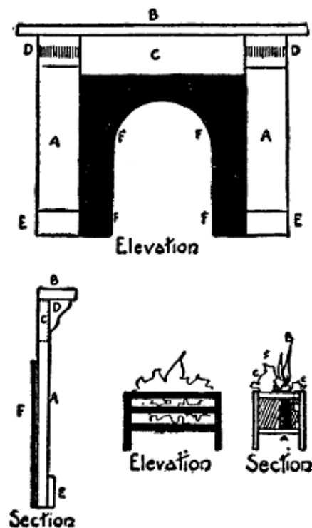
FIG. 10.—Portable fireplace and grate.
