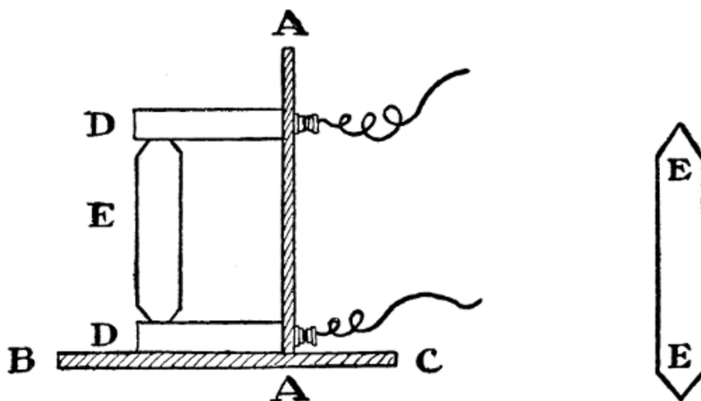
FIG. 5.—Sectional view of microphone.
