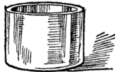
FIG. 16.—Showing smooth break after red-hot poker has been plunged into the oil.
