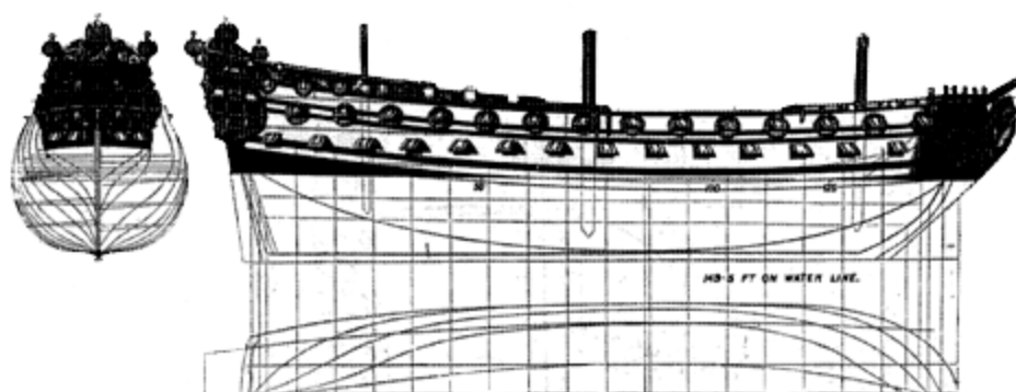
FIG. 52.—British second-rate. 1665.
