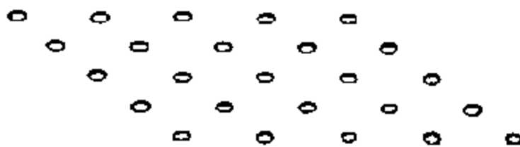
FIG. 14.—Probable arrangement of oar-ports in ancient galleys.
