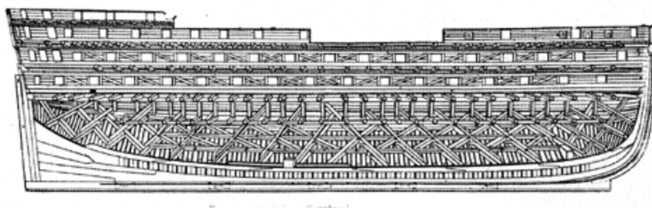
FIG. 62.—Sir Robert Seppings' system of construction.
