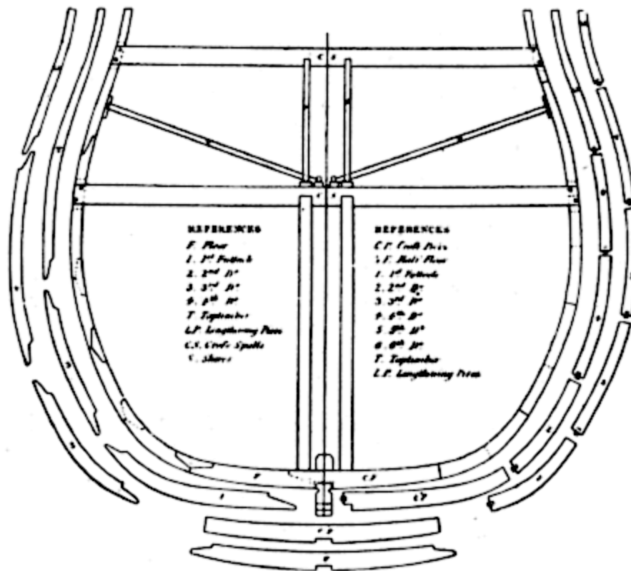
FIG. 64.—Sir Robert Seppings' system of construction.
