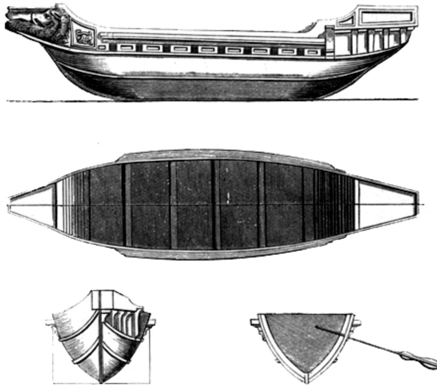
FIG. 13.—Roman merchant-ship.
