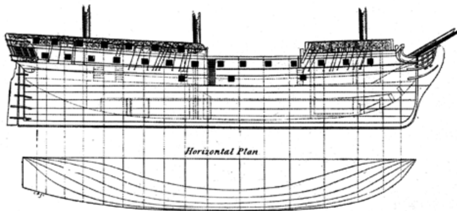
FIG. 59.—Heavy French frigate of 1780.
