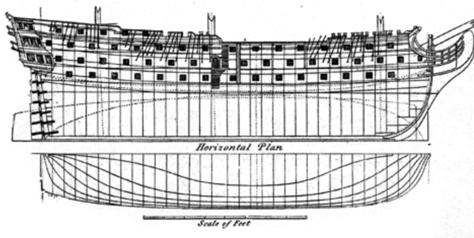
FIG. 57.—British first-rate. 1794.
