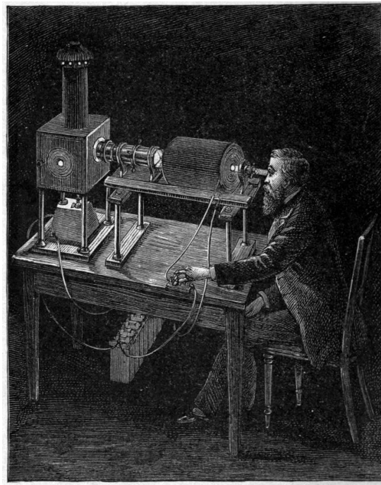
MAGNETISM, LIGHT, AND MOLECULAR SPINNING TOPS.
