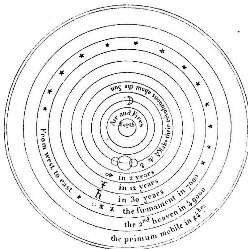
FIG. 19.—CAPELLA'S SYSTEM.
