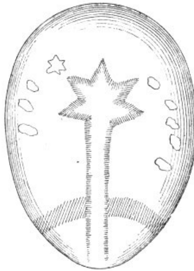
FIG. 56.—AN EGG MARKED WITH A COMET.
