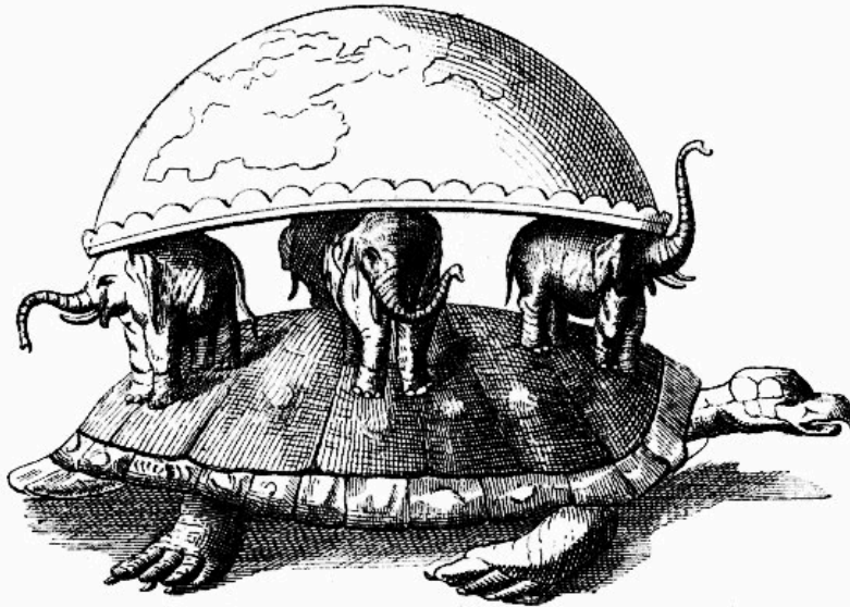
FIG. 28.—HINDOO EARTH.
