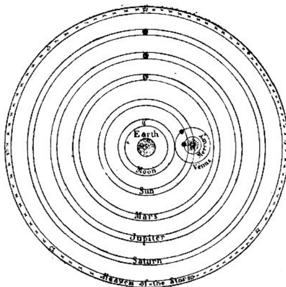
FIG. 18.—EGYPTIAN SYSTEM.
