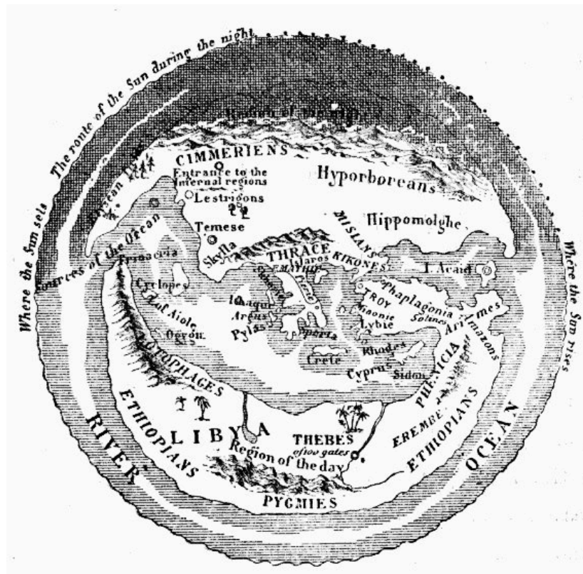
FIG. 32.—HOMERIC COSMOGRAPHY.
