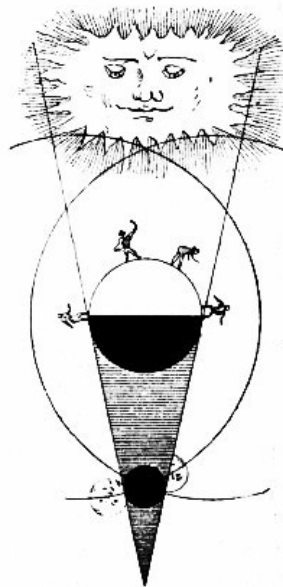
FIG. 35.—THE EARTH'S SHADOW.
