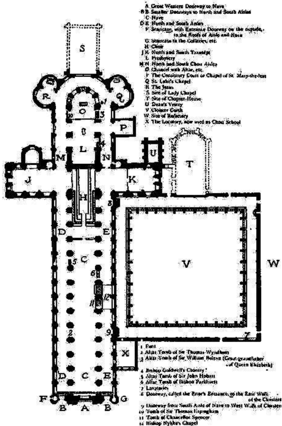
PLAN OF NORWICH CATHEDRAL
