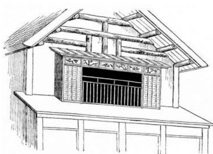
Fig. 42.—Bay Window, Village of Odzuka, Rikuzen.
