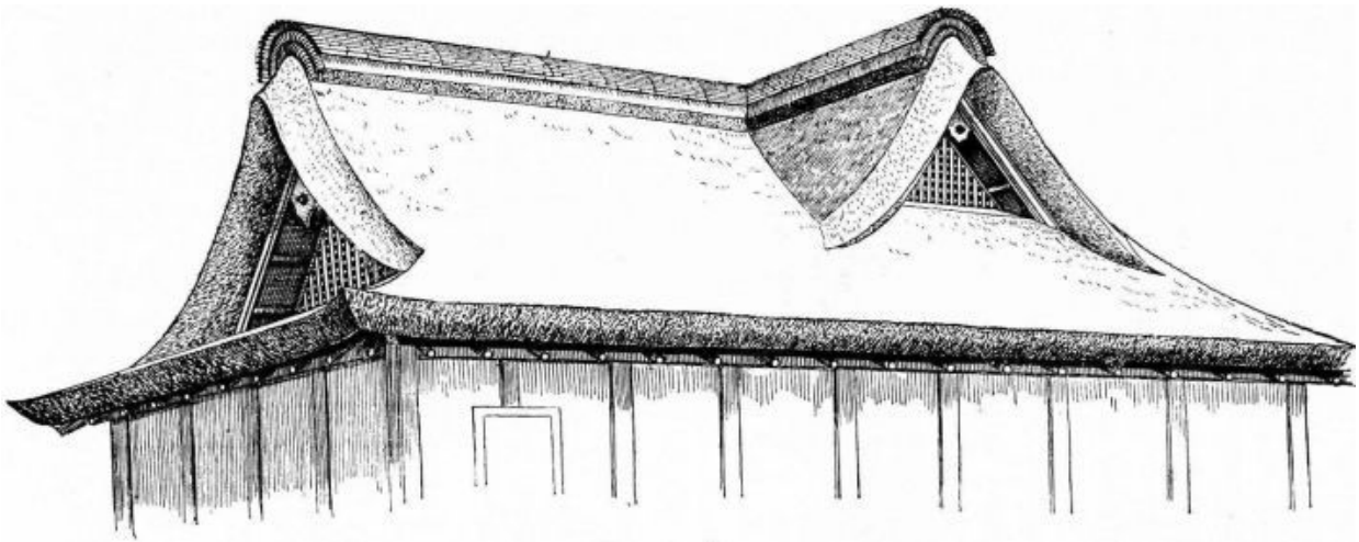
Fig. 83.—Thatched Roof, near Tokio. 10
