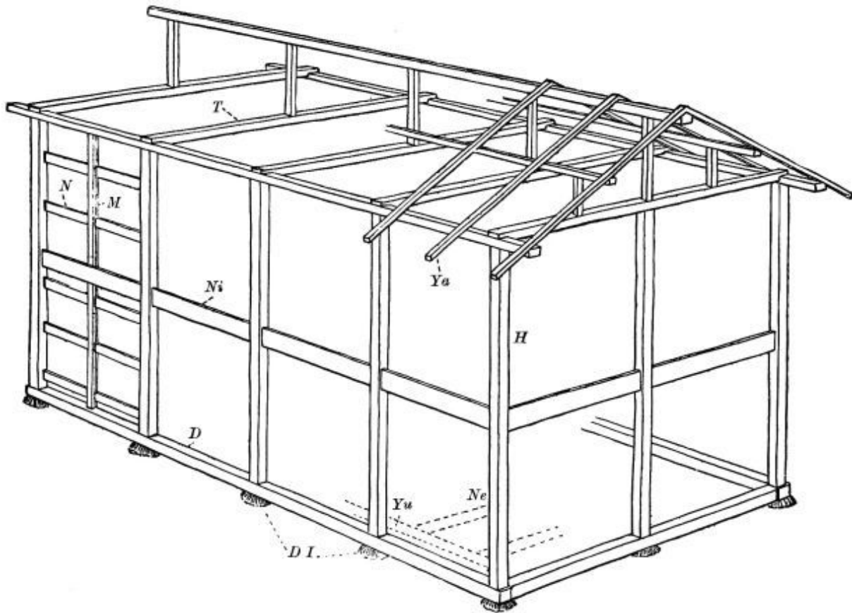
Fig. 12.—Framing of an Ordinary Two-stored House.
