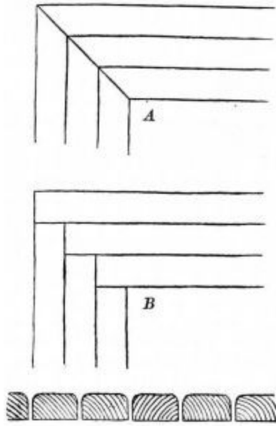
Fig. 226.—Verandah floor.
