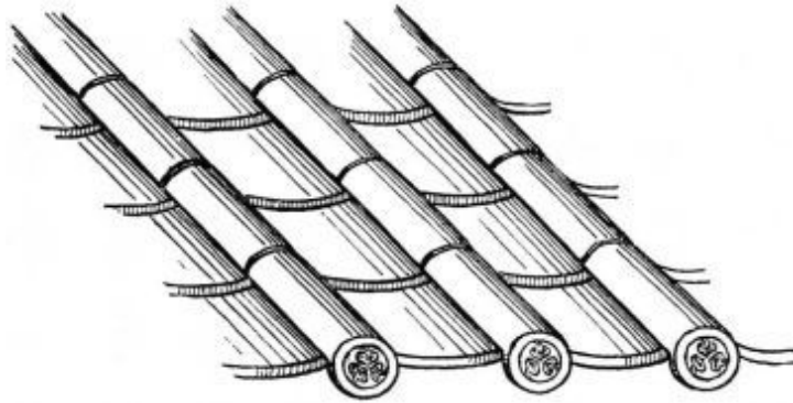
Fig. 73.—Hon-gawara, or True Tile.
