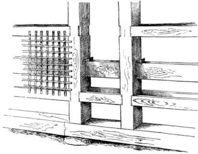
Fig. 4.—Side Framing.
