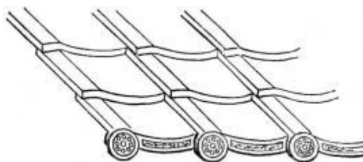
Fig. 71.—Eaves of tiled roof.
