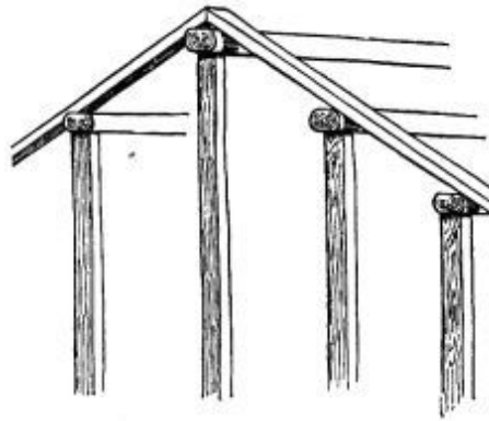
Fig. 8.—Framing.
