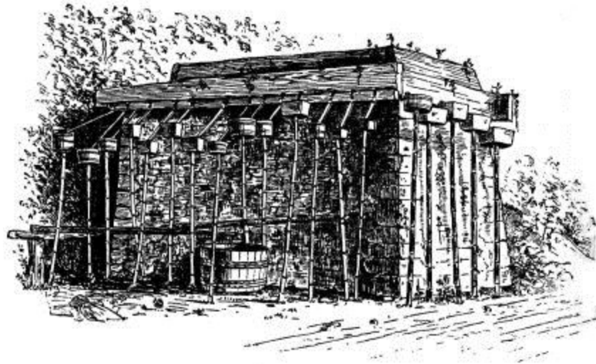
Fig. 291.—Aqueduct reservoir at Miyajima, Aki.
