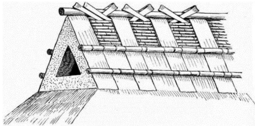
Fig. 93.—Crest of thatched roof in Kii.
