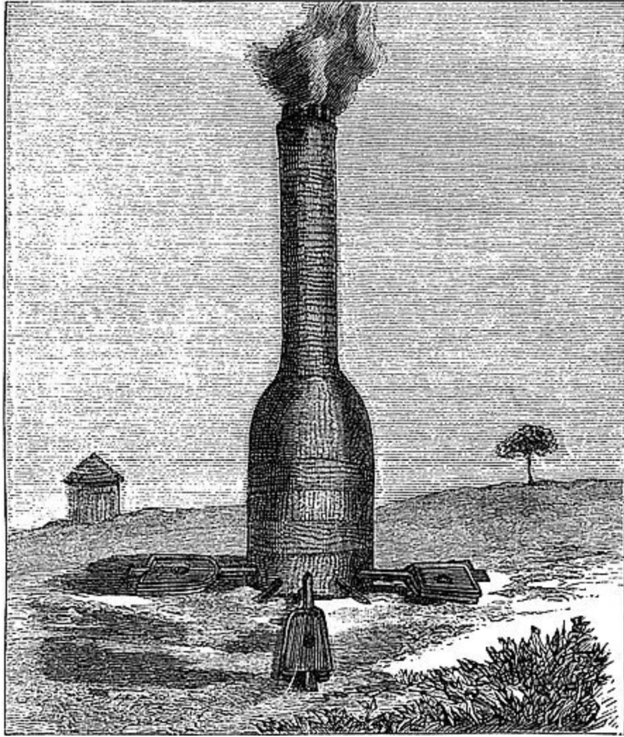
FIG. 104.—IRON SMELTING FURNACE AMONGST THE MARÁVE PEOPLE.
