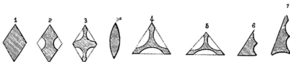
FIG. 124.—SECTIONS OF THRUSTING-SWORDS.
