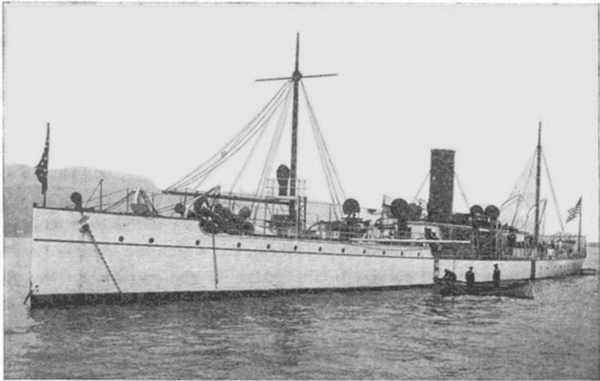
DYNAMITE CRUISER "VESUVIUS."
