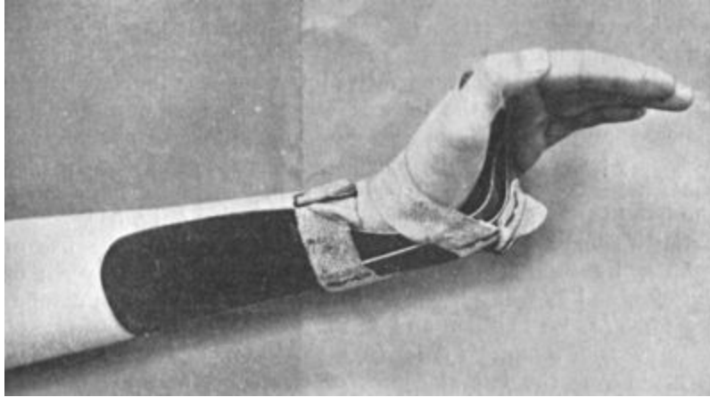
FIG. 31.—“Cock-up” Splint, for maintaining Dorsiflexion at Wrist.
