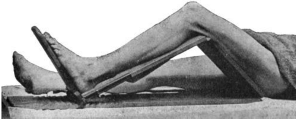
FIG. 70.—Adjustable Double-inclined Plane.
