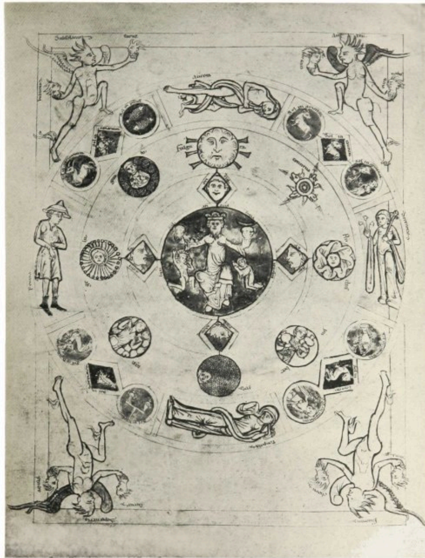
PLATE IV. THE UNIVERSE
