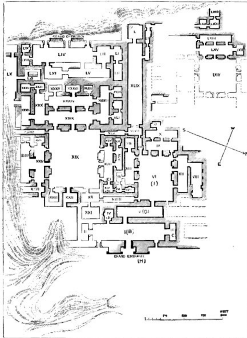
FIG. 63.—Layard's plan of the Palace of Sennacherib discovered in the mound of Kouyunjik. The temple axis, XXXVI., XXXIV., XXIX., XIX. (XXII. is on a lower level), faces the rising of the May sun.
