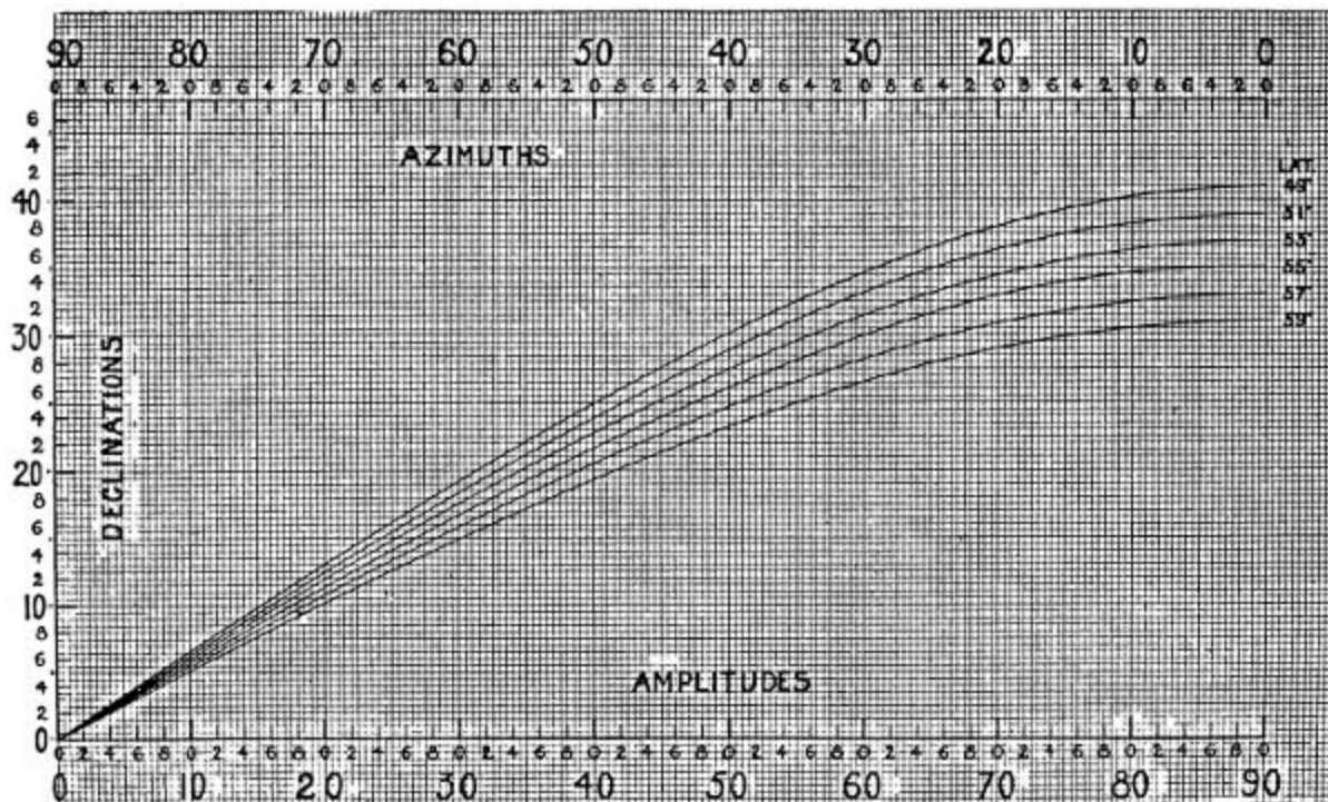
FIG. 33.—Diagram for finding declination from given amplitudes or azimuths in British latitudes.
