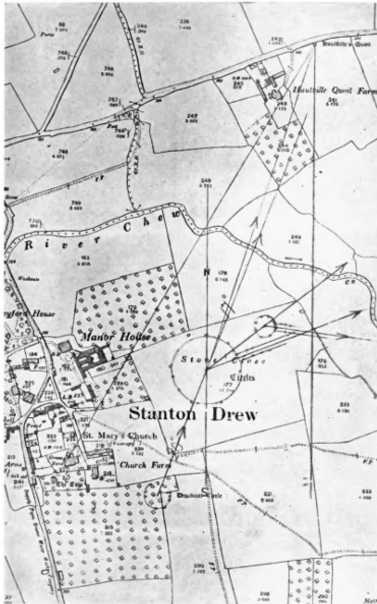
FIG. 47.—The Circles and Avenues at Stanton Drew. Photograph of 25-inch Ordnance map, shewing approximate azimuths of sight-lines.
