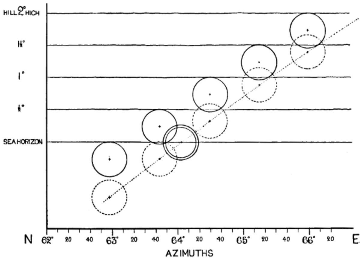
FIG. 51.—Showing the influence of the height of the sky-line on the apparent place of sunrise in May and August. The double circle shows the tabular place of sun's centre.
