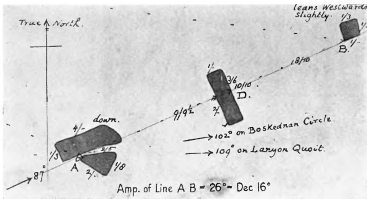
FIG. 56.—Plan of the Mên-an-tol from Lukis, showing that it was an apparatus for observing the sunrise in May and August in one direction and the sunset in February and November in the other. Sun's declination, 16^{\circ} N. or S.
