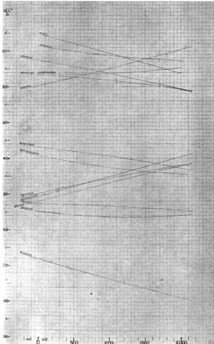
FIG. 35.—Declinations of Southern Stars from 250 A.D. to 2150 B.C.
