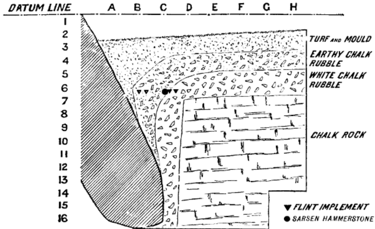
FIG. 21.—Face of rock against which a stone was made to rest.
