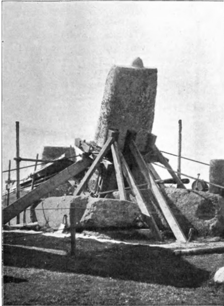
FIG. 17.—The cradle and supports, looking west.
