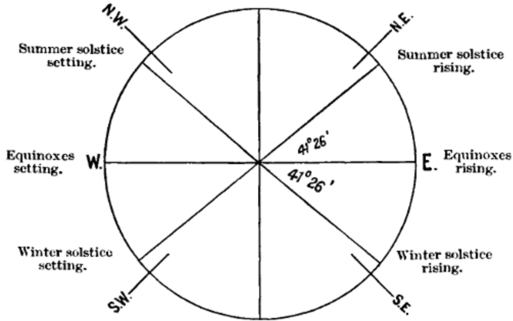
FIG. 6.—The various bearings of the sun risings and settings in a place with a N. latitude of 51^{\circ} .
