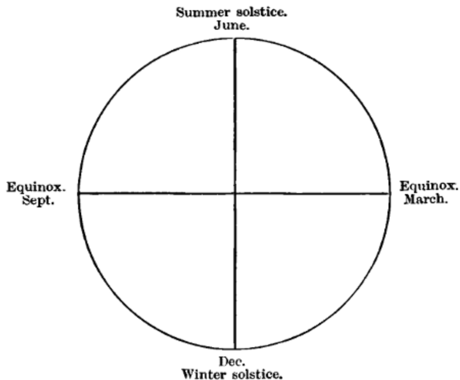
FIG. 5.—The four Astronomical Divisions of the year.
