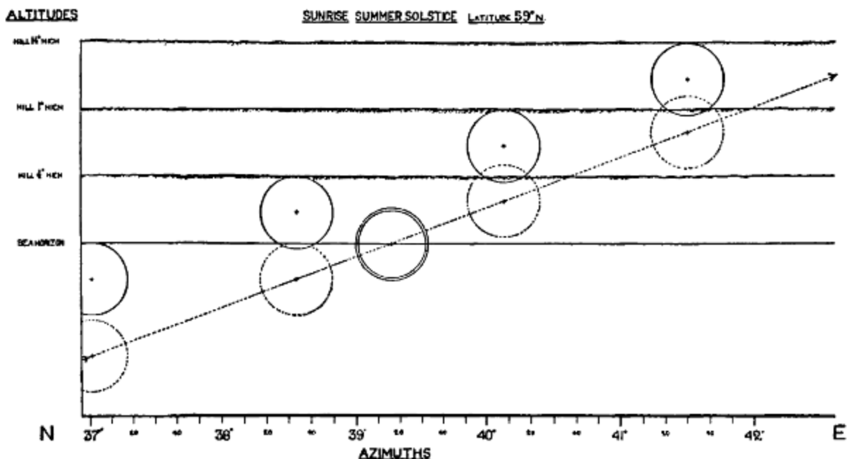
FIG. 36.—The Conditions of “Sunrise” at the Summer Solstice in Lat. 59° N.
