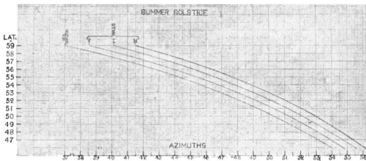
FIG. 37.—The Azimuths of the Sunrise (upper limb) at the Summer Solstice.
