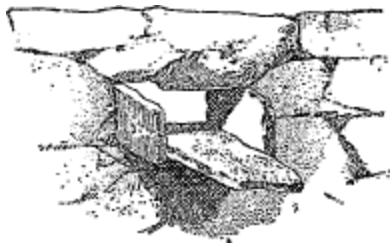
FIG. 40. Trough roof drains of stone.
