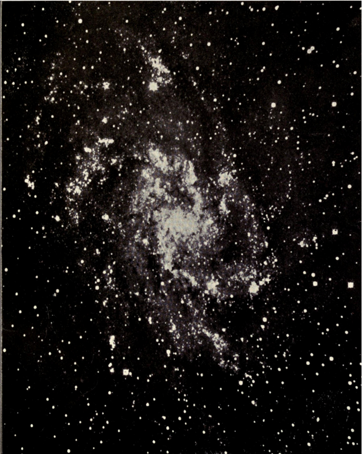
Wonderful spiral in triangulum
