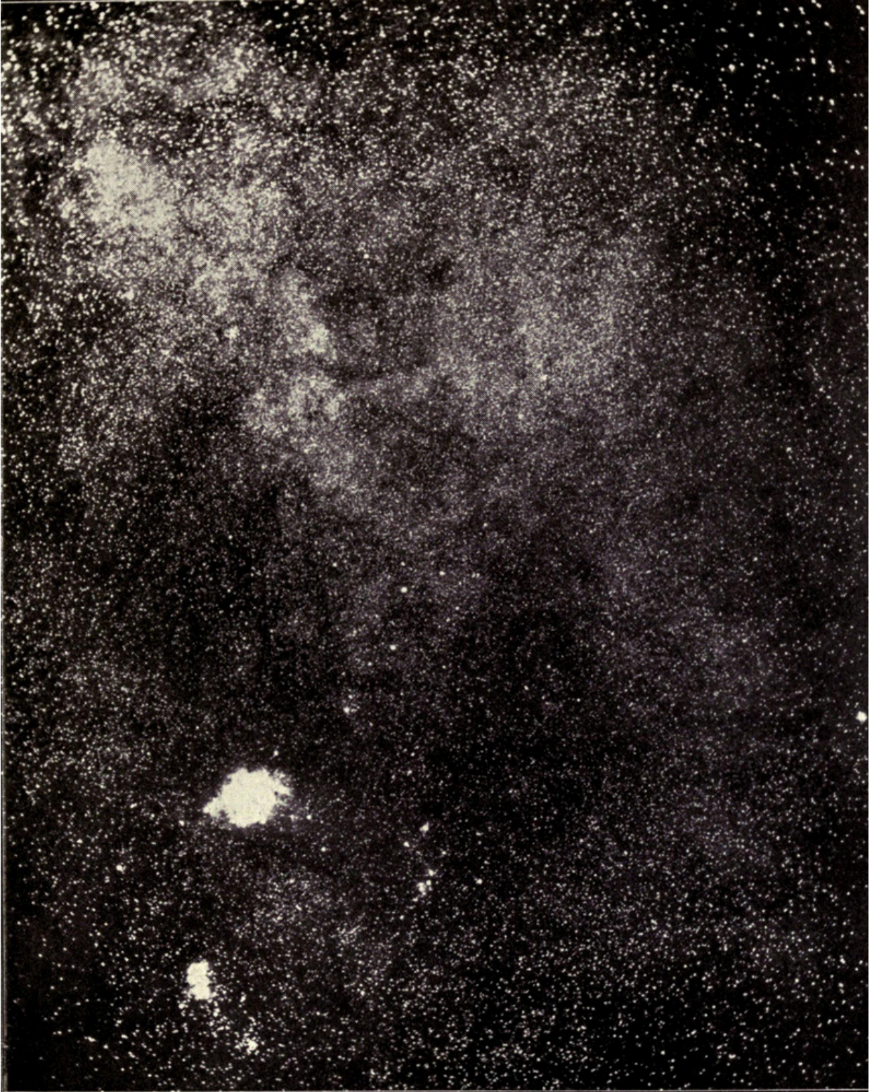
The Milky Way. Region near M.S. Photographed by Professor Barnard
