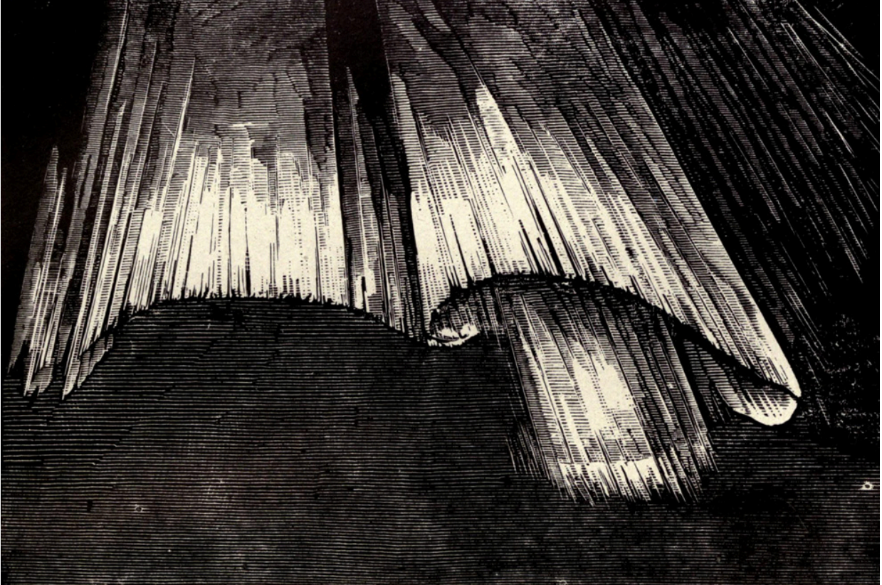
Auroral curtain seen in Scandinavia
