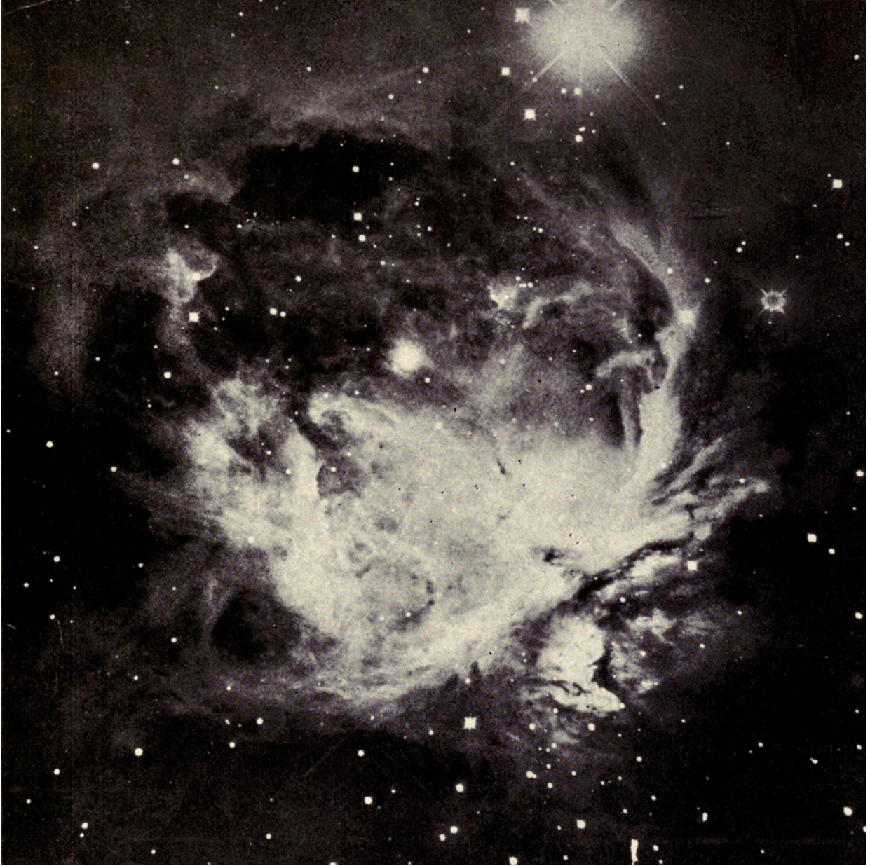
The Orion nebula
