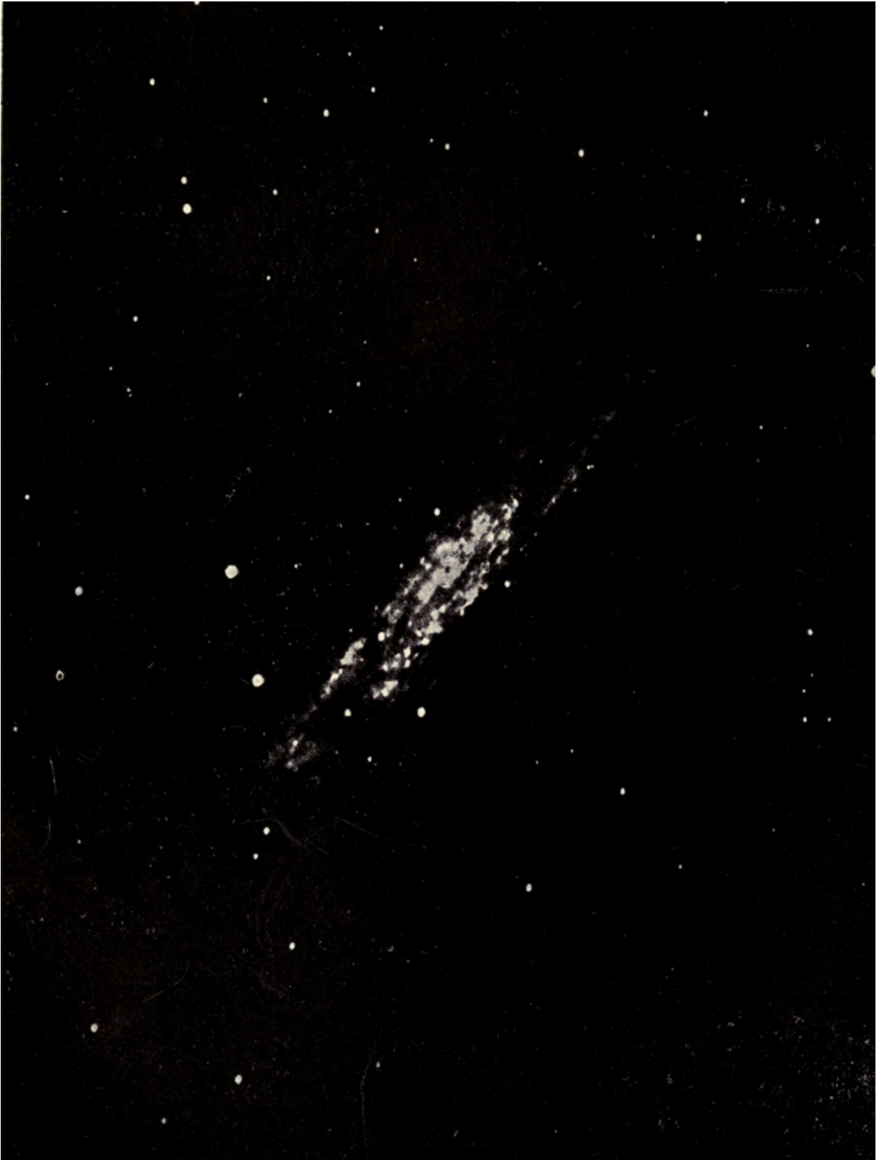
Nebula in Cetus
