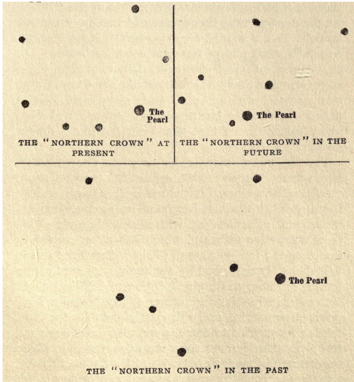
The “Northern Crown”
