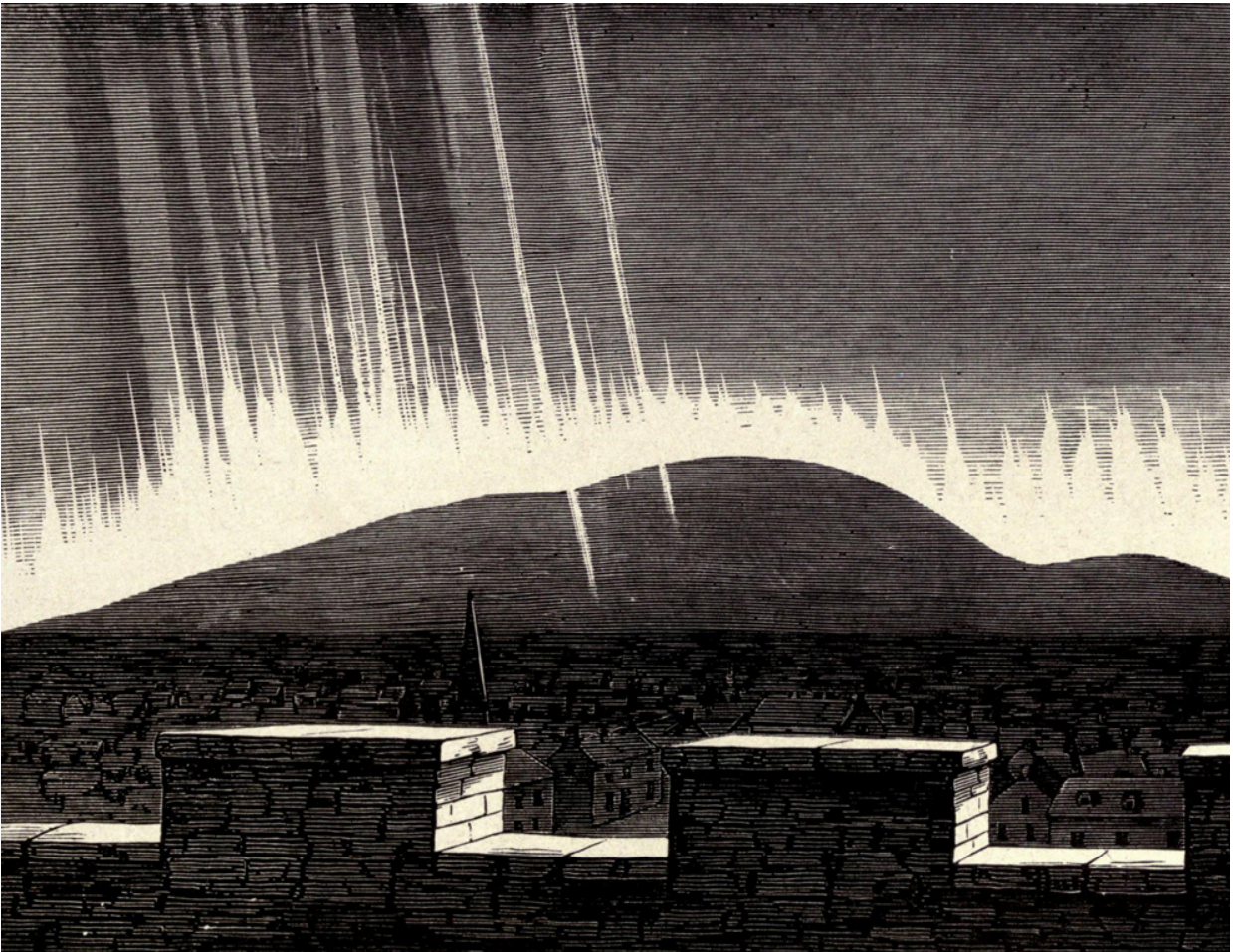
Auroral beams seen in England
