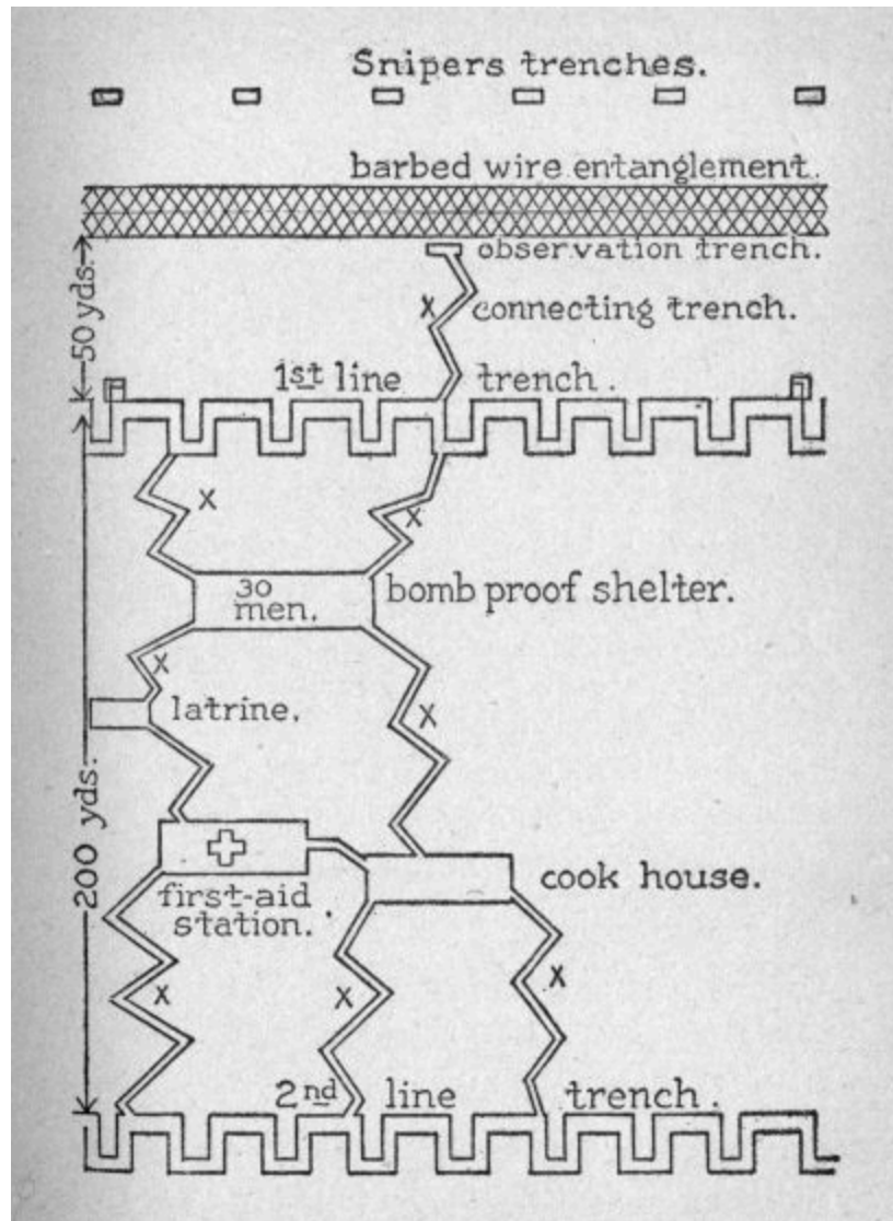
Trench layout diagram
