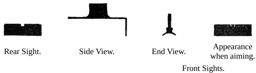
Patridge Sights. Figure 60.
