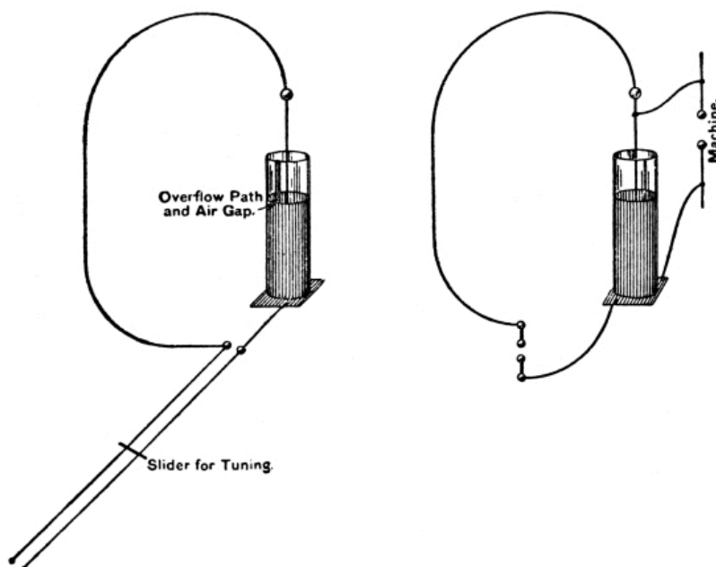
FIG. 4.—Experiment with Syntonic Leyden Jars ( cf. page 21 ).
