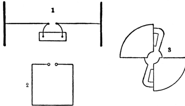
FIG. 14. — Bjerknes' Apparatus, showing (1) a Hertz vibrator connected to an induction coil; (2) a nearly closed circuit receiver properly tuned with the vibrator; and (3) a one sided electrometer for inserting in the air gap of 2. The receiver is not provided with knobs, as shown, but its open circuit is terminated by the quadrants of the electrometer, which is shown on an enlarged scale alongside. The needle is at zero potential and is attracted by both quadrants. By calculation from the indications of this electrometer Bjerknes plotted the curves 1, 2 and 3 on pages 4 and 5 . Fig. 1 represents the oscillations of the primary vibrator, rapidly damped by radiation of energy. Fig. 2 represents the vibrations thereby set up in the resonating circuit when the two are accurately in tune; and which persist for many swings. Fig. 3 shows the vibrations excited in the same circuit when slightly out of tune with the exciter. A receiver of this kind makes many swings before it is seriously damped, though the open plate radiator does not.
