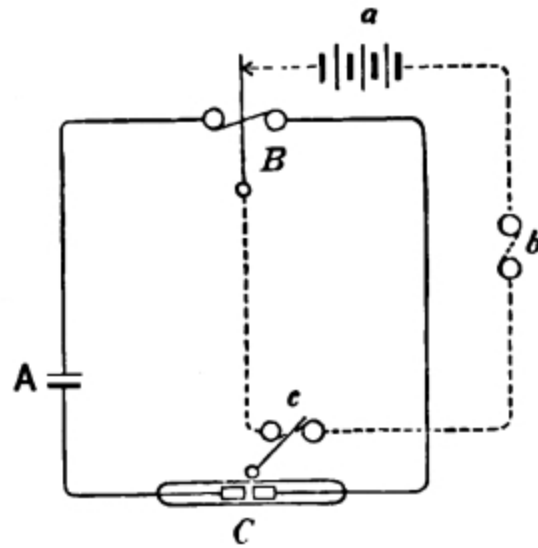
FIG. 44 (Fig. 8 of Slaby's book).—
