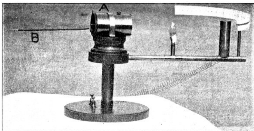
FIG. 19B. — A Portable Detector, B the Collecting Wire.
