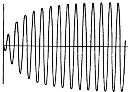
FIG. 2.—Oscillation of Ring-shaped Hertz Resonator excited by Syntonic Vibrator (after Bjerknes).
