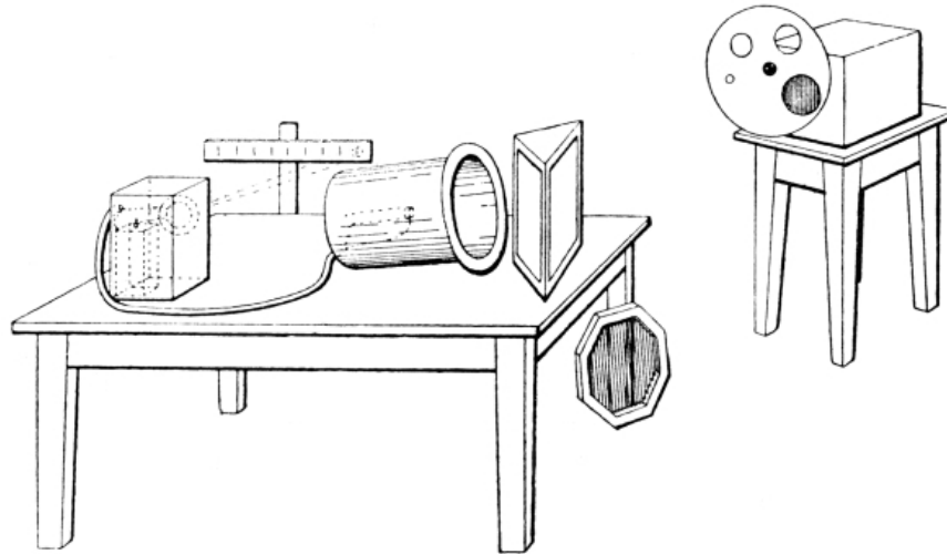
FIG. 21. — General arrangement of experiments with the Copper “Hat,” showing Metal Box on a Stool, standing outside the Theatre. The Box is not exactly represented, but inside it the Radiators were fixed with a graduated series of apertures; the Copper Hat containing the Coherer is seen on the Table with the Metal Box on the left of the Table containing Battery and Galvanometer Coil connected to it by a compo pipe conveying the wires, as in Fig. 19c ; the Lamp and Scale barely indicated at one side of the Table; a Paraffin Prism; and a Polarising Grid of copper wires stretched on a frame. (This figure is from a thumbnail sketch by Mr. A. P. Trotter, taken at the Lecture in 1894.)
