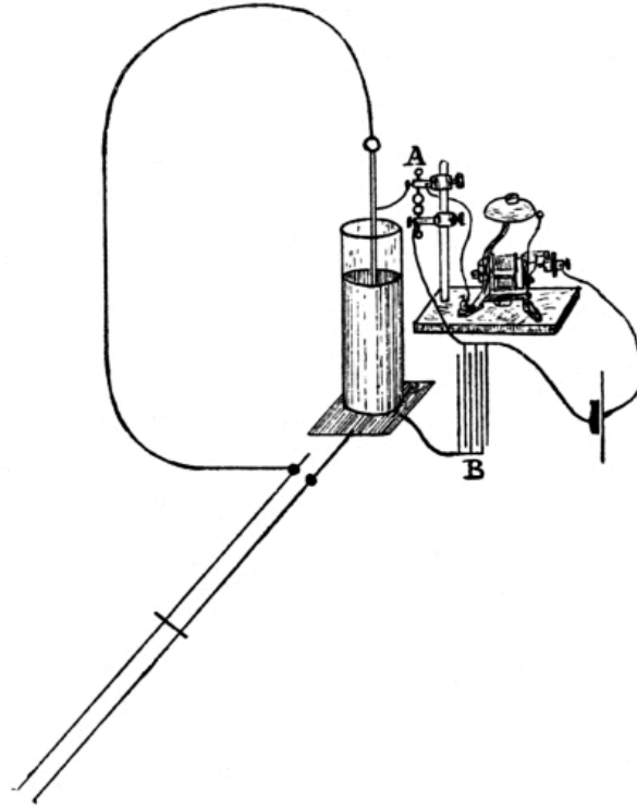
FIG. 16A. — Receiver in Syntonic Jar Experiment, with Knob Coherer and Tapper-back ( cf. Fig. 4 ).
