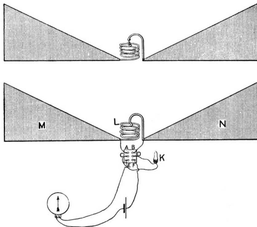
Syntonic Sender and Receiver used in the experiments plotted on page 28 . The switch enables the coherer K to be connected either to the tuned resonator M L N or to the detecting circuit E F. Weak impulses are felt when the switch is C E, D F; strong impulses when the switch is C A, D B; provided the coil L is similar to the coil of the radiator above. The impulses are plotted in the diagram Fig. 19A.
