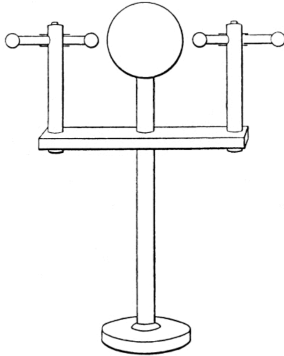
FIG. 19. — Radiator used in the library of the Royal Institution, exciting the Coherer ( Fig. 17 ) on the lecture table in the Theatre. I also used a radiator with two or with three large spheres between two knobs, and described it in Nature , Vol. 41, p. 462, 1890. This is the radiator which Prof. Righi has improved and made in a compact form with oil between the two middle spheres.
