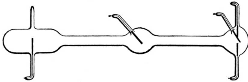
FIG. 13. — Zehnder's Trigger Tube. Half Natural Size. The two right-hand terminals, close together, are attached to the Hertz receiver; another pair of terminals are connected to some source just not able to make the tube glow until the scintilla occurs and makes the gas more conducting—as observed by Schuster and others.
