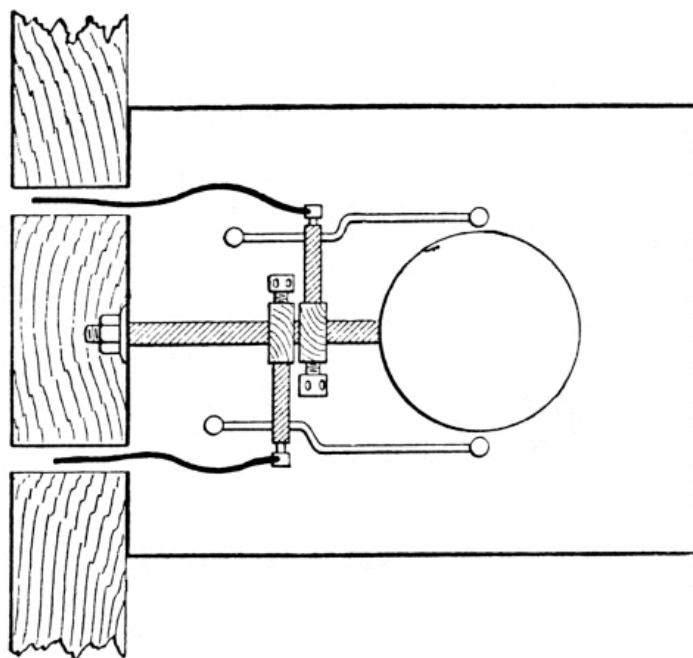
FIG. 20. — Spherical Radiator for emitting a Horizontal Beam, arranged inside a Copper Hat, fixed against the outside of a metal-lined Box, which contains induction coil and battery and key. One-eighth natural size. The wires pass into the box through glass tubes not shown.
