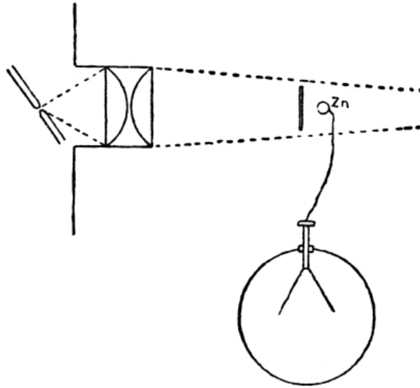
FIG. 8. — Zinc Rod in Arc Light, protected by Glass Screen. The lenses are of quartz, but there is no need for any lenses in this experiment; leakage of electricity begins directly the glass plate is withdrawn.
