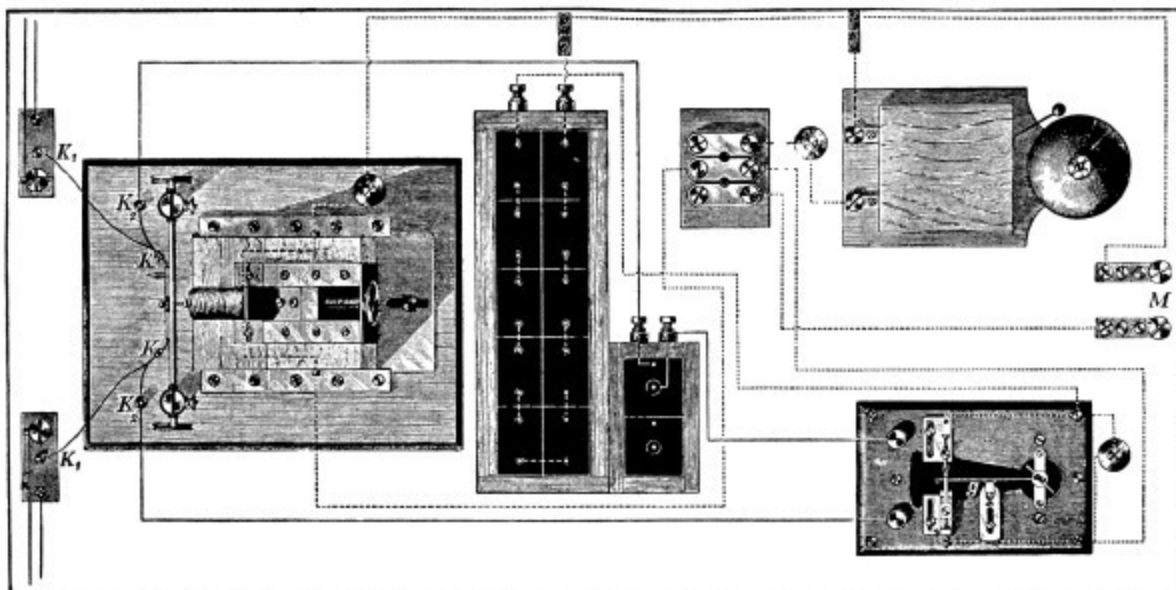
FIG. 45 (Fig. 16 of Slaby's book).—
