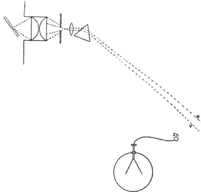
FIG. 9. — Zinc Rod discharging Negative Electricity in the very Ultra-violet Light of a Spectrum formed by a Quartz Train. The best discharging light is found far beyond the limits of the visible spectrum.
