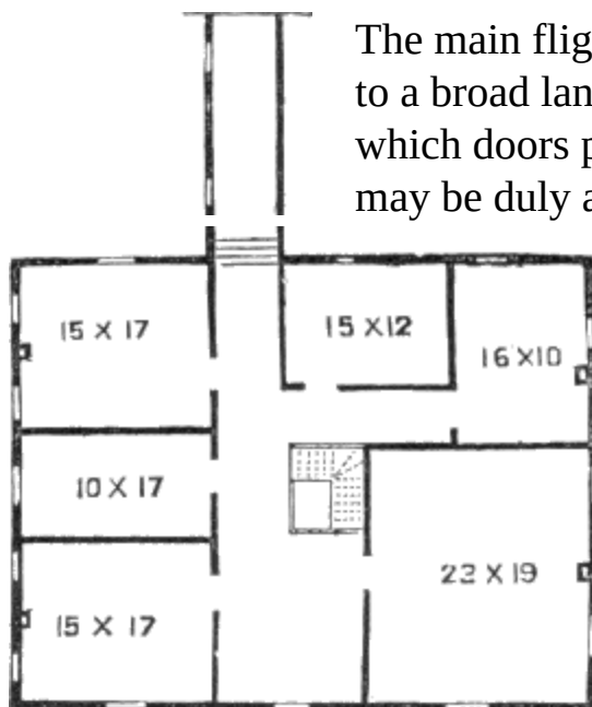
CHAMBER PLAN.
