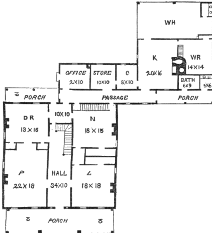
GROUND PLAN
