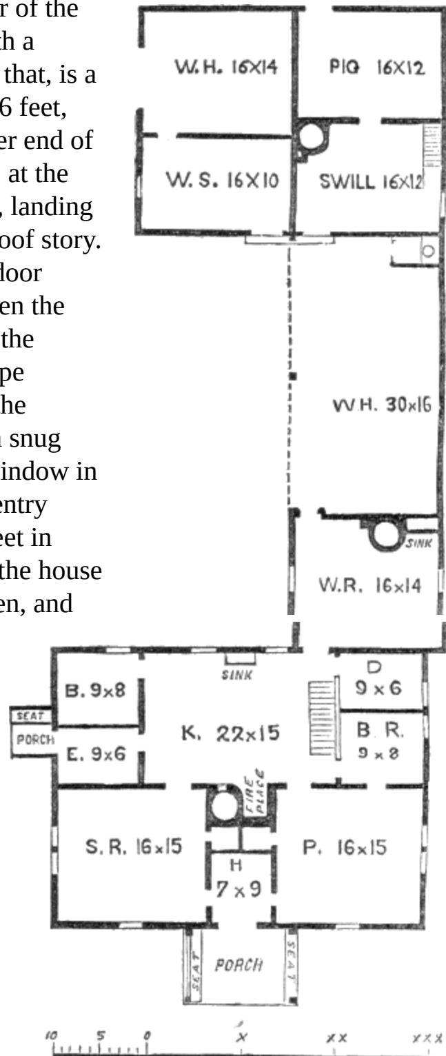
GROUND PLAN.
