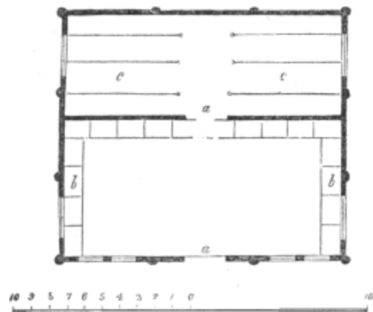
GROUND PLAN.
