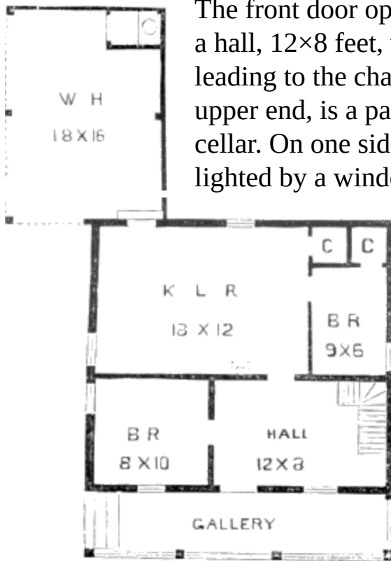
PLAN
