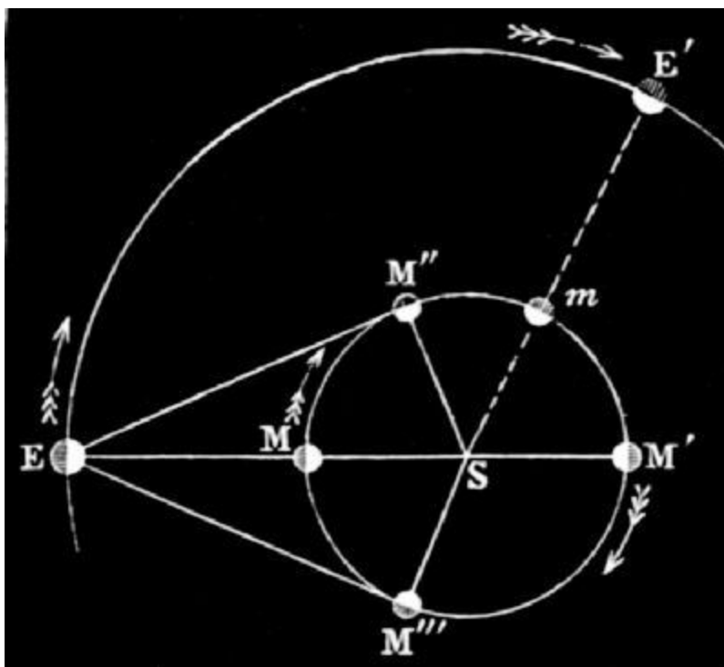
FIG. 13.—Orbit of Mercury and Earth.
