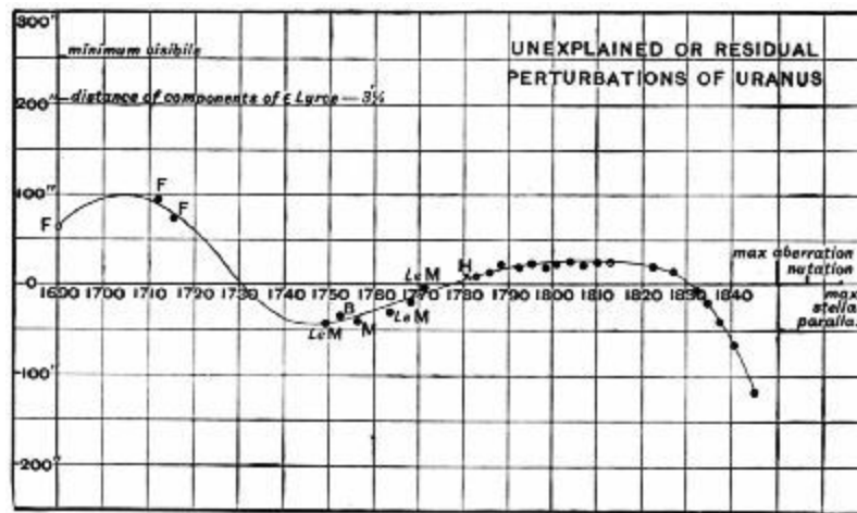
FIG. 93.—Perturbations of Uranus.
