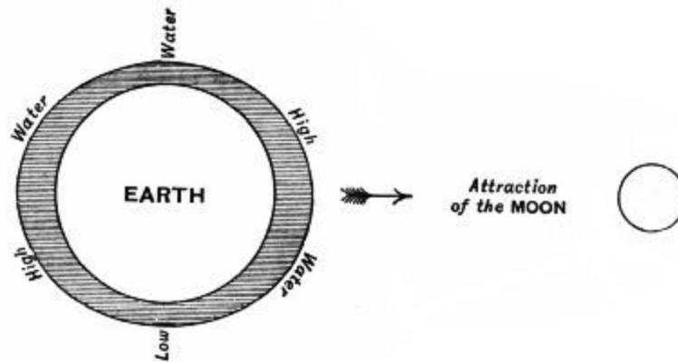
FIG. 112.—Earth and moon (earth's rotation neglected).
