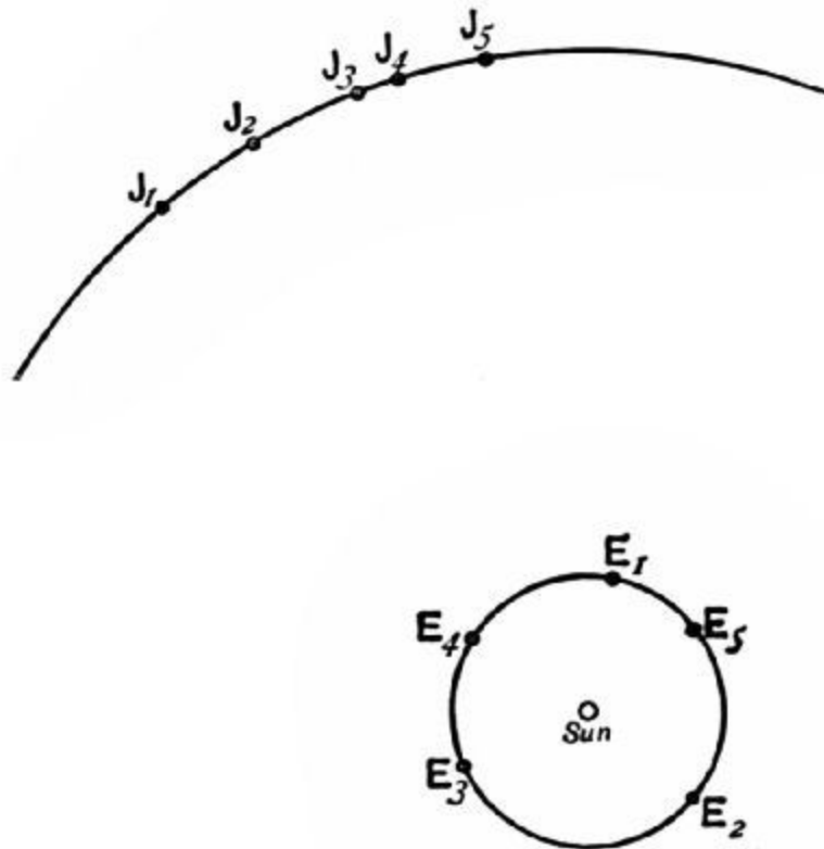
FIG. 12.—True orbits of Earth and Jupiter.
