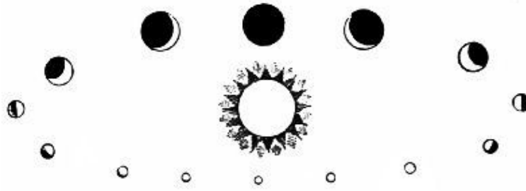
FIG. 47.—Phases of Venus. Showing also its apparent variations in size by reason of its varying distance from the earth. When fully illuminated it is necessarily most distant. It looks brightest to us when a broad crescent.
