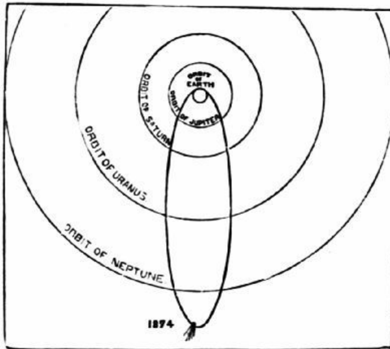
FIG. 99.—Orbit of Halley's comet.
