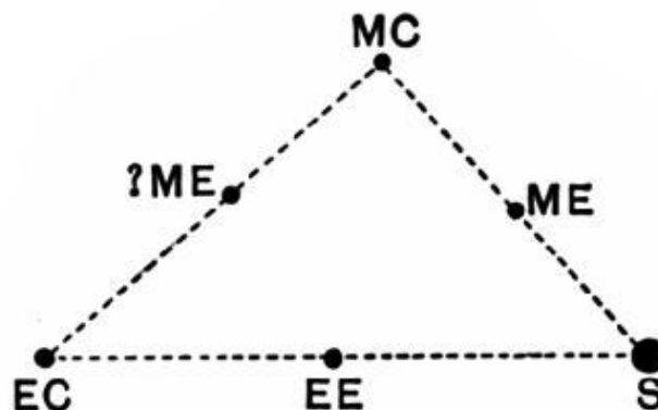
FIG. 29.—S represents the sun; EC, the centre of the earth's orbit, to be placed as best suited; MC, the same for Mars; EE, the earth's equant, or point about which the earth uniformly revolved ( i.e. the point determining the law of speed about the sun), likewise to be placed anywhere, but supposed to be in the line joining S to EC; ME, the same thing for Mars; with ?ME for an alternative hypothesis that perhaps Mars' equant was on line joining EC with MC.
