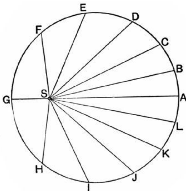
FIG. 30.—Excentric circle supposed to be divided into equal areas. The sun, S, being placed at a selected point, it was possible to represent the varying speed
