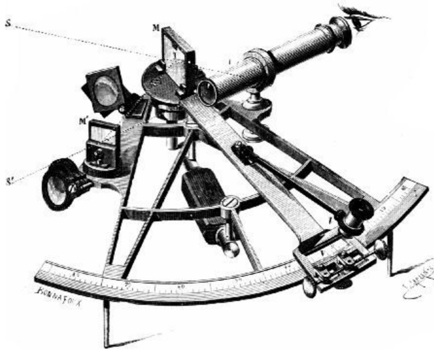
FIG. 67.—The sextant, as now made.
