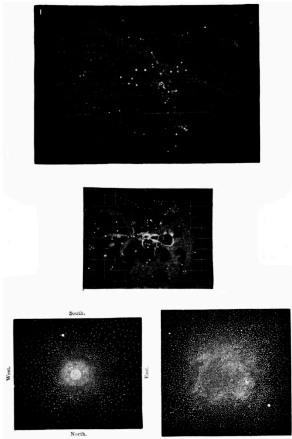
FIG. 43.—Some clusters and nebulae.
