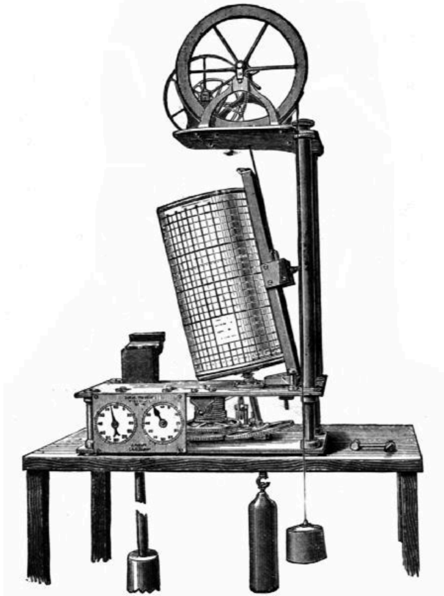
FIG. 117.—Tide-gauge for recording local tides, a pencil moved up and down by a float writes on a drum driven by clockwork.
