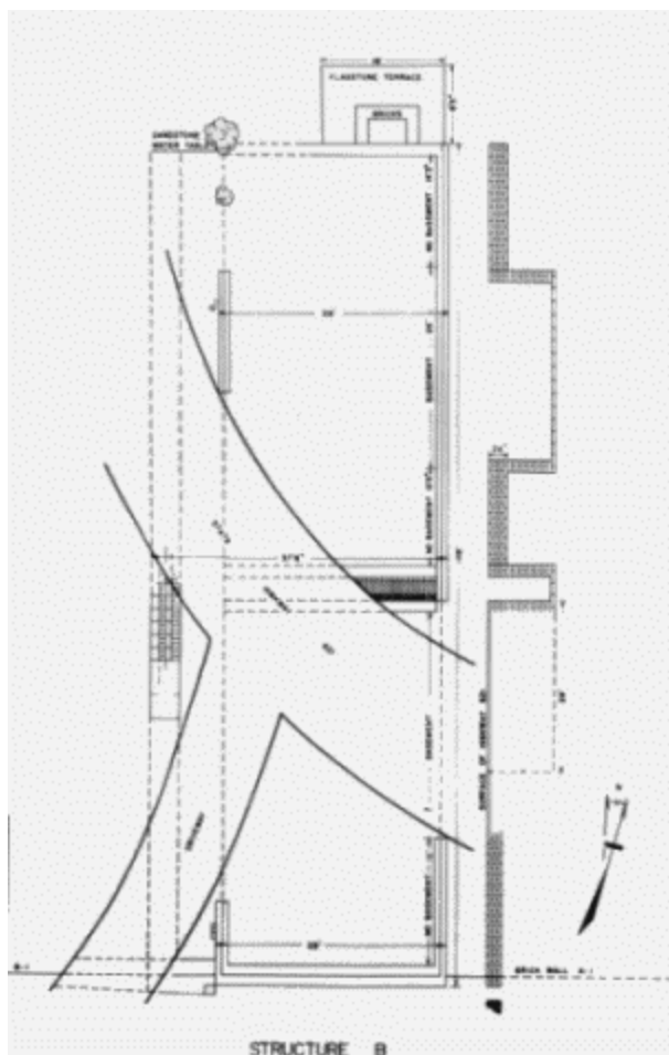
Figure 32.—EXCAVATION PLAN of Structure B.
