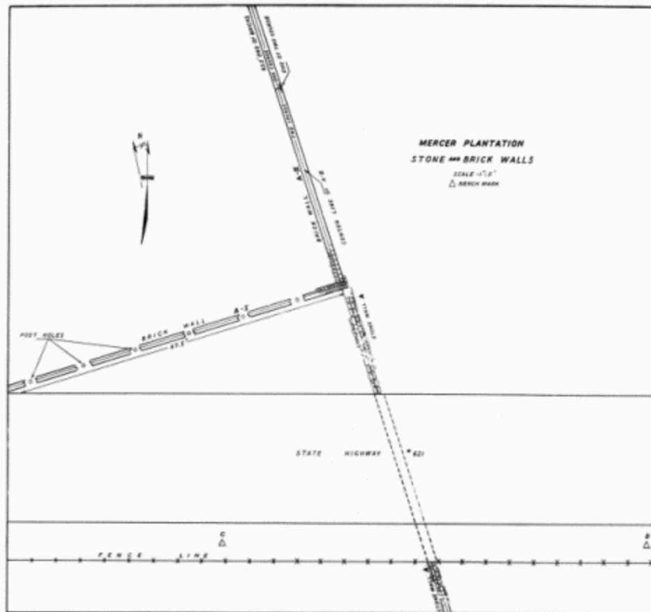
Figure 21.—EXCAVATION PLAN of wall system.
