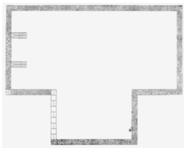
Figure 60.—EXCAVATION PLAN of Stafford courthouse foundation.
