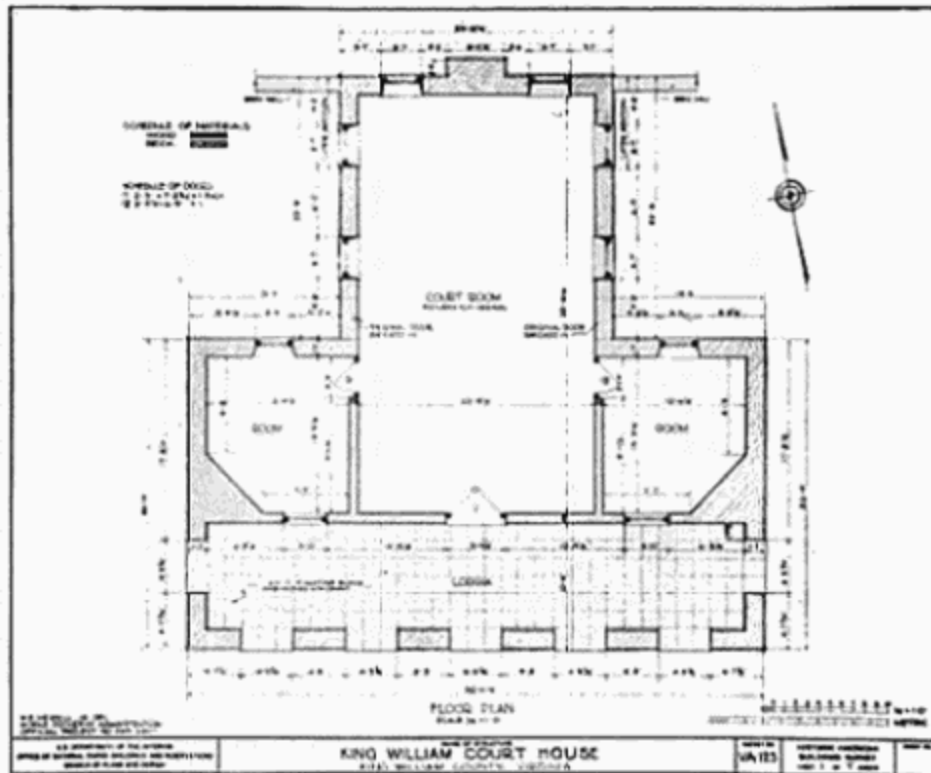
Figure 62.—PLAN OF KING WILLIAM COURTHOUSE, whose plan dimensions correspond closely to the Stafford foundation. (Courtesy of Historic American Buildings Survey, Library of Congress.)
