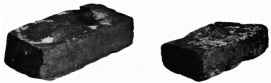
Figure 53.—VIRGINIA BRICK from Structure B (left) 9 by 4 by 2¾ inches. Right, small brick from Structure F, probably imported, 7¼ by 3½ by 1¾ inches. Perhaps one of the 630 bricks brought on the Marigold by Captain Roger Lyndon and purchased by John Mercer.
