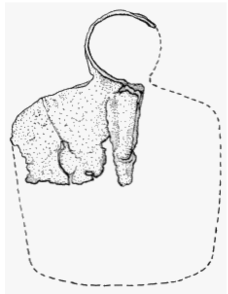
Illustration 83.—Hilling hoe. One-fourth. (USNM 59.1848.)
