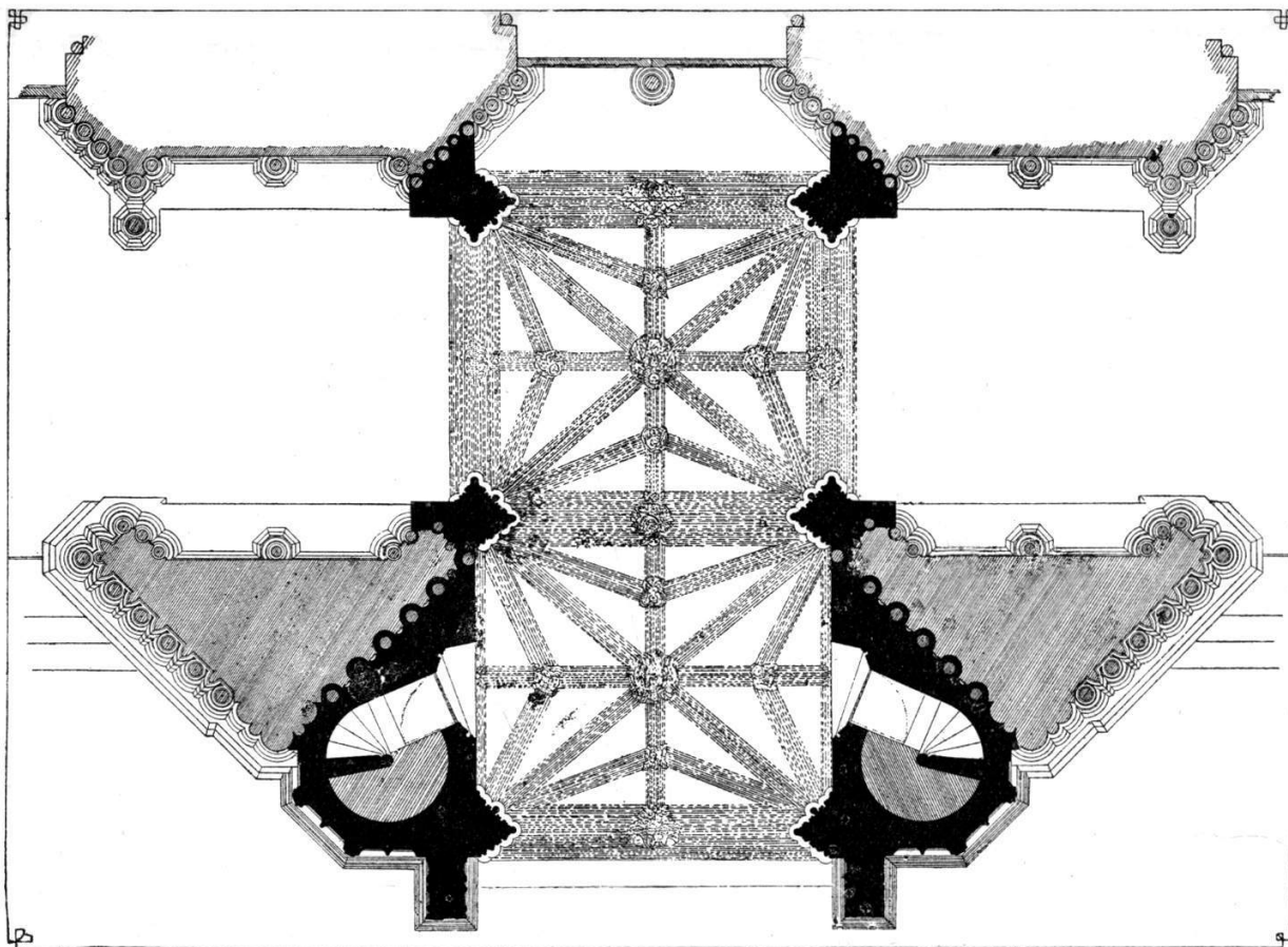
PLAN OF CENTRAL PORTION OF WEST FRONT, WITH GROINING OF PORCH. BY W. H. LORD.
