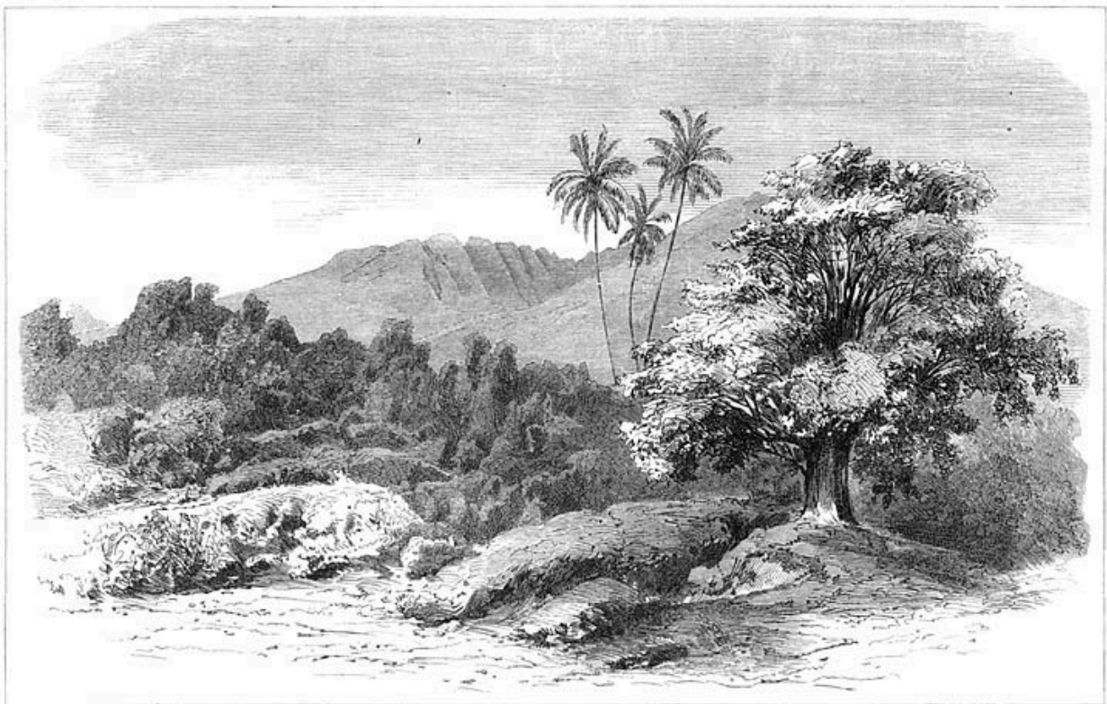
Vulkan Ysarog in WSW
