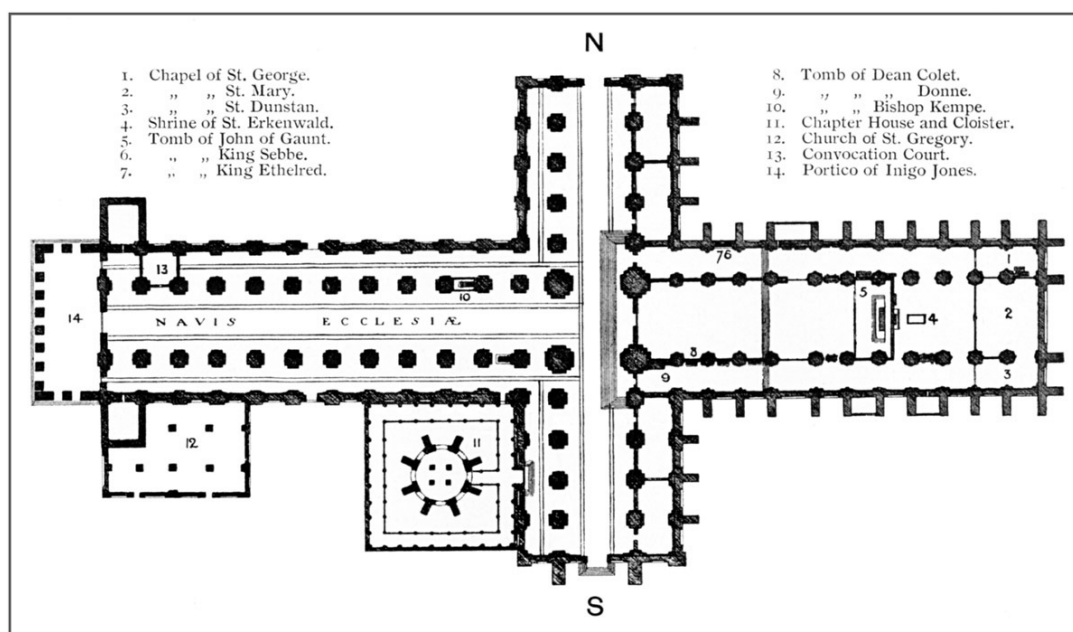
PLAN OF OLD ST. PAUL'S IN 1666. ToList
