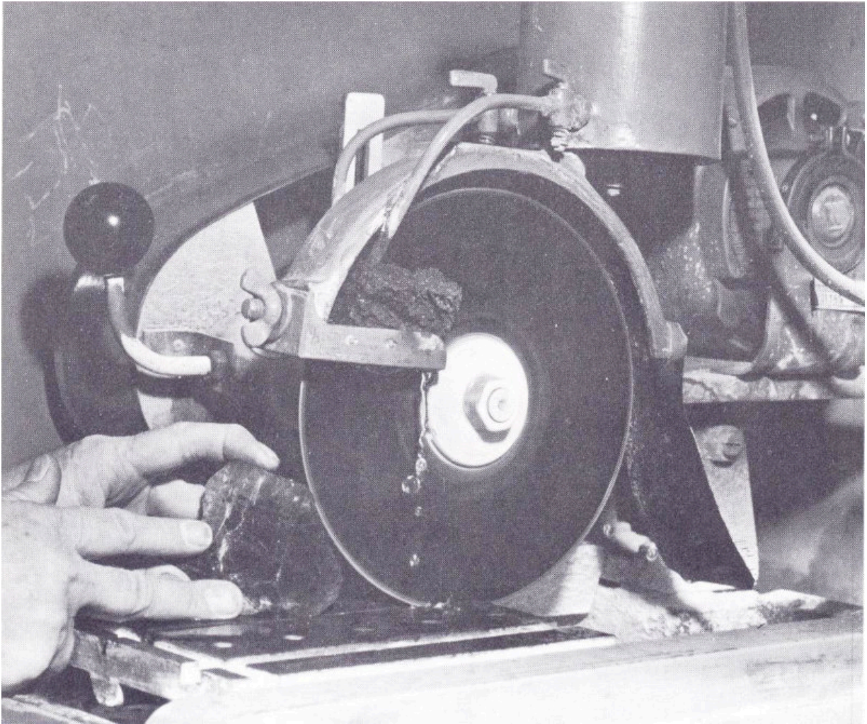
With this typical trim saw, water is used as a coolant for the rapidly rotating metal disk, which has a diamond-impregnated rim. Here, the blade is cutting its way through a piece of gem tourmaline.
