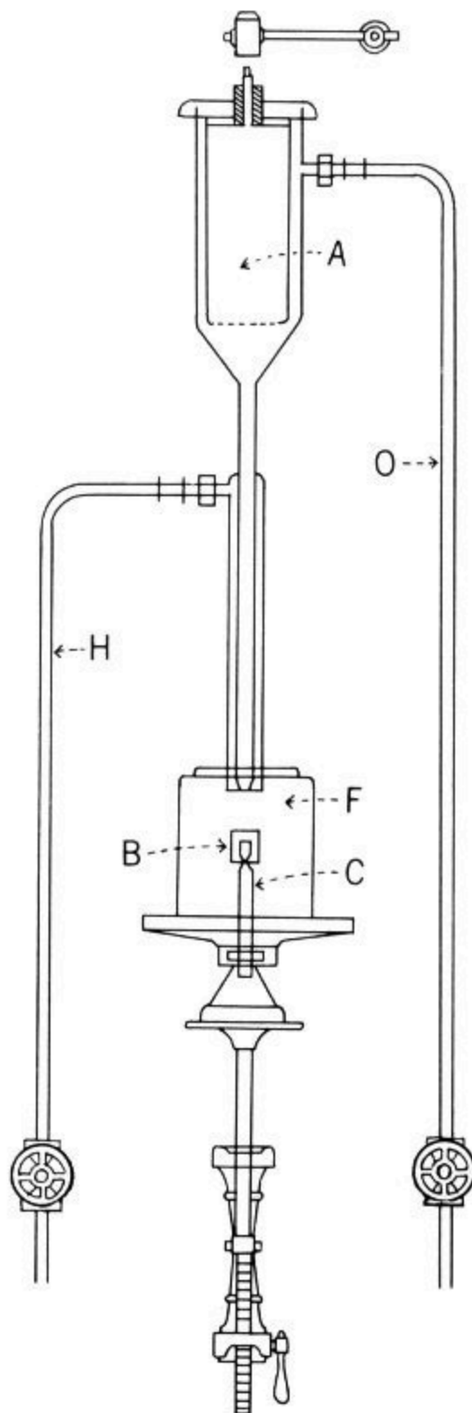
The Verneuil furnace, for making synthetic gem rough. A mixture of hydrogen (H) and oxygen (O) burns almost explosively, heating the fusion chamber (F) to high temperatures. For example, powdered aluminum oxide and coloring agents are sifted
